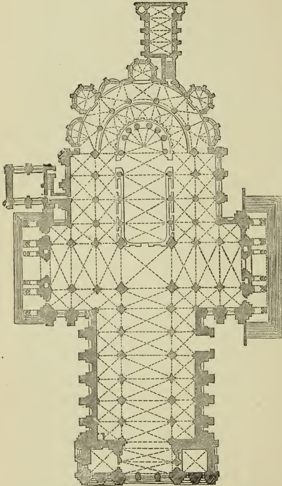
389. Plan of Chartres Cathedral. (From Chapuy.) Scale 100 ft. to 1 in.
