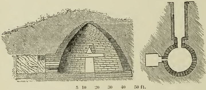
122. Section and Plan of Tomb of Atreus at Mycenæ. Scale of plan 100 ft. to 1 in.
