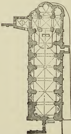
350. St. Trinité, Angers. (From Faultrier.) Scale 100 ft. to 1 in.
