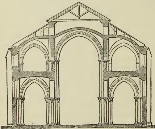
370. Section of Narthex at Vezelay. (From Didron's "Annales Archéologiques.")
