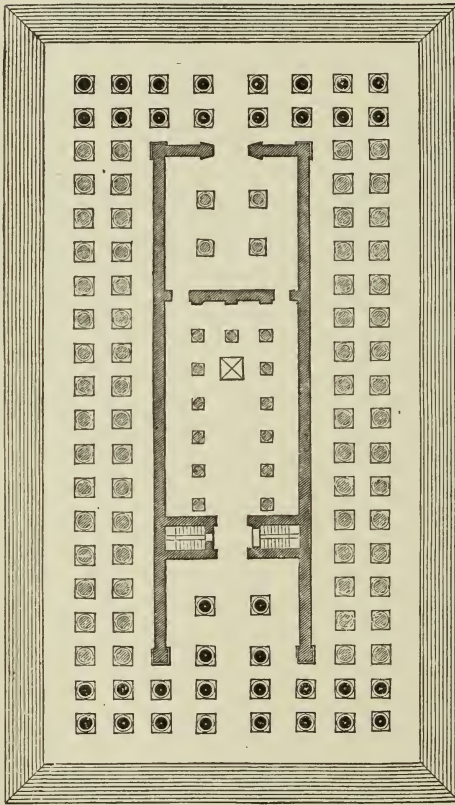
159. Plan of the Temple of Diana at Ephesus, embodying Mr. T. Wood's discoveries. Scale 100 ft. to 1 in.
