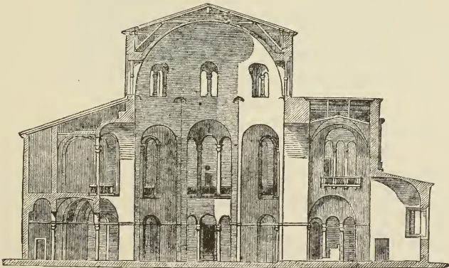
302. Section of St. Vitale, Ravenna. (From Isabelle.) Scale 50 ft. to 1 in.
