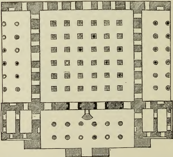
90. Restored Plan of Great Hall of Xerxes at Persepolis. Scale 100 ft. to 1 in.
