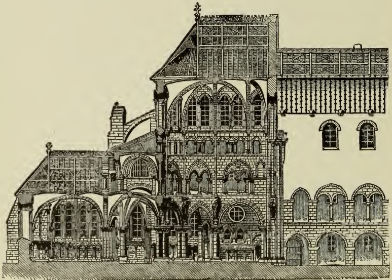
376. Section of Eastern Portion of Church of Mortier en Der. (From the "Archives des Monuments," etc.)
