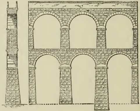
250. Aqueduct of Tarragona. Scale 50 ft. to 1 in.
