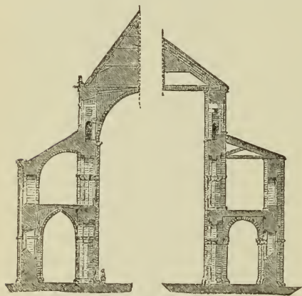
380. Fig. 1, after Vaulting; Fig. 2, before Vaulting. Section of Nave of St. Stephen, Caen.
