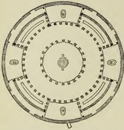
296. Plan of San Stephano Rotondo. (From Gutensohn and Knapp.) Scale 100 ft. to 1 in.
