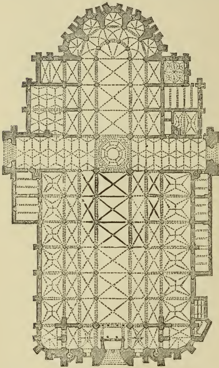
445. Plan of the Cathedral at Antwerp. Scale 100 feet to 1 in.
