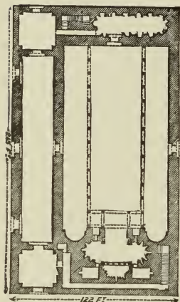
272. White Convent near Siout. (From a plan by the Hon. Sir Arthur Gordon.) Scale 100 ft. to 1 in.
