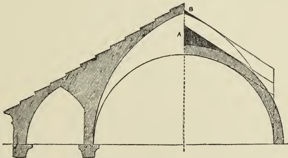
310. Diagram of Vaulting. South of France.
