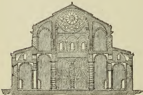
339. Section of the Church of St. Sernin, Toulouse. Scale 50 ft. to 1 in.
