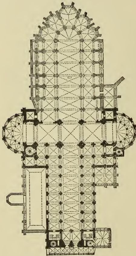
440. Plan of Cathedral at Tournay. Scale 100 ft. to 1 in.
