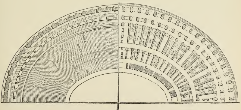
211. Quarter-plan of the Seats, and quarter-plan of the Basement of the Flavian Amphitheatre. No scale.
