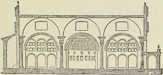
201. Longitudinal Section of Basilica of Maxentius. Scale 100 ft. to 1 in.
