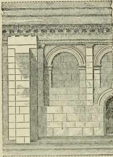
317. Elevation of half one Bay of the Exterior of St. Paul au Trois Chateaux.
