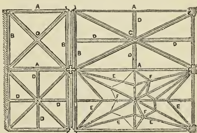
426. Diagram of Vaulting.
