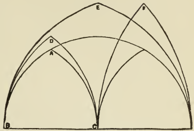
381. Diagram of Vaulting.
