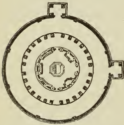
297. Plan of Sti. Angeli, Perugia. (From Isabelle.) Scale 100 ft. to 1 in.
