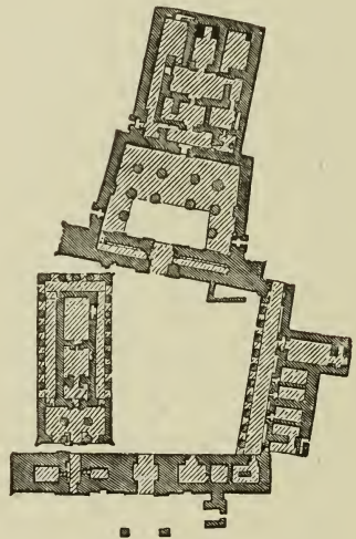
43. Plan of Temple at Philæ. Scale 100 ft. to 1 in.
