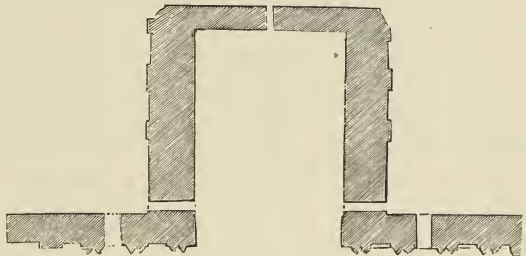
260. Plan of Tâk Kesra at Ctesiphon. (From Flandin and Coste.) Scale 100 ft. to 1 in.
