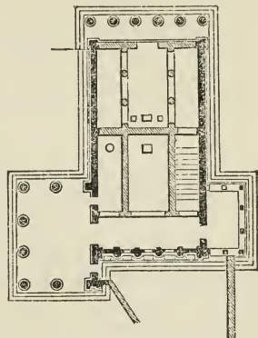
158. Restored Plan of Erechtheium. Scale 50 ft. to 1 in.
