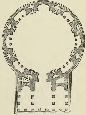
190. Plan of Pantheon at Rome. Scale 100 ft. to 1 in.
