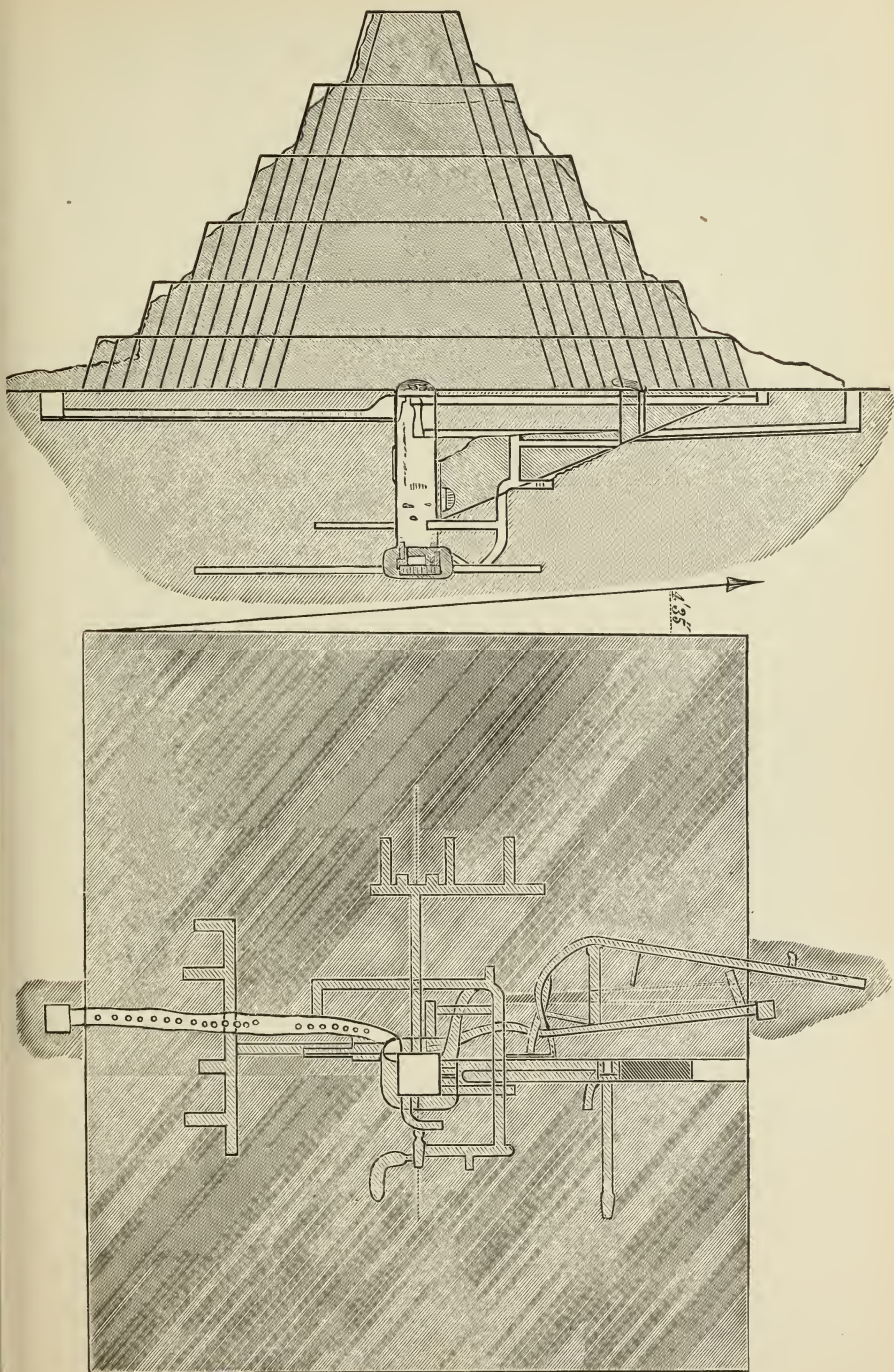
No. 9. Pyramid of Saccara. (From Colonel Vyse's work.) Scale 100 ft. to 1 in.
