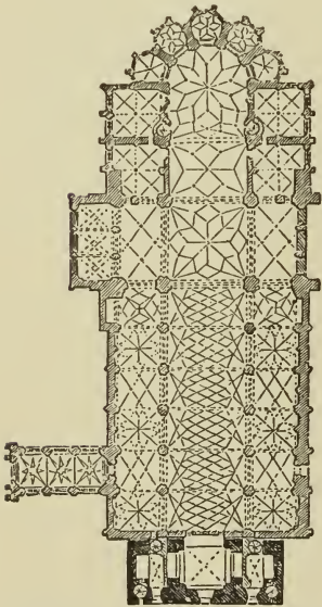
446. Plan of St. Jacques, Liège. (From Weale's "Architectural Papers.") Scale 100 ft. to 1 in.
