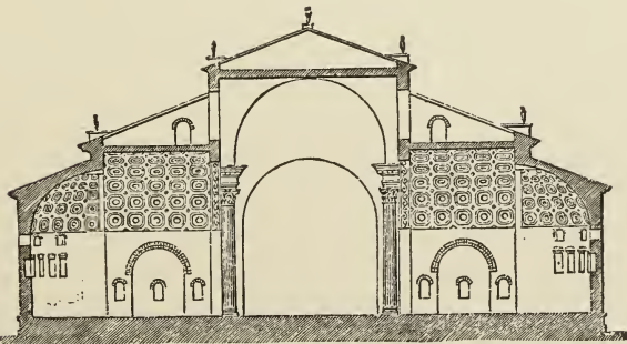
202. Transverse Section of Basilica of Maxentius. Scale 100 ft. to 1 in.
