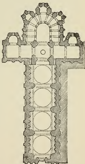
352. Plan of Church at Fontevault. (From Verneilh.) Scale 100 ft. to 1 in.
