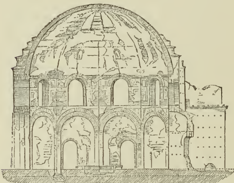
228. Section of Minerva Medica. (From Isabelle.) Scale 50 ft. to 1 in.
