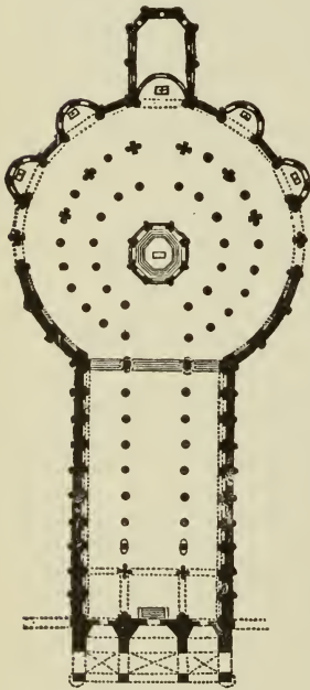
342. Church of Charroux Scale 100 ft. to 1 in.
