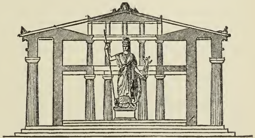
150. Section of the Parthenon. Scale 50 ft. to 1 in.
