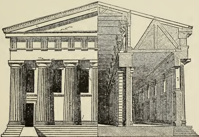
151. Part Section, part Elevation, of Great Temple at Agrigentum. Scale 50 ft. to 1 in.
