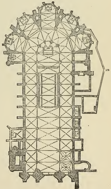
405. Plan of Cathedral at Bazas. (From Lamothe. 1 ) Scale 100 ft to 1 in.
