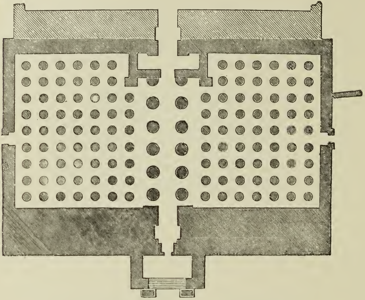
22. Plan of Hypostyle Hall at Karnac. Scale 100 ft. to 1 in.
