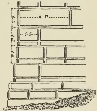
96. Elevation of Platform at Passargadæ.
