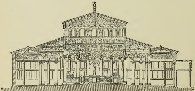
298. Section of Sti. Angeli, Perugia. (From Isabelle, "Edifices Circulaires.") No scale.
