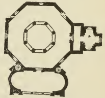
294. Baptistry of Constantine. (From Isabelle.) Scale 100 ft. to 1 in.
