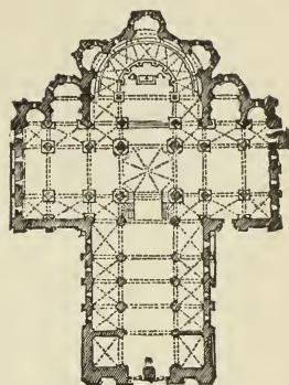
340. Plan of Church at Conques. (From Taylor and Nodier.) Scale 100 ft. to 1 in.
