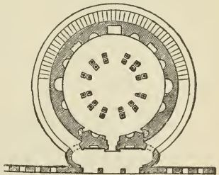
295. Plan of the Tomb of Sta. Costanza, at Rome. (From Isabelle, "Edifices Circulaires.") Scale 100 ft. to 1 in.
