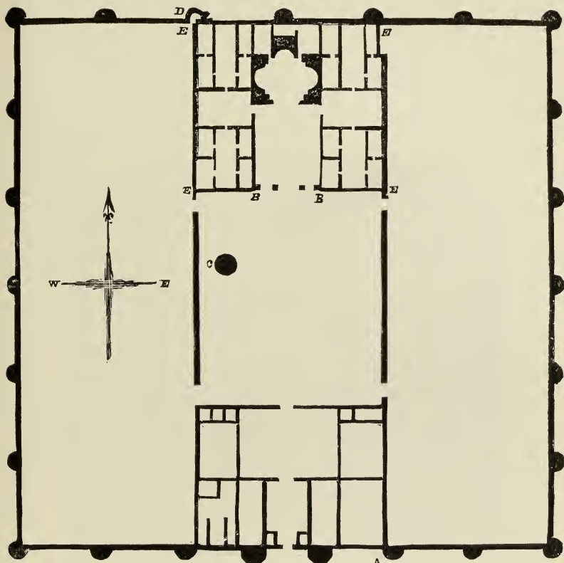
262. Sketch Plan of Palace at Mashita.
