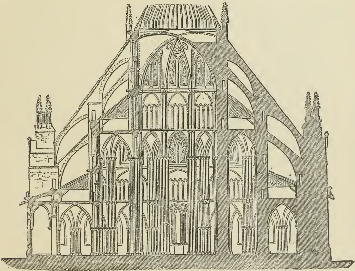
407. Section of Cathedral at Bourges. (From drawings by F. Penrose, Esq., architect.) Scale 50 ft. to 1 in.
