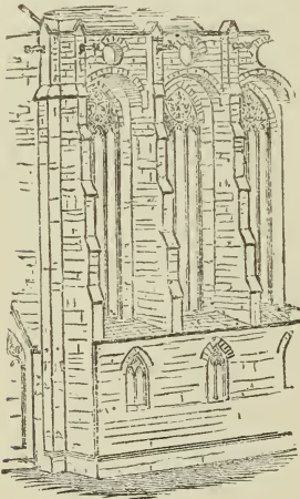
336. Section of Church of Cordeliers at Toulouse. 50 ft. to 1 in. (From King's "Study Book.")
