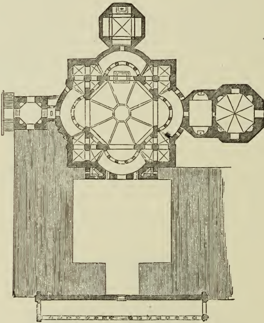
303. Plan of S. Lorenzo at Milan. (From Quast, "Altchristlichen," etc.) Scale 100 ft. to 1 in.
