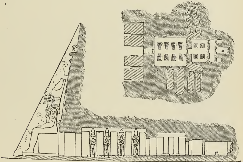
28. Plan and Section of Rock-cut Temple at Ipsamboul. Scale for plan 100 ft. to 1 in.; section 50 ft. to 1 in.
