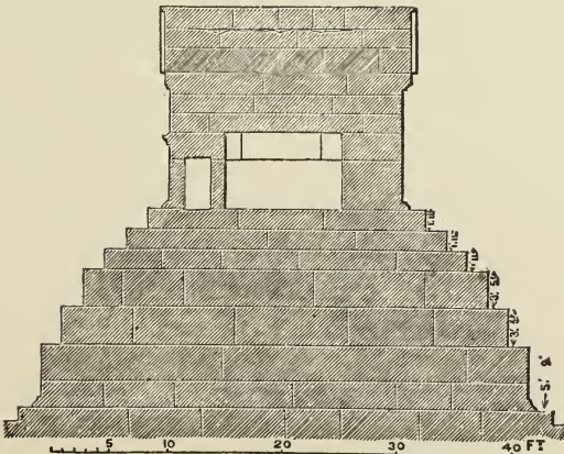
54. Section of Tomb of Cyrus. (From Texier.)
