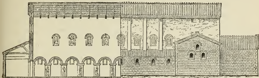
285. Half Section, half Elevation, of the Church of San Vincenzo alle Tre Fontane. (From Gutensohn and Knapp.) Scale 50 ft. to 1 in.
