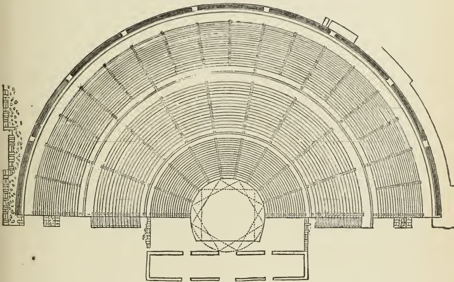
161. Plan of Theatre at Dramyssus. Scale 100 ft. to 1 in.
