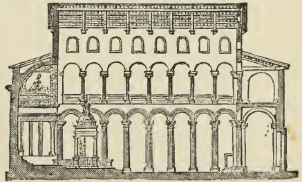
280. Section of Sta. Agnese. (From Gutensohn and Knapp.) Scale 50 ft. to 1 in.
