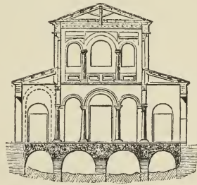
283. Section of Sta. Pudentiana. (From Hubsch. 1 ) Scale 50 ft. to 1 in.
