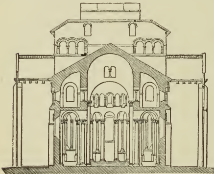
360. Section of Church at Issoire, looking East. (From Mallay.) Scale 50 ft. to 1 in.
