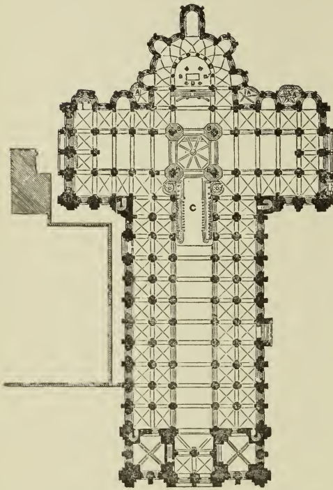
338. Church of St. Sernin, Toulouse. (From the "Archives des Monuments Historiques.") Scale 100 ft. to 1 in.
