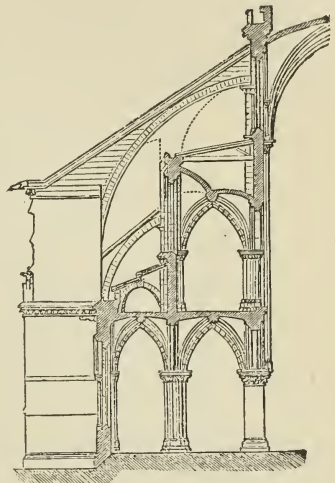
387. Section of Side Aisles, Cathedral of Paris. (From Gailhabaud, "Architecture.") Scale 50 ft. to 1 in.
