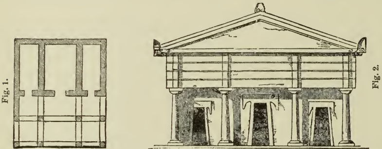
167. Plan and Elevation of an Etruscan Temple.
