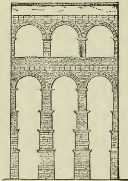
249. Aqueduct of Segovia. Scale 50 ft. to 1 in.
