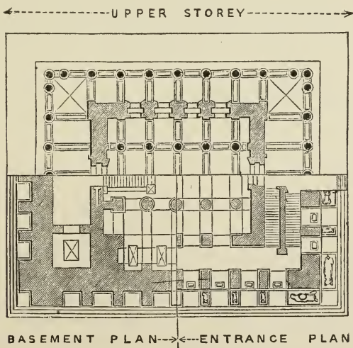
163. Plan of Mausoleum at Halicarnassus, from a Drawing by the Author. Scale 50 ft. to 1 in. VOL. I. — 18
