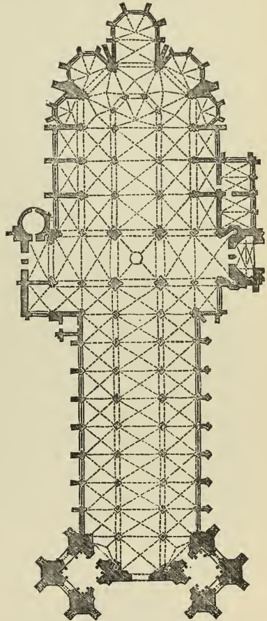
411. Plan of Church of St. Ouen at Rouen (From Peyr e's "Manuel.") Scale 100 ft. to 1 in.
