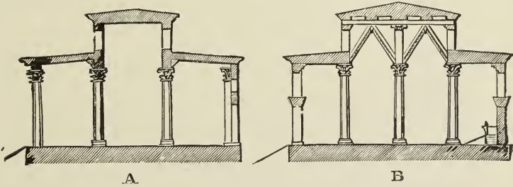
104. Diagram Sections of the House of the Cedars of Lebanon.
