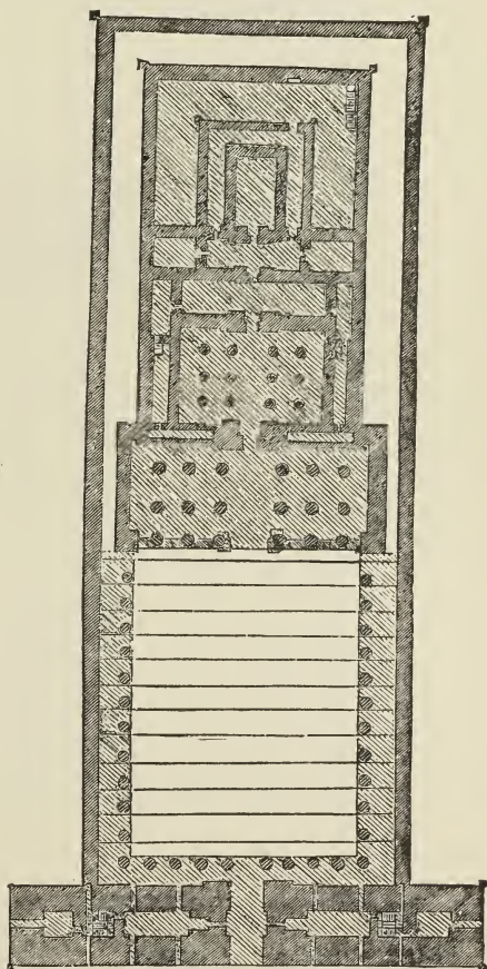
35. Plan of Temple at Edfou, Apollonopolis Magna. Scale 100 ft. to 1 in.
