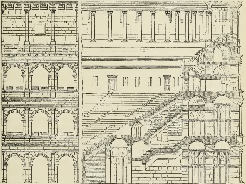
210. Elevation and Section of part of the Flavian Amphitheatre at Rome. Scale 50 ft. to 1 in.
