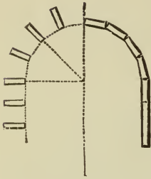
428. Diagram of Buttresses.
