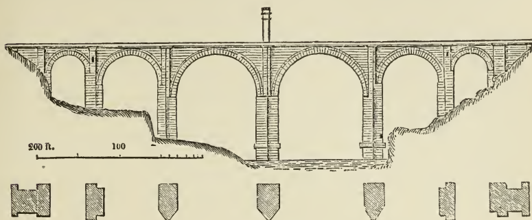
251. Bridge of Trajan, at Alcantara, in Spain.
