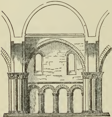
354. Elevation of one of the Bays of the Nave at Fontevraud. (From Verneilh.)
