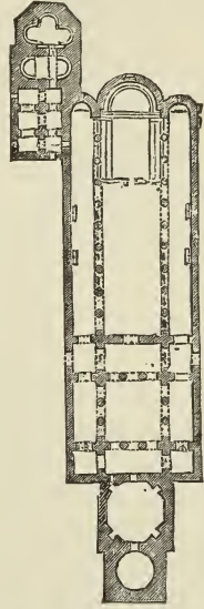
290. Church at Parenzo in Istria. (From Agincourt.) Scale 100 ft. to 1 in.
