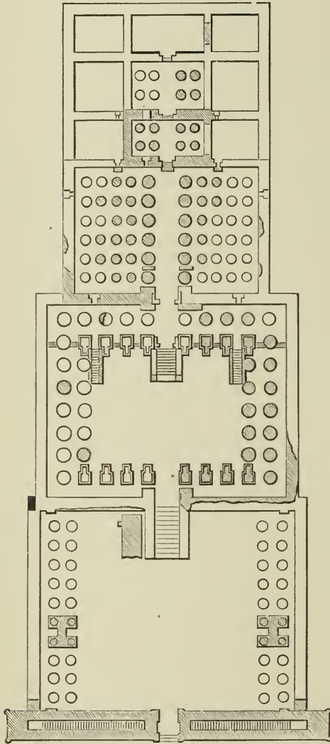
19. Rhamesion at Thebes. Scale 100 ft. to 1 in.
