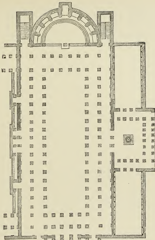
198. Plan of Trajan's Basilica at Rome. Scale 100 ft to 1 in. The part shaded darker is all that is uncovered.
