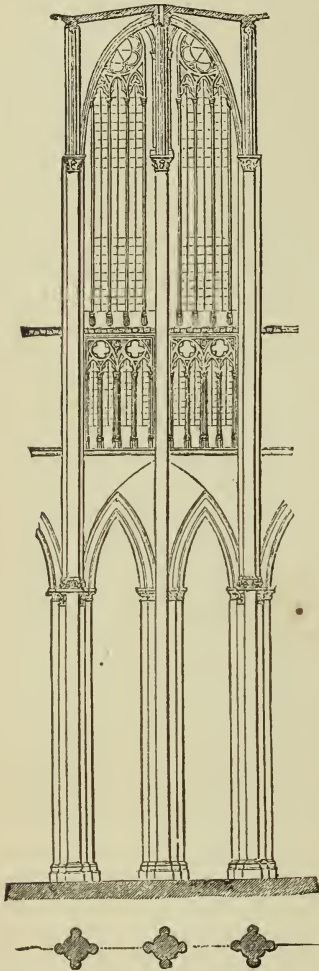
396. Bay of Nave of Beauvais Cathedral. No scale.
