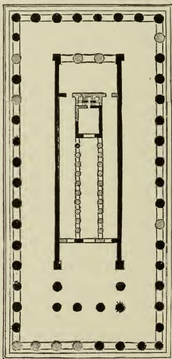
148. Plan of the great Temple at Selinus. (From Hittorf, "Arch. Antique en Sicile.") Scale 100 ft. to 1 in.
