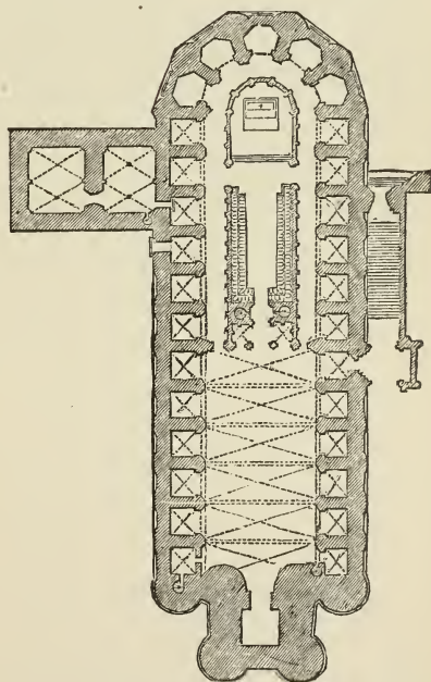
334. Plan of Cathedral at Alby. (From Chapuy, "Cathédrales Françaises.") Scale 100 ft. to 1 in.
