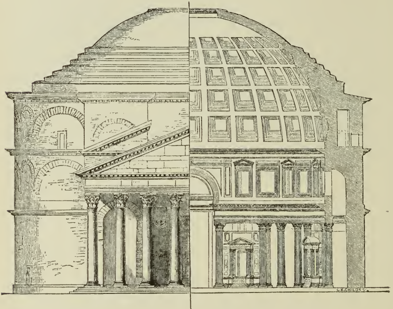
191. Half Elevation, half Section, of the Pantheon at Rome. Scale 50 ft. to 1 in.
