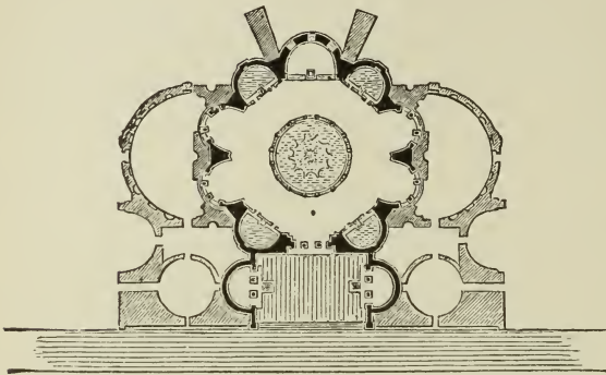
227. Plan of Minerva Medica at Rome, as restored in Isabelle's "Édifices Circulaires," on the theory of its being a Bath. Scale 100 ft. to 1 in.
