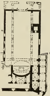
282. Plan of Sta. Pudentiana. Scale 100 ft. to 1 in.
