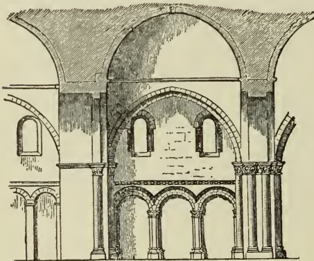
332. One Bay of Nave, Angoulême. (From Verneilh.) No scale.
