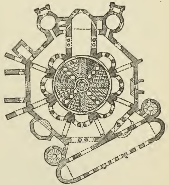
301. Plan of St. Vitale, Ravenna. (From Isabelle.) Scale 100 ft. to 1 in.
