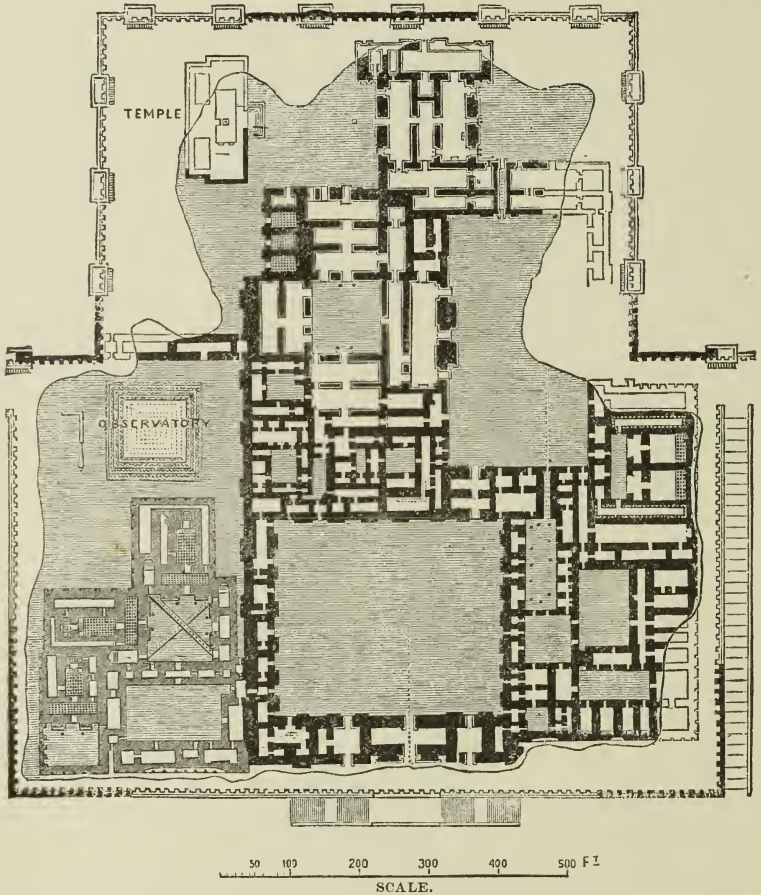
62. Plan of Palace at Khorsabad, as completely excavated by M. Place. The parts black and tinted were actually found. Those in outline are conjectural.
