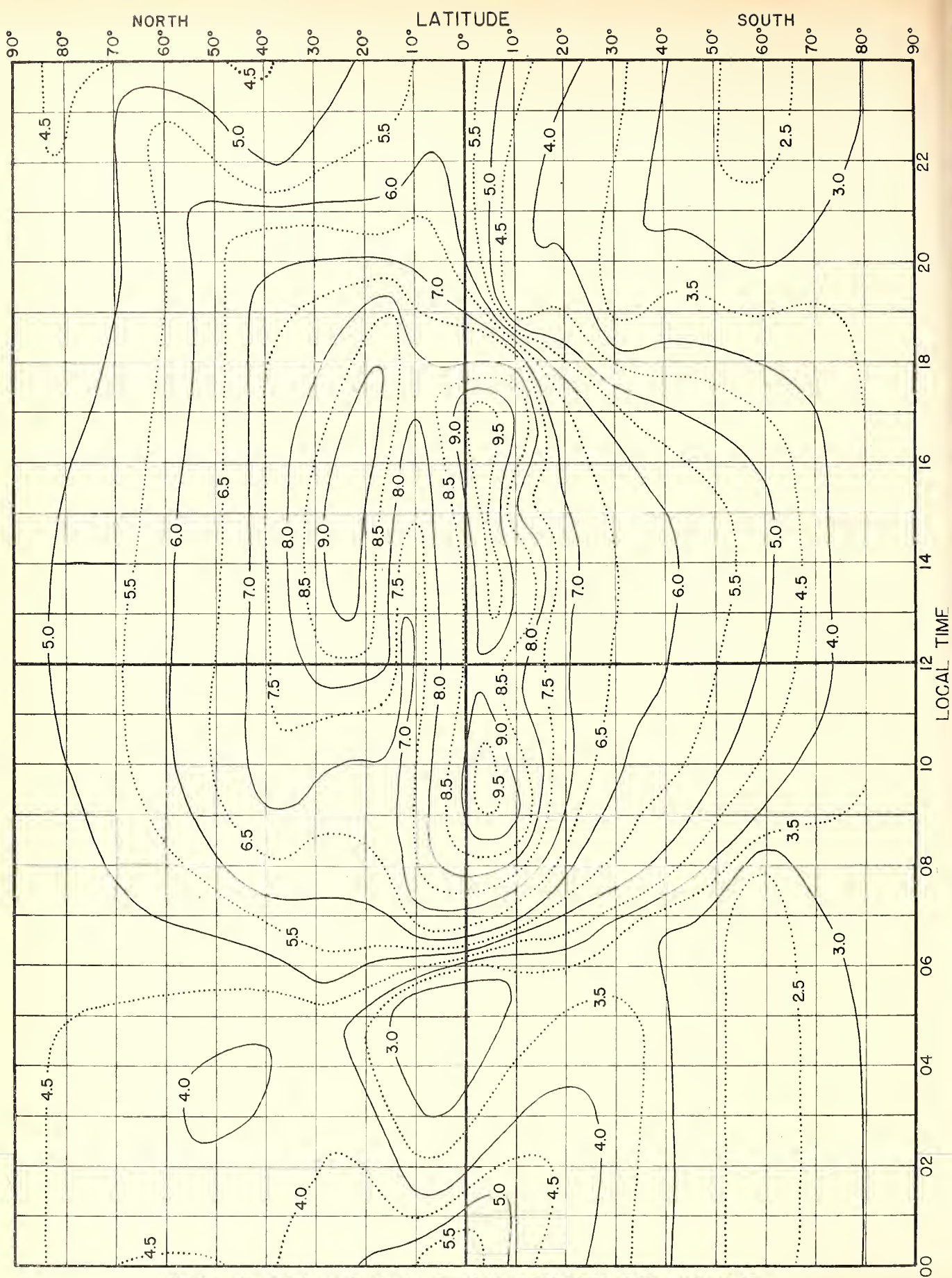
Fig. 9. F_2 ZERO-MUF, IN Mc, E ZONE, PREDICTED FOR JULY, 1945.
