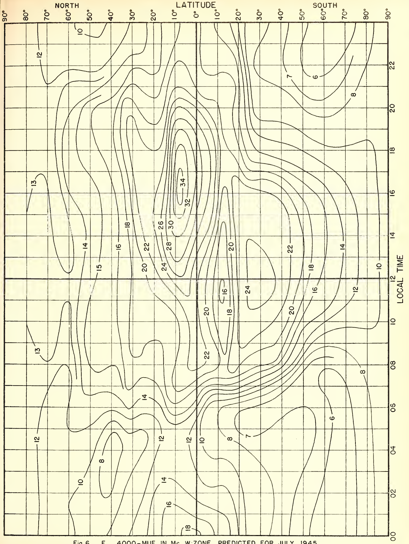
Fig. 6. F_2 4000-MUF, IN Mc, W-ZONE, PREDICTED FOR JULY, 1945.
