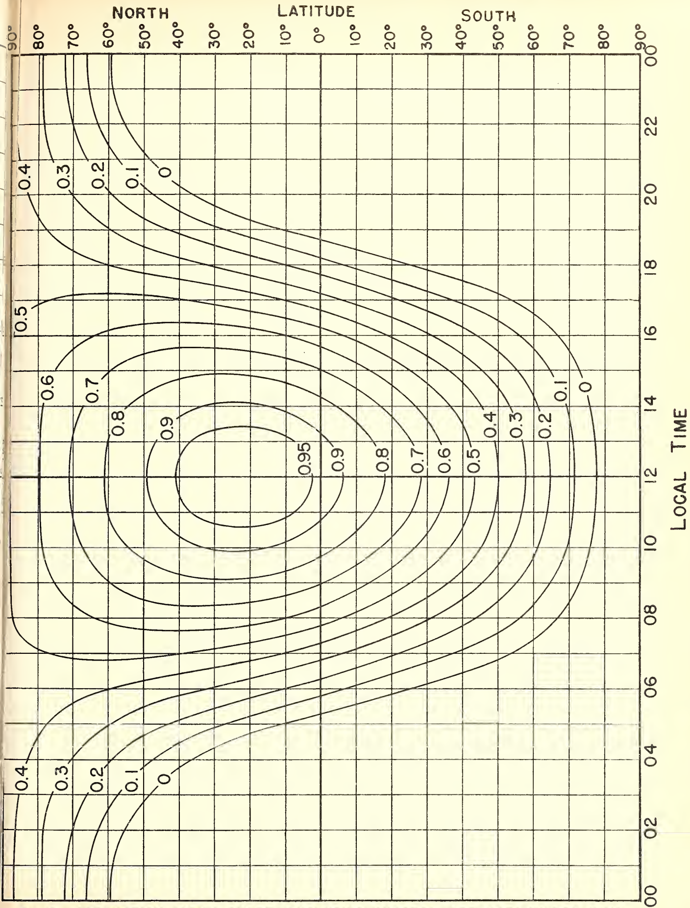
Fig.16. ABSORPTION INDEX CHART (EXCLUDING AURORAL ABSORPTION) FOR JULY.
