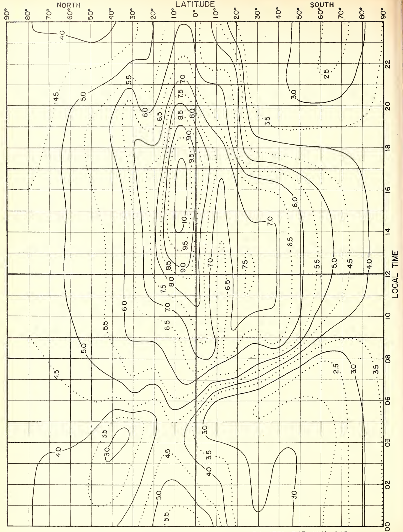
Fig 5. F_2 ZERO-MUF, IN Mc, W ZONE, PREDICTED FOR JULY, 1945.
