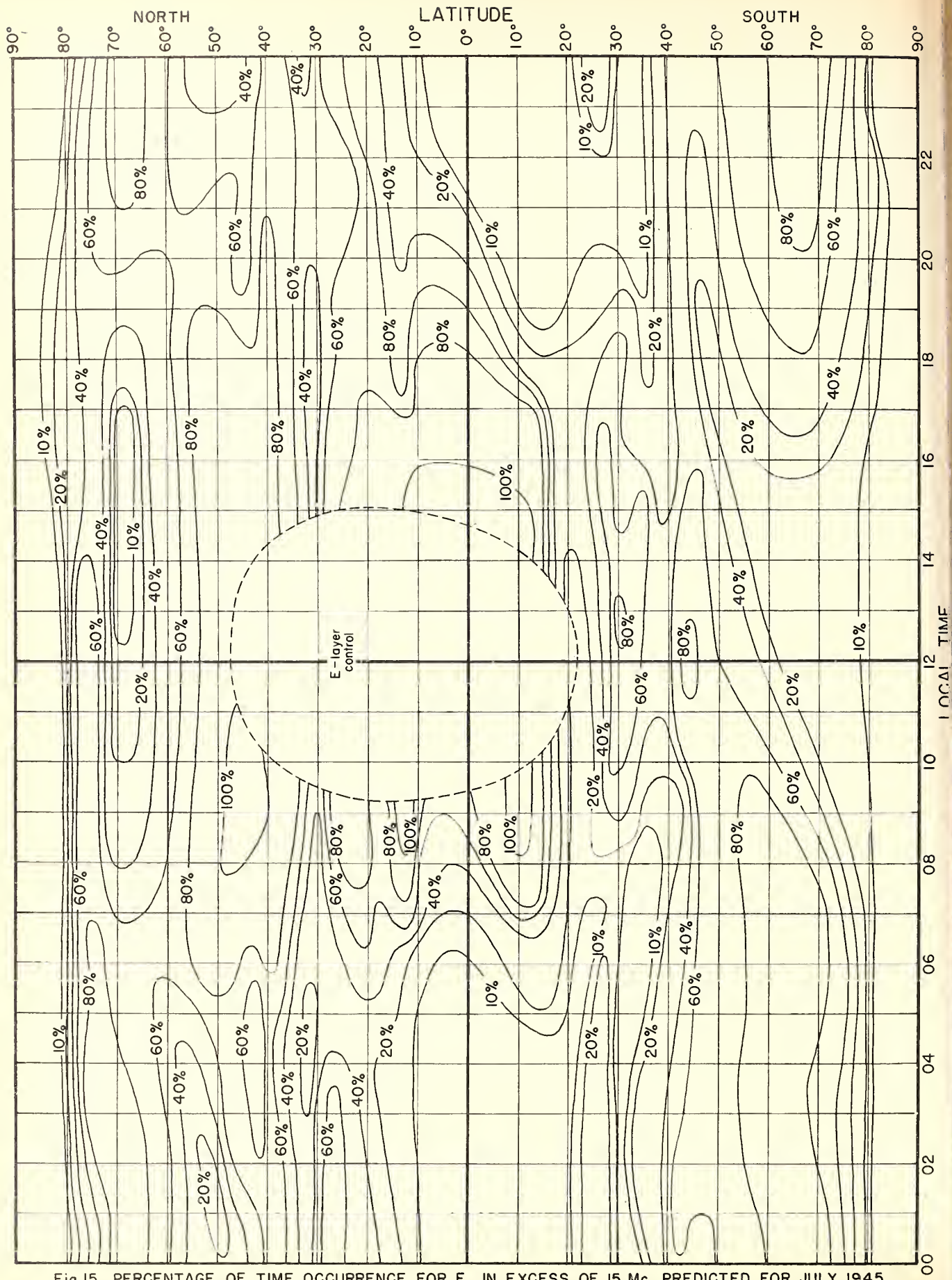
Fig. 15. PERCENTAGE OF TIME OCCURRENCE FOR E_s IN EXCESS OF 15 Mc, PREDICTED FOR JULY, 1945.
