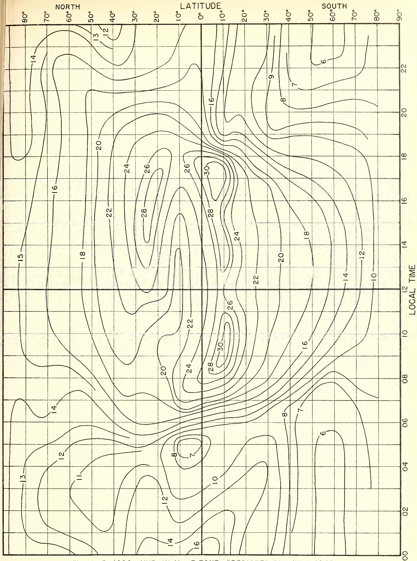
Fig. 10. F_2 4000 - MUF, IN Mc, E ZONE, PREDICTED FOR JULY, 1945.
