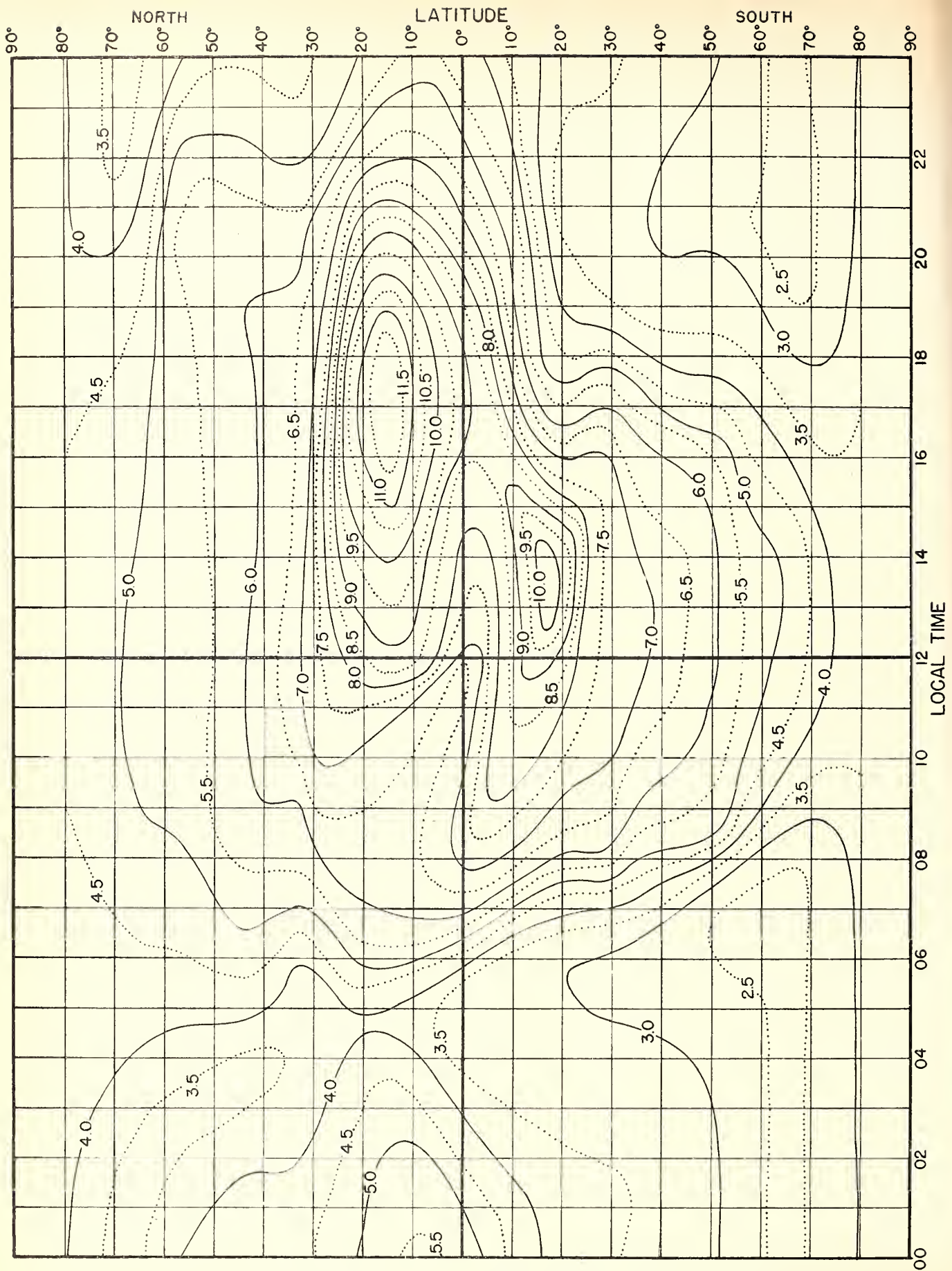
Fig. 7. F_2 ZERO-MUF, IN Mc, I ZONE, PREDICTED FOR JULY, 1945.
