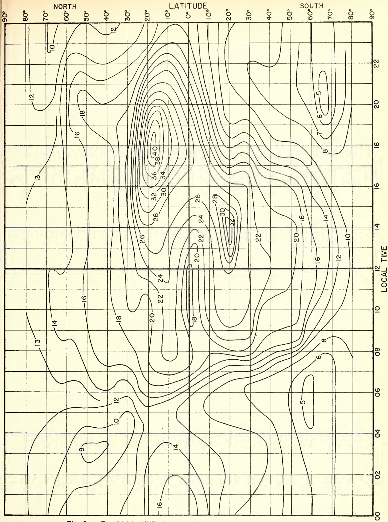
Fig. 8. F_2 4000-MUF, IN M_c, I ZONE, PREDICTED FOR JULY, 1945.
