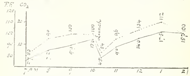
FIG. 2.—D. O. (Friday, October 8th.) Pulse frequency and CO 2 discharge rate, simultaneously at hour intervals during seven hours work at the coal face.
