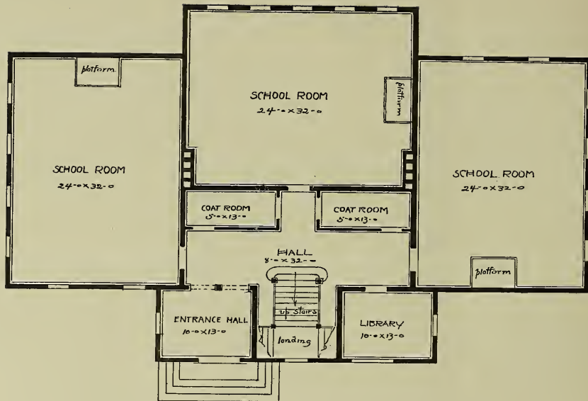
First Floor Plan for Frame School Building.
