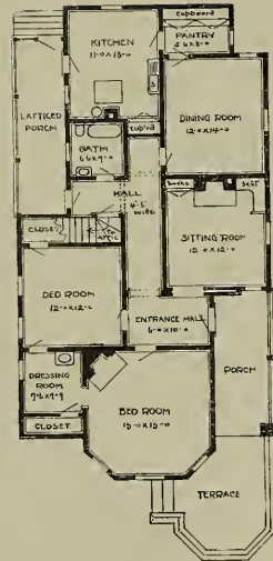
Floor Plan.
