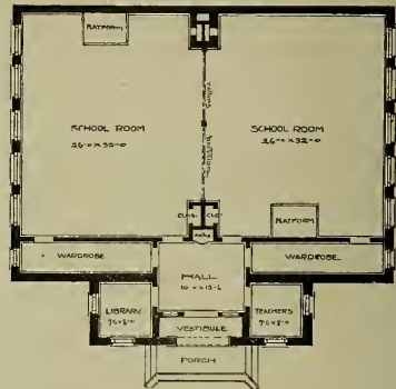
Perspective and Floor Plan for Two Room Brick School Building.
