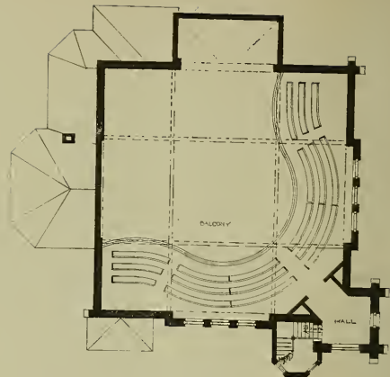
Balcony Plan.
