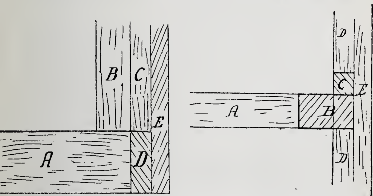
Figs 141 and 142.—A, Bearer. B, Runner. C, Guide on top of B. D, Lining of end E.
