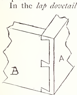
Fig. 85.—Lap Dovetail.
