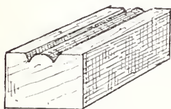
Fig. 60.—Bead.
