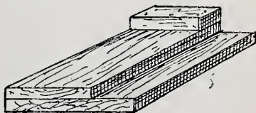
Fig. 51.—Shooting Board.
