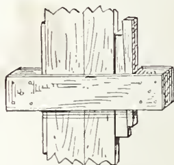
Fig. 50.—Improved Cramp.
