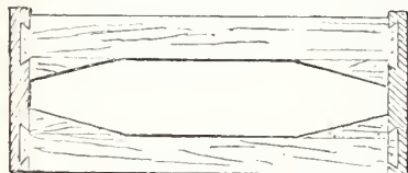
Fig. 87.—Dovetailed Top-bearers.
