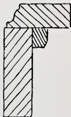
Fig. 151. Lining of Plinth.
