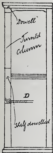
Fig. 163.—End Elevation.
