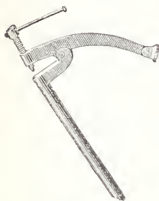
Fig. 40.—Bench Holdfast.
