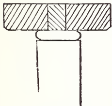
Fig. 170.—Fitting of Legs to Rails.
