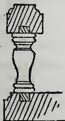
Fig. 172.—Fitting of Spindles.
