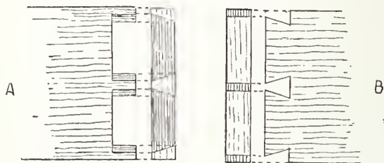
Fig. 82.—Plain Dovetails.
