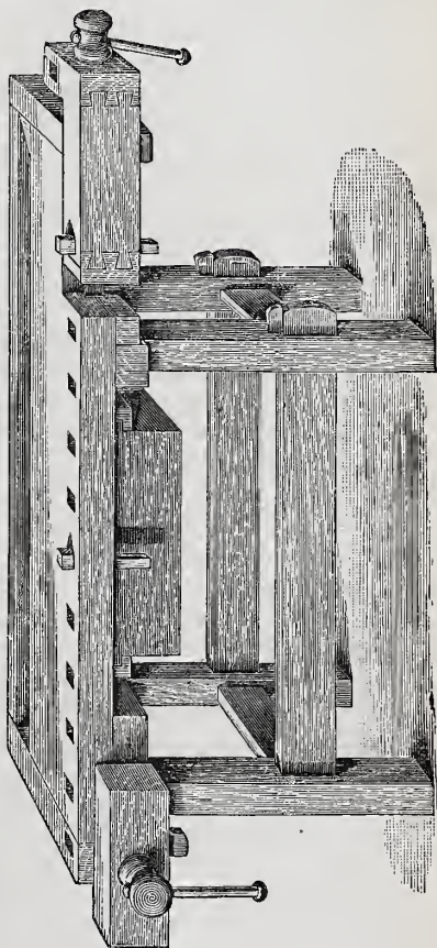
Fig. 69.—German Bench.
