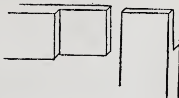
Fig. 99.—Halved Corner Joint.
