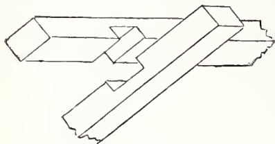
Fig. 100.—Halved Joint.
