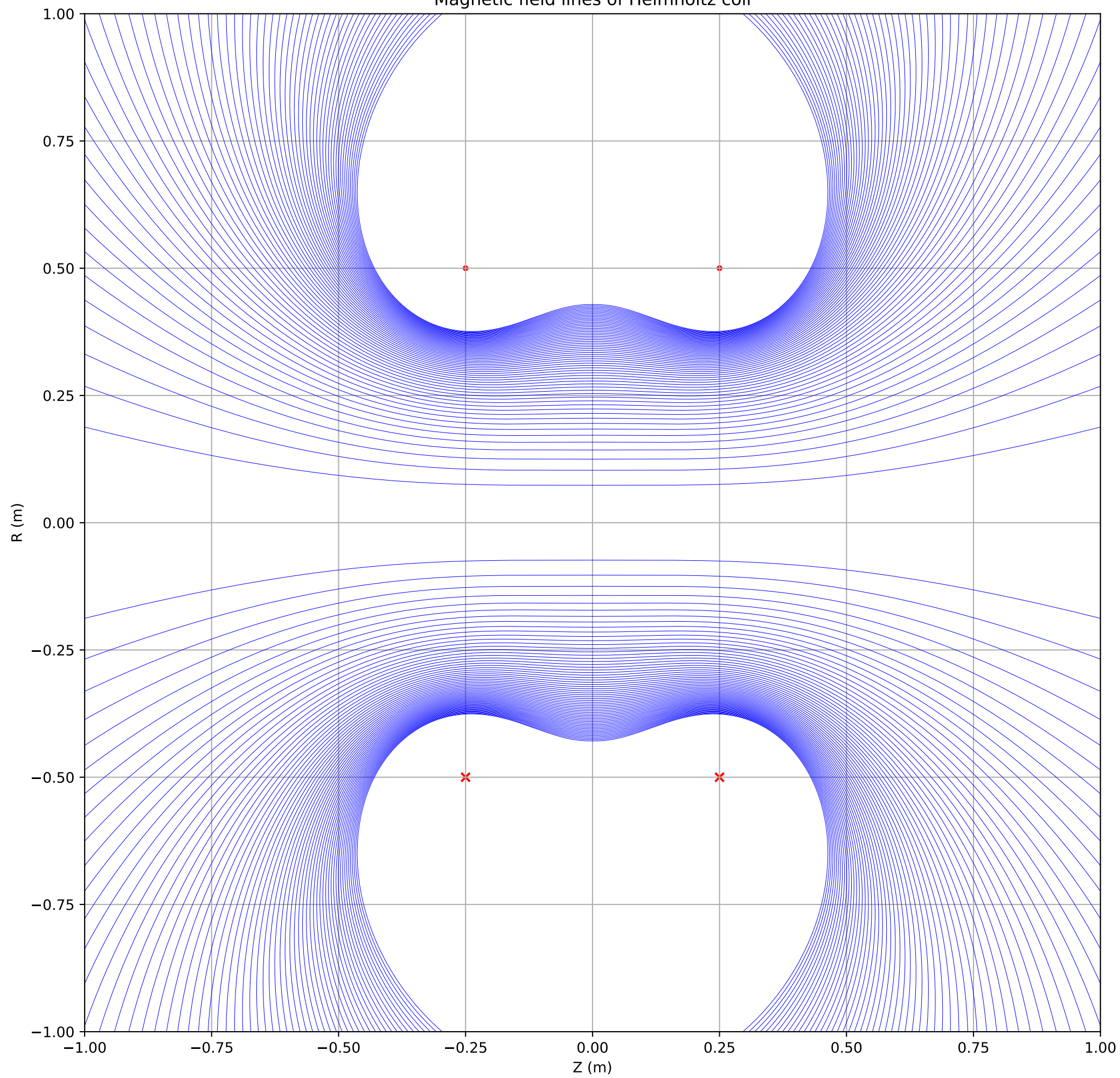
Magnetic field lines of Helmholtz coil
