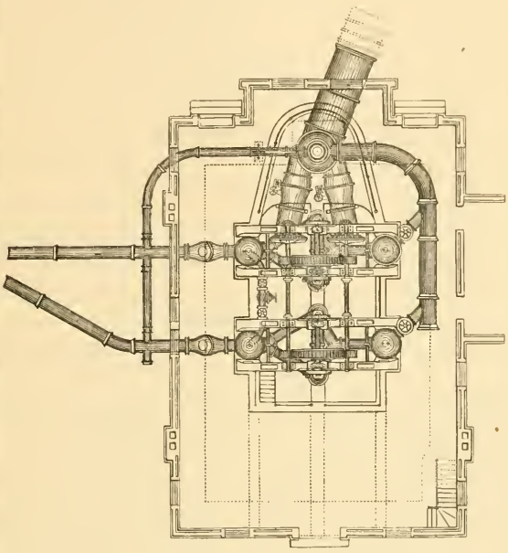
MANCHESTER WATER WORKS PLAN OF PUMP-HOUSE AND PUMPS J. T. Fowler, Civil Engineer DRAWN BY J. T. F. 1871
