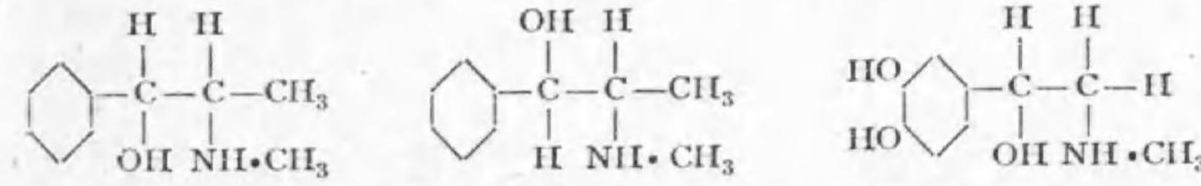
1-Phenyl-methylamino-propanol M.P. 216°-217° d,l-Phenyl-methylamino-propanol M.P. 186°-188° l-Orthodioxo-phenylethanol-methylamin
