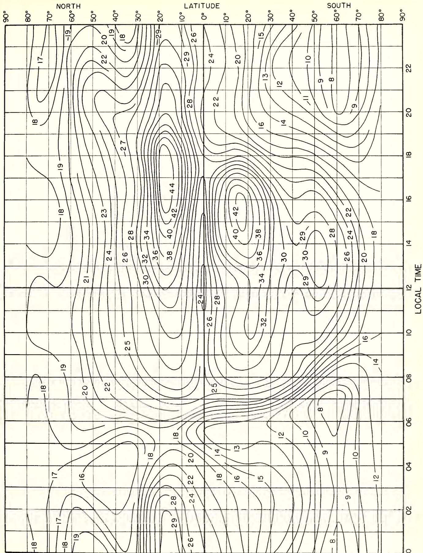
Fig. 8. F_2 4000-MUF, IN Mc, I ZONE, PREDICTED FOR JUNE, 1946.
