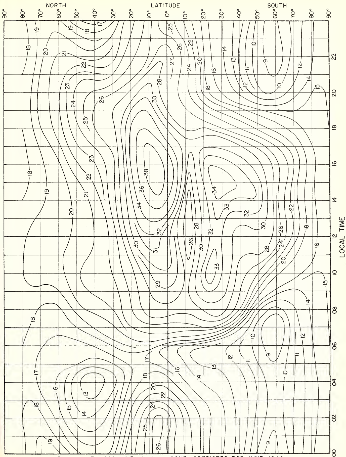
Fig. 6. F_2 4000-MUF, IN Mc, W ZONE, PREDICTED FOR JUNE, 1946.
