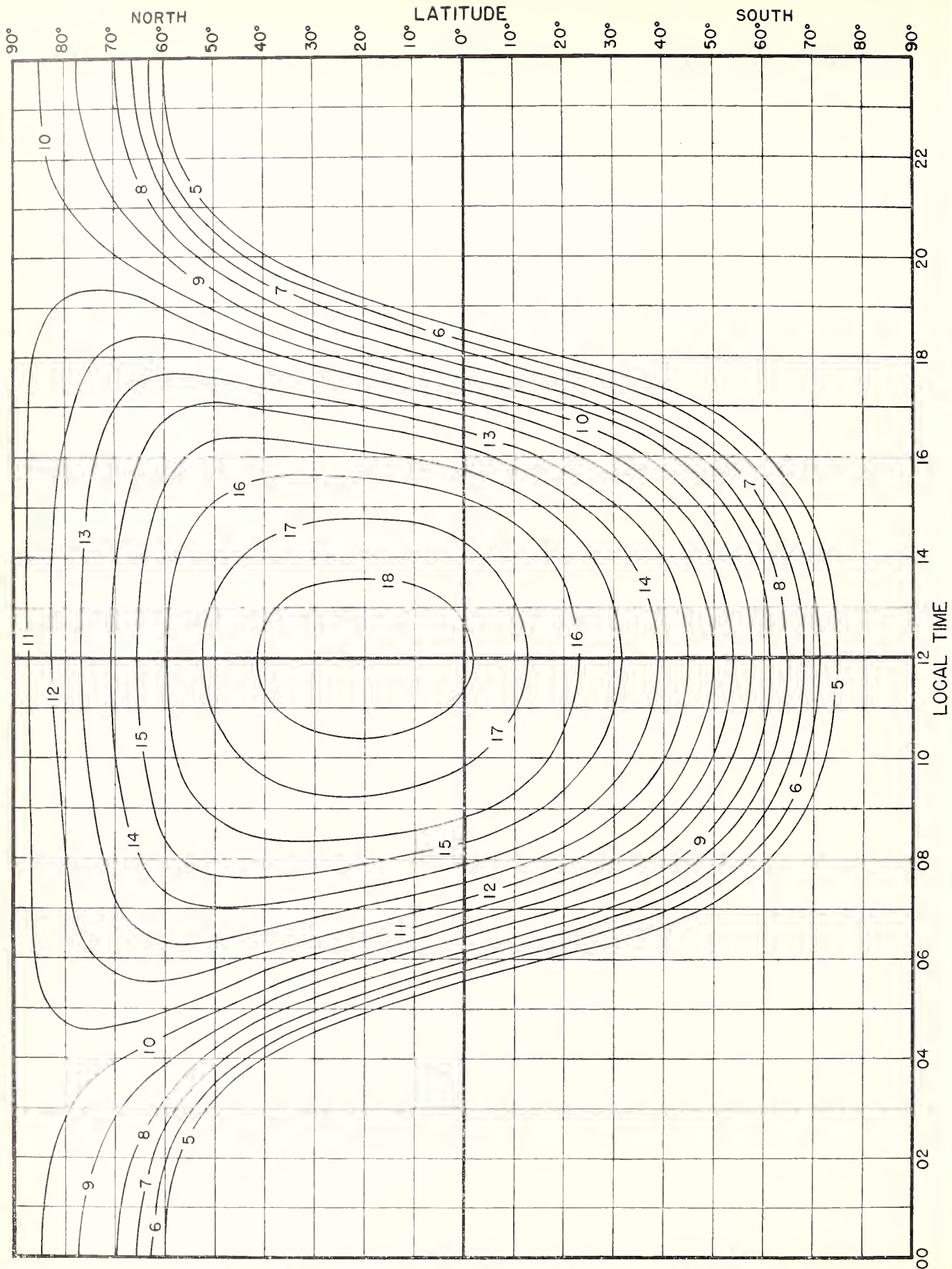
Fig. 11 E-LAYER 2000-MUF, IN Mc, PREDICTED FOR JUNE, 1946.
