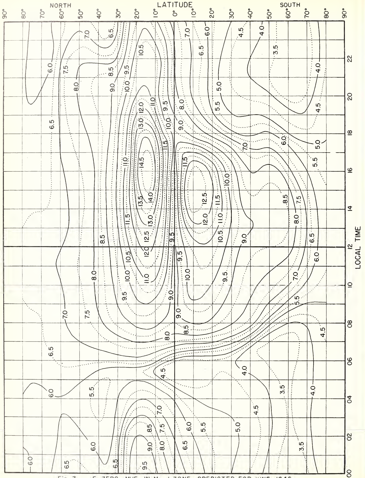
Fig 7. F 2 ZERO-MUF, IN Mc, I ZONE, PREDICTED FOR JUNE, 1946.
