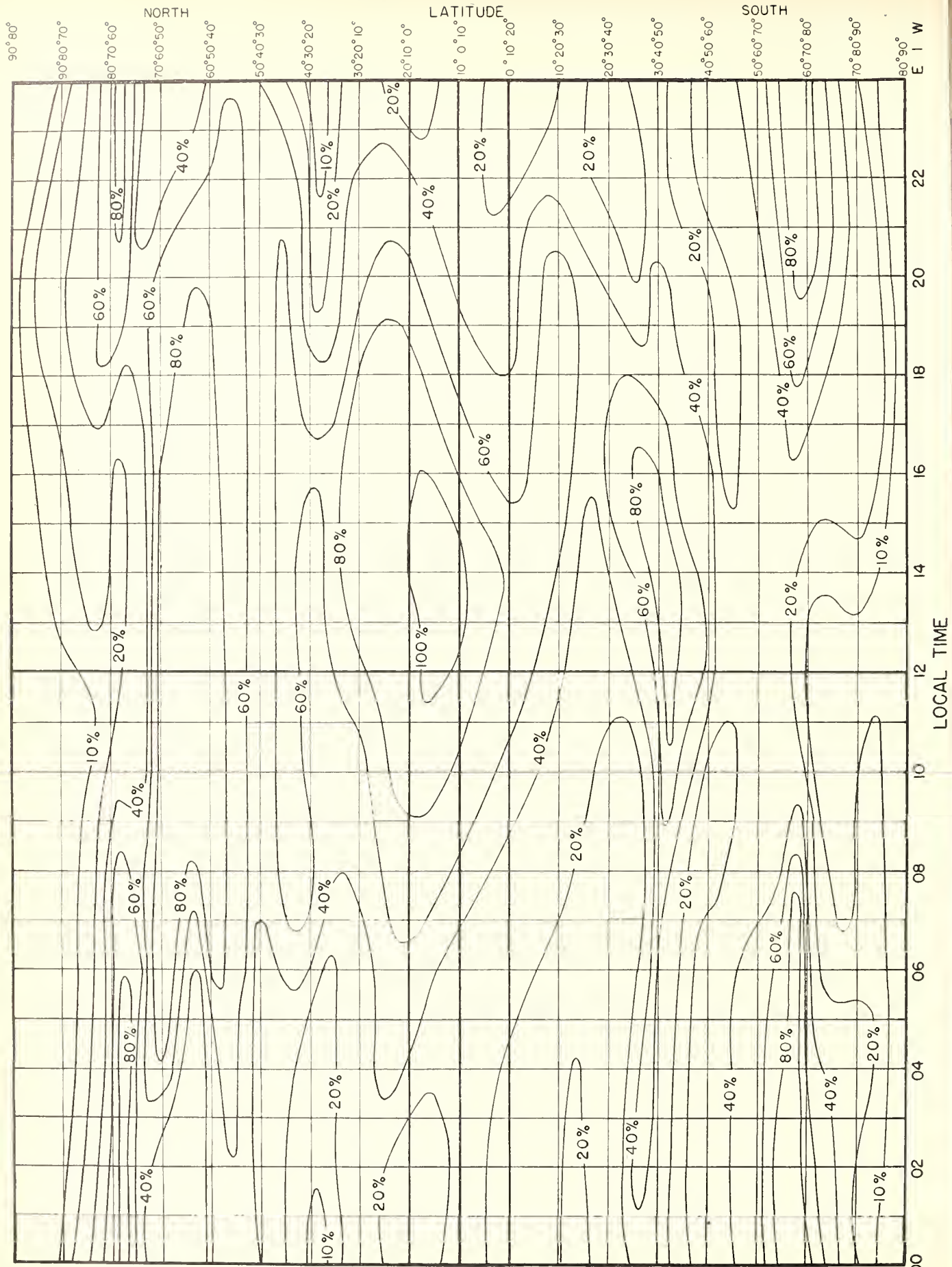
Fig. 15. PERCENTAGE OF TIME OCCURRENCE FOR E s IN EXCESS OF 15 Mc, PREDICTED FOR JUNE, 1946.
