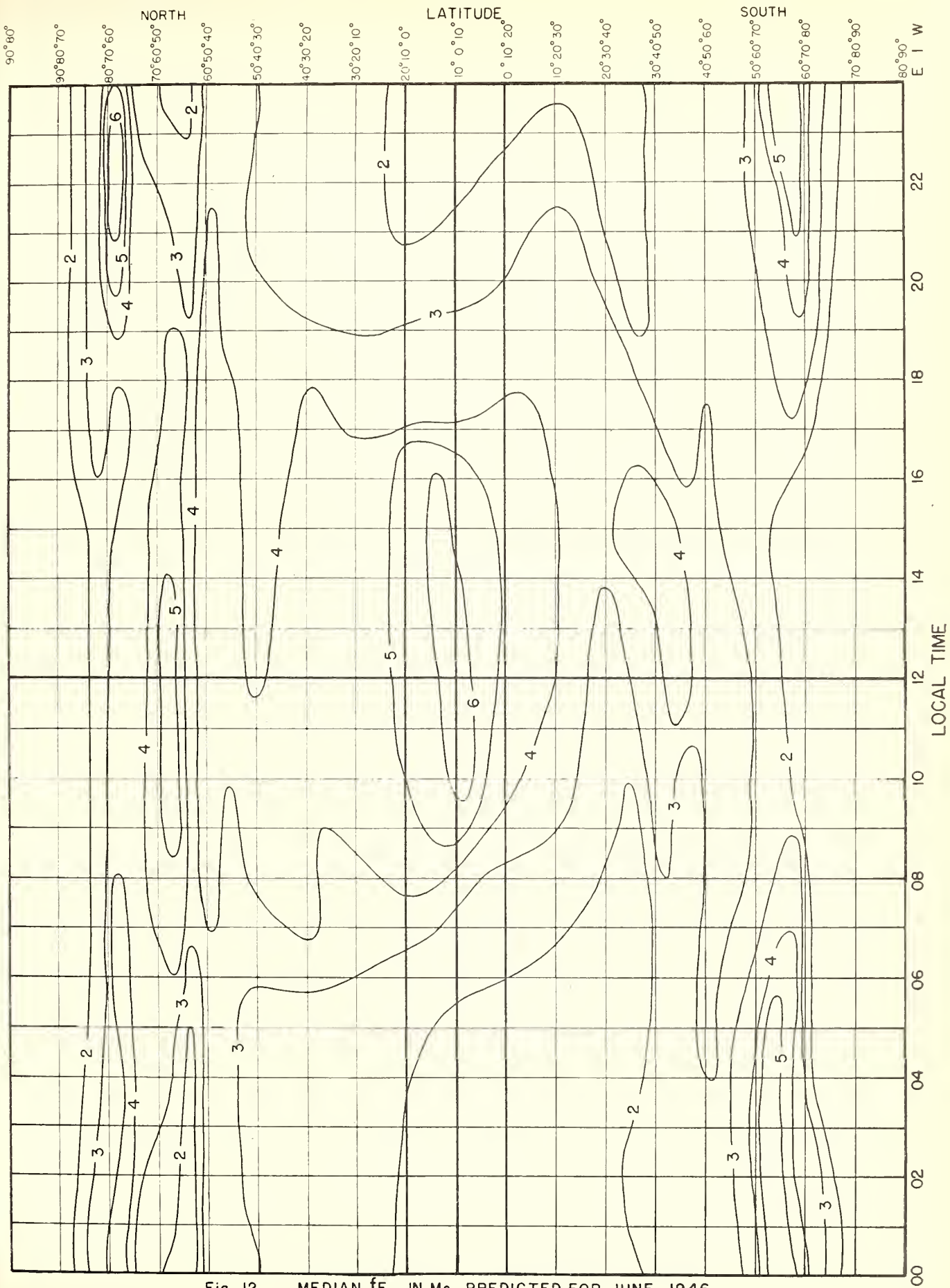
Fig. 12. MEDIAN fE_s , IN Mc, PREDICTED FOR JUNE, 1946.
