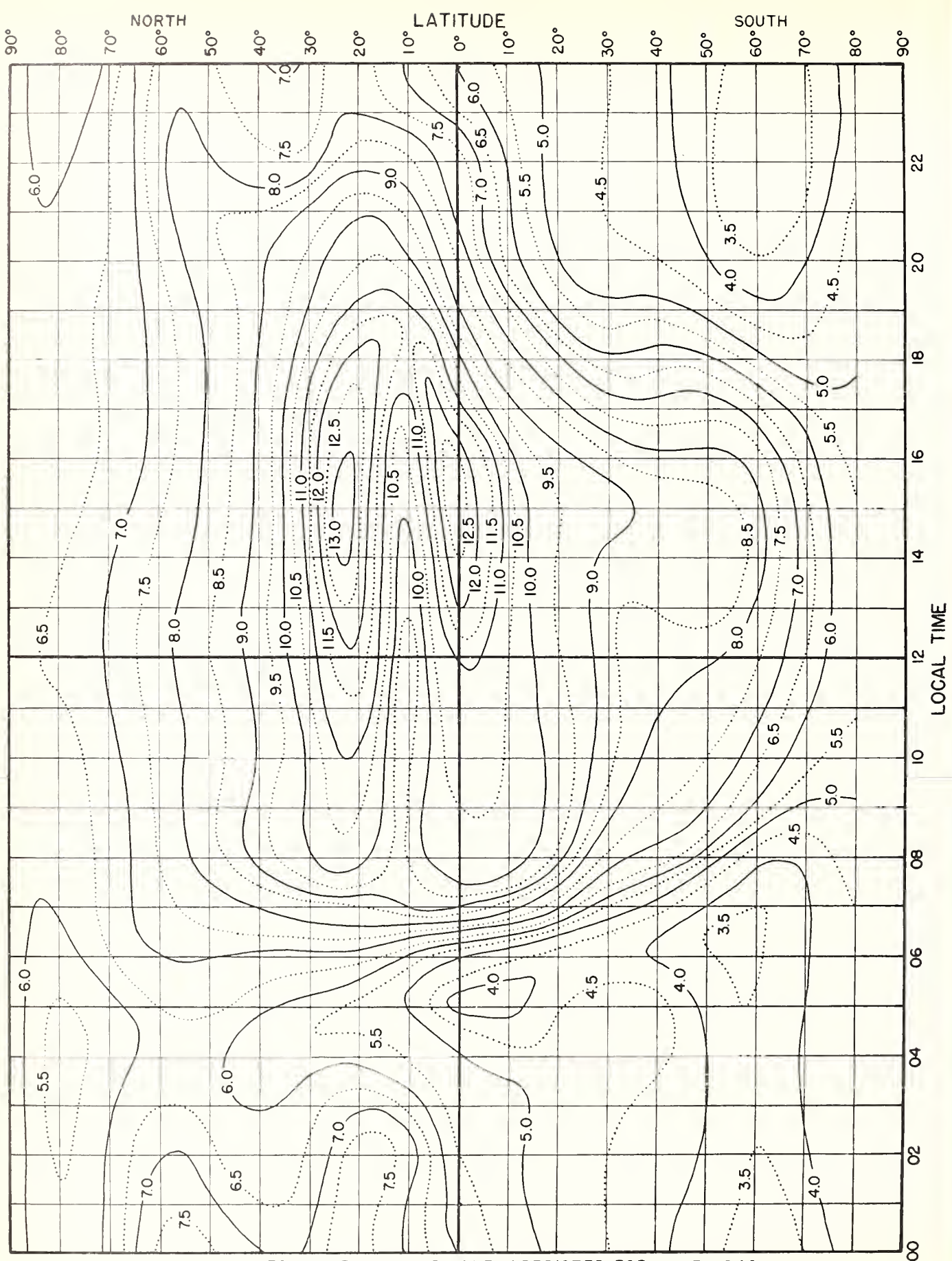
Fig. 9. F_2 ZERO-MUF, IN Mc, E ZONE, PREDICTED FOR JUNE, 1946.
