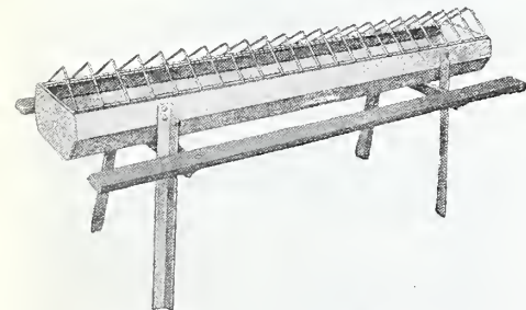
No. 25S—5 feet long. Trough 9 inches wide, 4 7/8 inches deep, holds 40 pounds or 4 1/2 pecks dry laying mash. Serves 60 hens. Three in carton K.D. Weight 53 lbs. Second class freight L.C.L. Price: $6.00, not prepaid.
