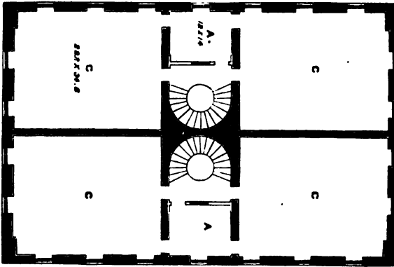
Fig. 2.—SECOND FLOOR.
