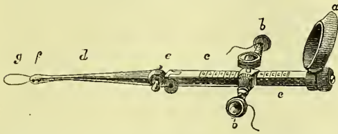
FIG. 283. Hilton's nasal polypus snare. a , ring for the surgeon's thumb; b , b , movable cross-piece, pushed backwards and forwards by the fore and middle fingers, so as to advance and retire the loop g , which in practice is far larger than is here shown. The stem c is hollow for the ends of the wire to run in. They are wound round the cross-piece. e is a hinge-joint, by means of which the stalk d which is in the nose can be placed at the requisite angle with the stem c . Its bulbous end, f , is perforated by two holes to convey the wire. The end of the wire is pushed round the polypus either with the fingers or a kind of fork.
