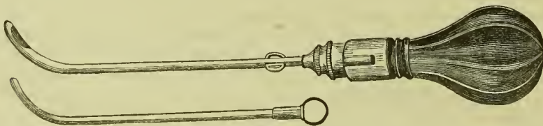
FIG. 383. Clover's syringe. The indiarubber ball is filled with water. This is injected into the bladder with the instrument as nearly vertical as may be. Then the ball is allowed to expand, drawing the water and fragments of stone up the eye of the instrument. The fragments fall into the glass receptacle by their own weight, and the process can be repeated several times without any risk. If a fragment too large to pass should fall into the eye of the catheter it must be dislodged before withdrawing the instrument. This is accomplished by passing the stem figured below the catheter.
