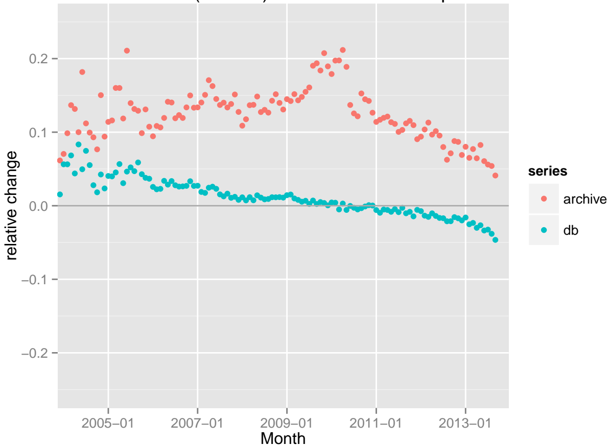
Active Editors ( eswiki ): deviation from dump data
