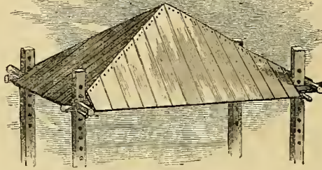
Fig. 2.—BOARD ROOF TO BARRACK.
