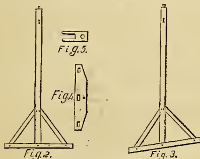
BRACED POSTS.
