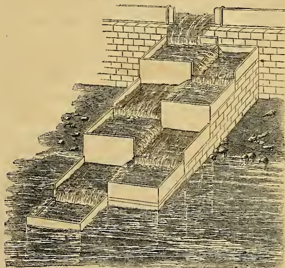
Fig. 1.—FISH-STAIRS AT LOWELL, MASS.
