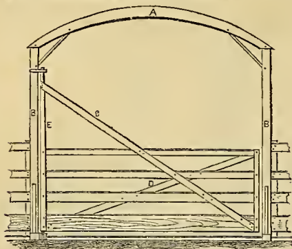
FRAME GATE.
