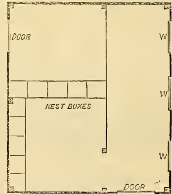
Fig. 2.—PLAN OF HEN HOUSE.
