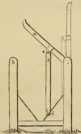
Fig. 2.—GATE OPEN.
