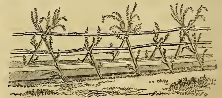
Fig. 2.—WILLOW FENCE WITH RIDGE.
