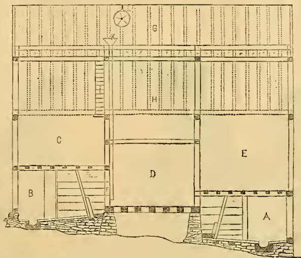
Fig. 2.—EAST AND WEST SECTION OF BARN.
