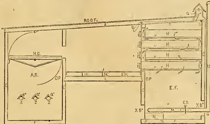
Fig. 1.—LONGITUDINAL SECTION OF DRYING HOUSE.
