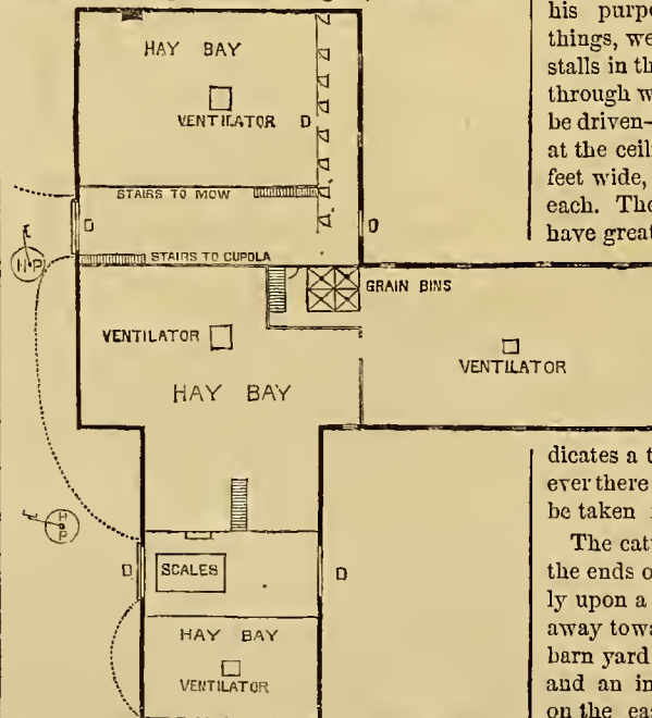
Fig. 2.—PLAN OF HAY FLOOR.
