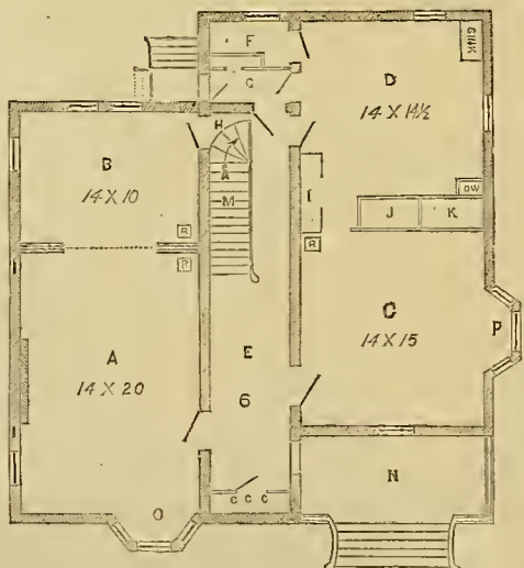
Fig. 2.—FIRST FLOOR OR GROUND PLAN.
