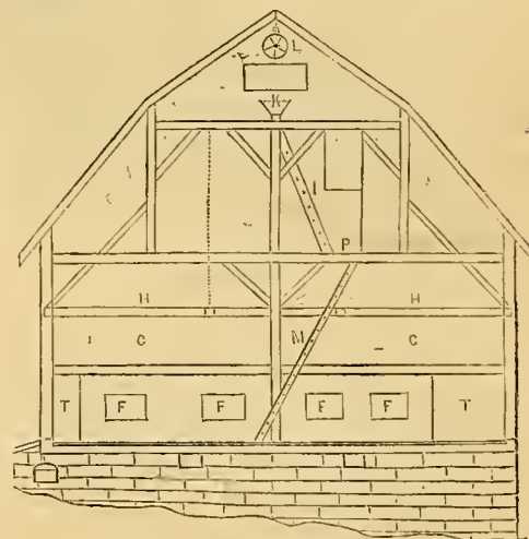
Fig. 3.—CROSS-SECTION OF BARN.
