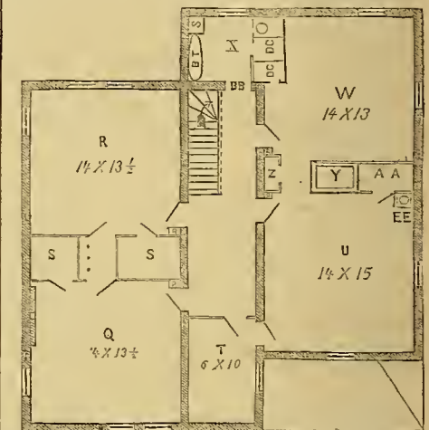
Fig. 3.—SECOND FLOOR OR CHAMBER PLAN.
