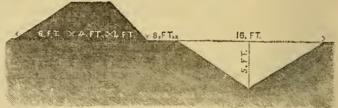
EMBANKMENT.
