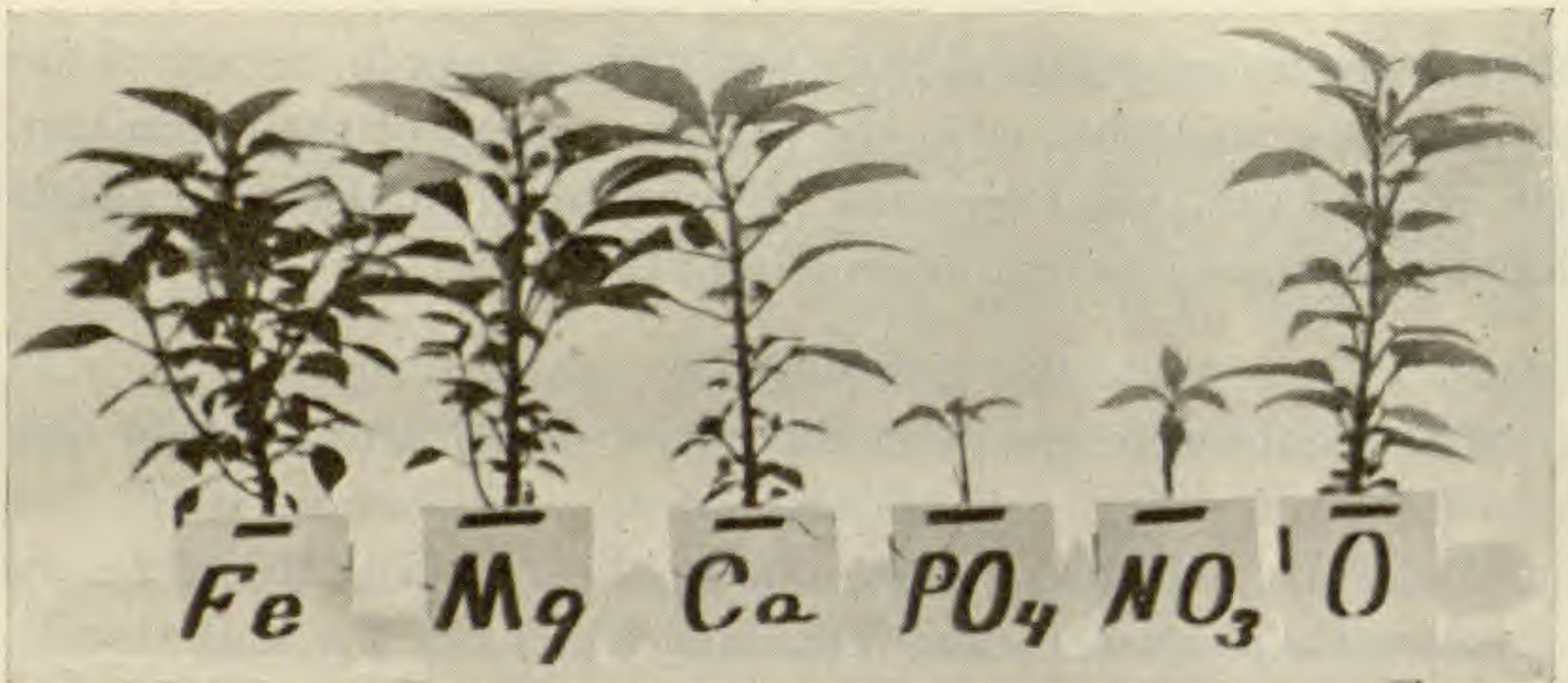
FIG. 1.— Coleus plants grown in various nutrient solutions: —Fe, iron lacking but all other essential elements present; —Mg, magnesium lacking, etc.; —O, all essential elements present; notice dwarfed condition of plants lacking phosphate or nitrate.
