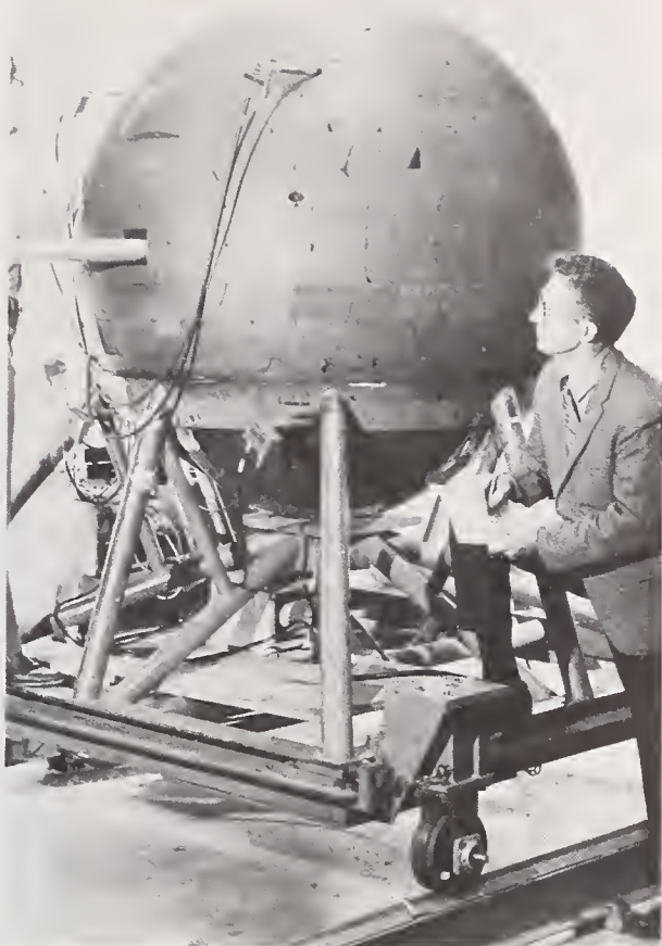
Fig. 1. The Macklin Graphite Sphere neutron Detector with C.H. Johnson at the Oak Ridge National Laboratory.
