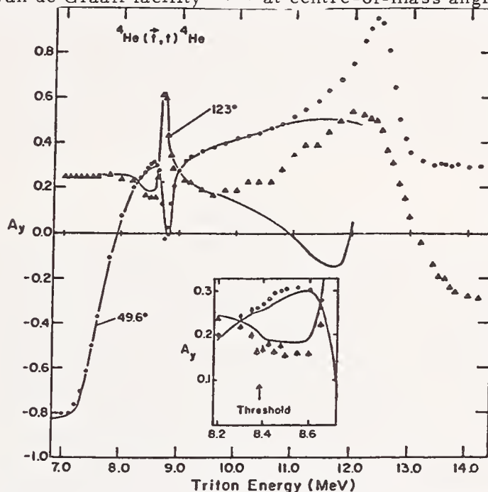
Fig. 9 : Excitation function for {}^4\text{He}(t,t){}^4\text{He} analyzing power 38 .
