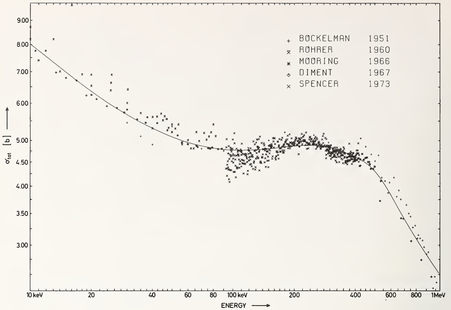
Fig.3 \sigma_{\text{tot}} from 10 keV to 1 MeV.
