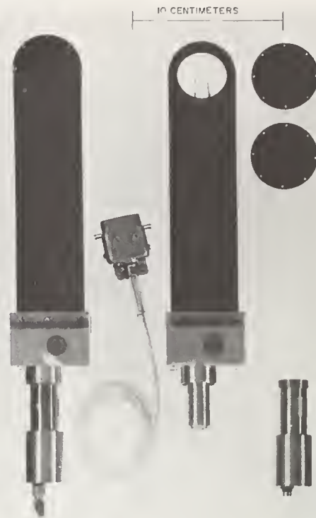
Fig. 4. Photograph of transmission ionization chamber monitor used in INDI experiment.
