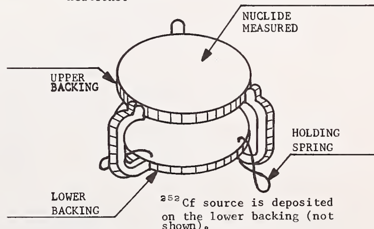
Fig. 2. Assembly for holding the ^{252}\text{Cf} source and fissionable nuclide target.
