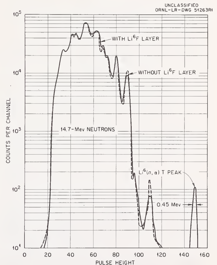
Figure 2. Pulse-height spectra for Li sandwich detector 14 using surface-barrier diodes.
