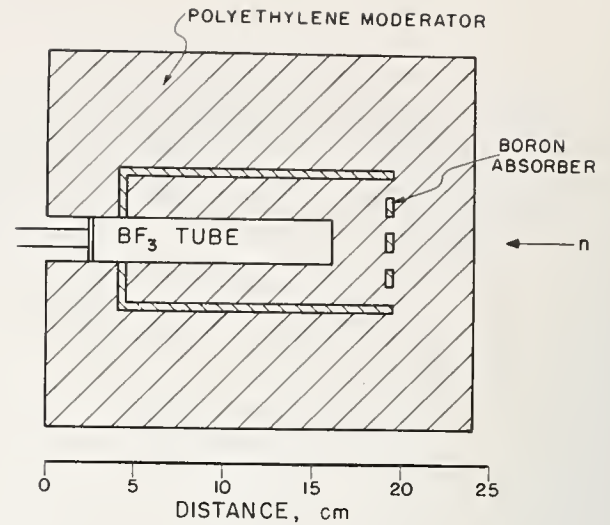
Fig. 8 Diagram of larger moderating neutron rem counter
