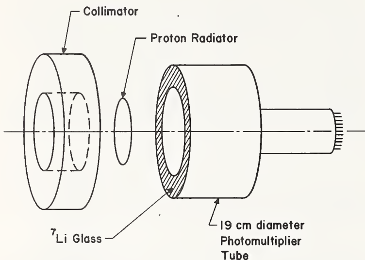
Fig. 4. Geometrical arrangement for proposed proton-recoil detector.
