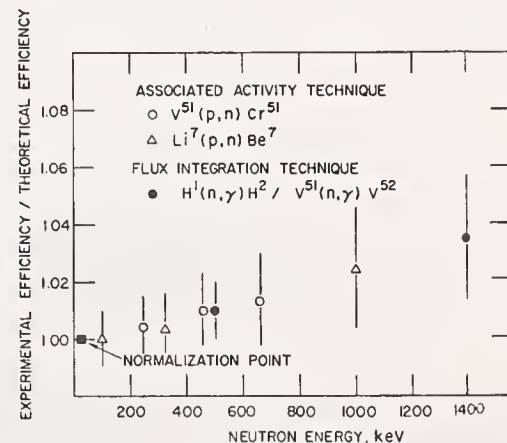
Fig. 3. The ratio of the experimental efficiency to the theoretically calculated efficiency of the grey neutron detector.
