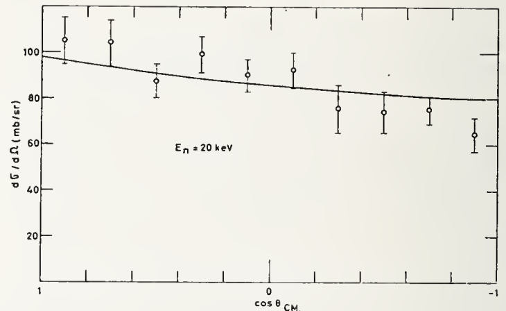
Fig. 1. Differential cross section at 20 keV from the data of reference 2. Solid curve is theoretical fit of Mahaux and Robaye. 4
