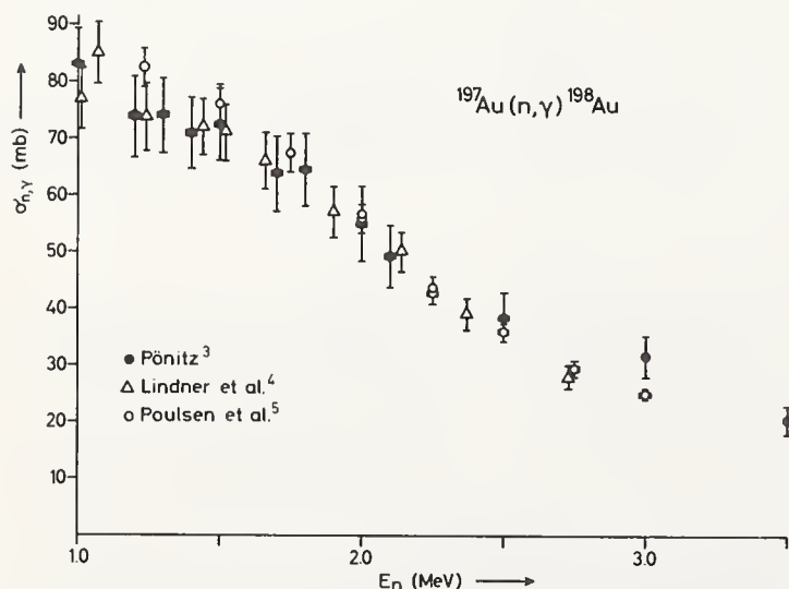
Fig. 2 : Comparison of prompt \gamma -detection (full symbols) and activation (open symbols) results for Au(n, \gamma ).
