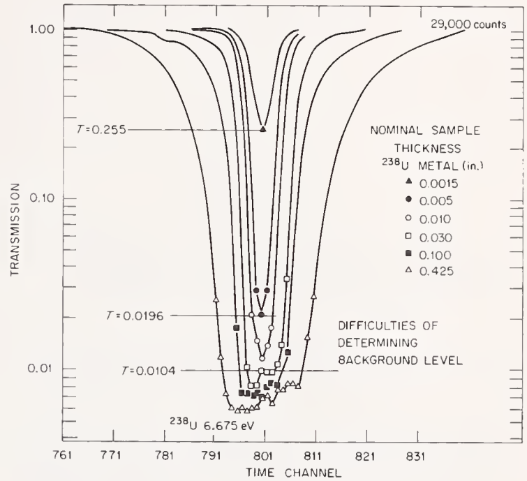
Figure 8. Neutron intensity near 6.7 eV observed through a broad range of {}^{238}\text{U} absorbers. From the work of Ref 24.
