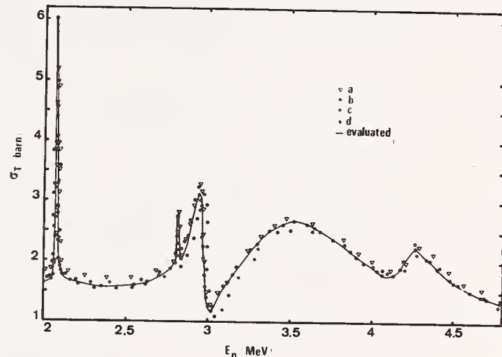
Fig.4. Comparison of neutron total cross sections of carbon between 2 and 5 MeV (a = ref. 9 , b = ref. 20,23 , c = ref. 11 , d = ref. 13 , the evaluated curve is from ref. 8 ).
