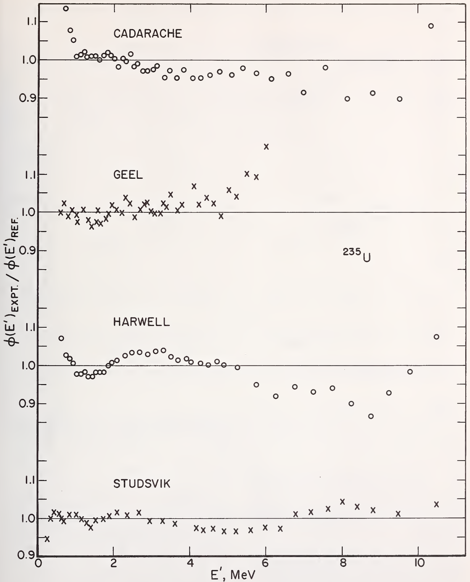
Figure 2. Ratio of Experimental Data for Neutron-Induced Fission in ^{235}\text{U} to a Reference Watt Spectrum 2 with A = 1.0193 , B = 2.3075 and \bar{E}' = 2.027 MeV.
