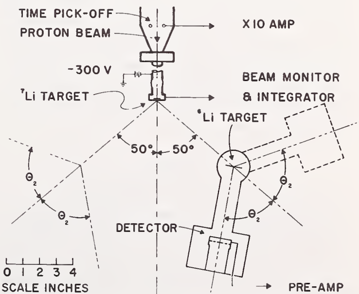
Fig. 10 : A plan view of the experimental arrangement to measure the analysing power of the {}^6\text{Li}(n,t){}^4\text{He} reaction.
