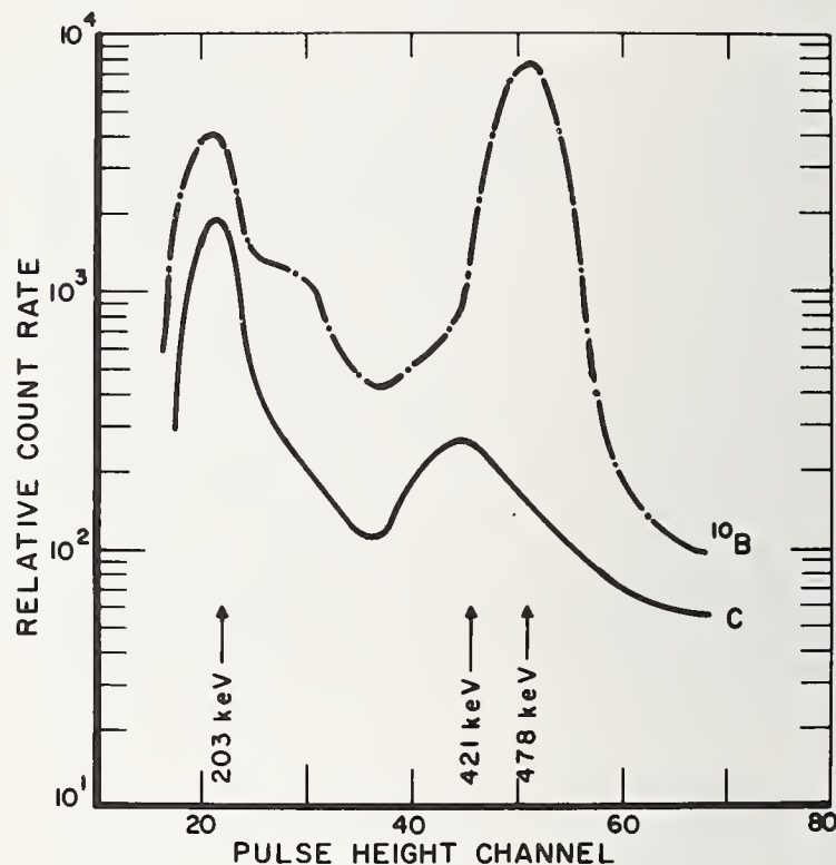
Figure 4. Pulse-height distributions for 510-keV neutrons for a NaI detector system used in implementing the ^{10}\text{B}(n,\alpha_1\gamma)^7\text{Li} cross section. The upper curve was obtained with a ^{10}\text{B} sample. The lower curve was obtained with a carbon scatterer. The arrow labeled 203 keV shows the position of the (n,n') gamma-ray from iodine. The arrow labeled 421 keV shows the position of a peak which is a mixture of 438-keV gamma-rays from sodium and 417-keV gamma-rays from iodine.
