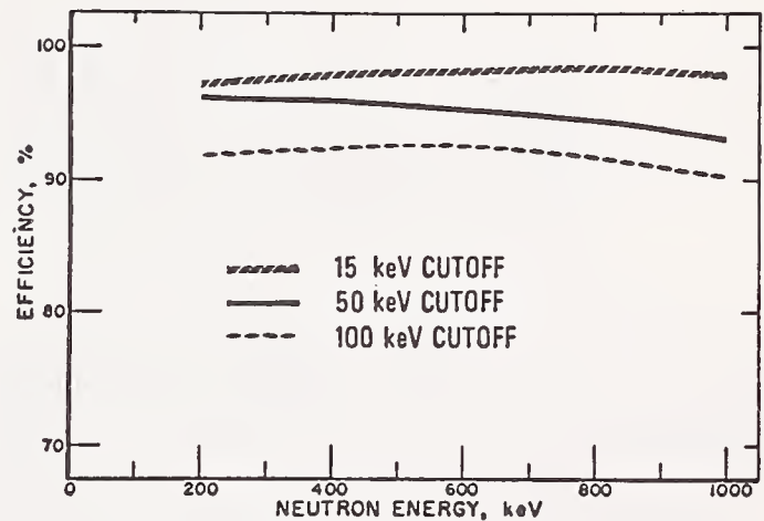
Fig. 9. Calculated efficiencies of the NBS Black Detector for different lower level cutoffs. Calculations were done with the computer program Carlo-Black.
