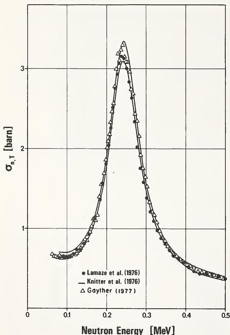
Fig. 2 : {}^6\text{Li}(n,t){}^4\text{He} cross section is plotted versus incident neutron energy. \bullet , - and \Delta are results of Lamaze et al. 2 , Knitter et al. 18 and Gayther 3 respectively.
