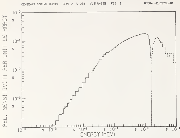
Fig. 3. Relative Sensitivity per Unit Lethargy of \langle 28\sigma_c/28\sigma_f \rangle_c in GODIVA with Respect to the ^{235}\text{U}(n,f) Cross Section.
