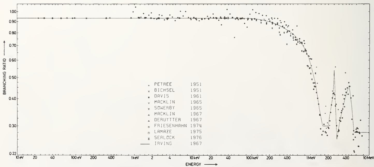
Fig.10 Branching ratio \sigma(n,a_1) / \sigma(n,a_0) + \sigma(n,a_1) from 10 eV to 10 MeV.
