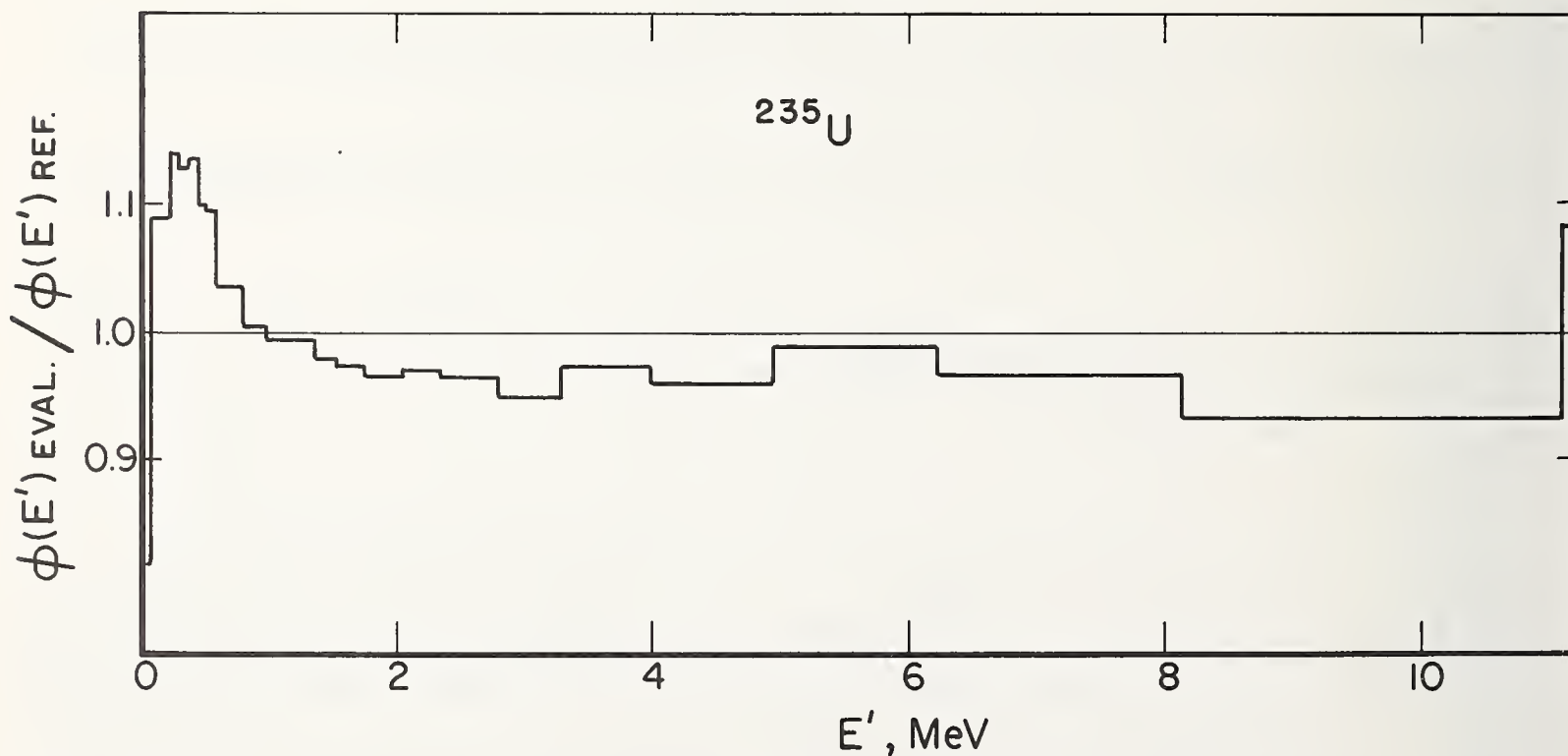
Figure 7. Ratio of NBS Evaluated Spectrum for Neutron-Induced Fission in ^{235}\text{U} to a reference Watt spectrum 2 with A = 1.0193 , B = 2.3075 and \bar{E}' = 2.027 \text{ MeV} .
