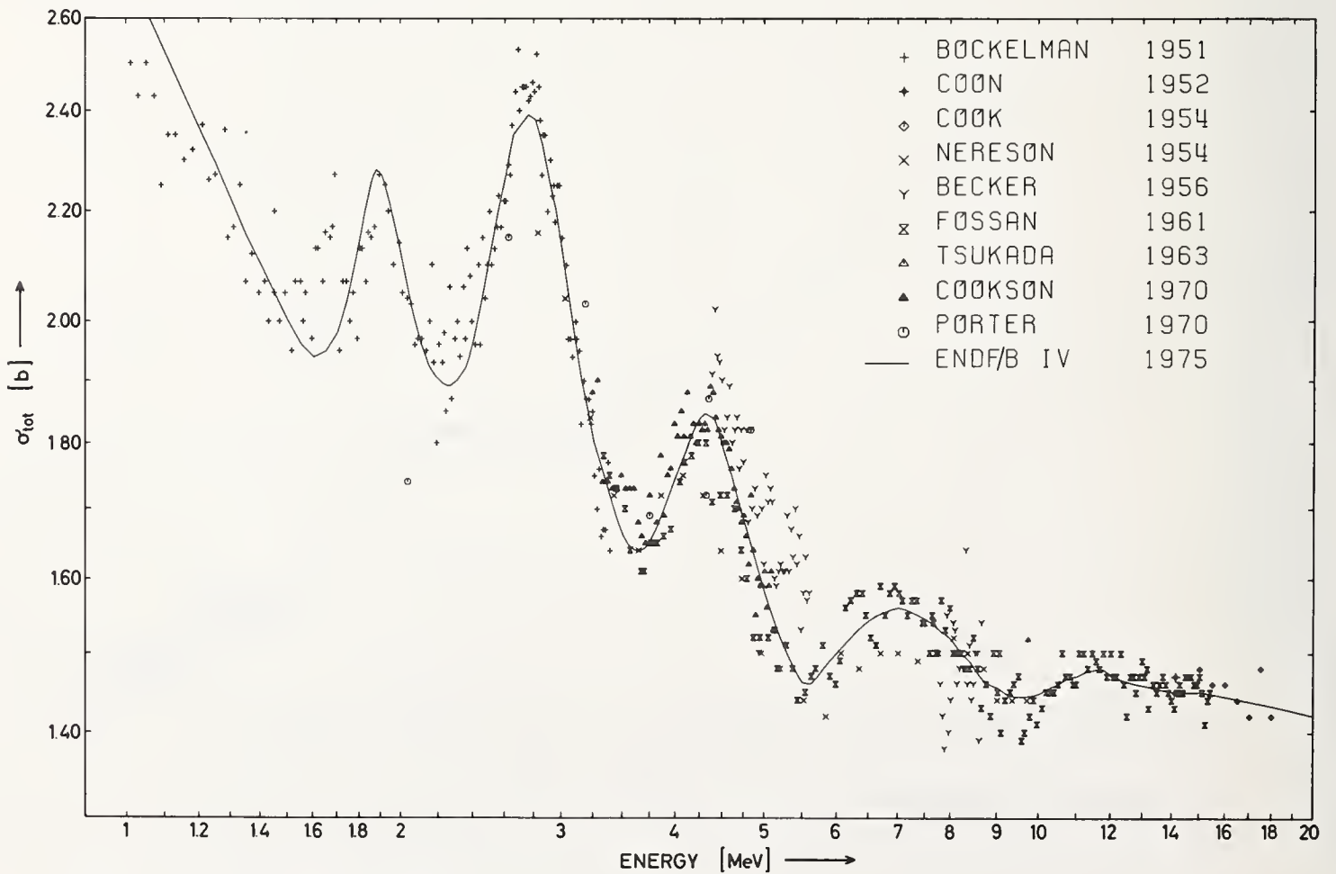
Fig.4 \sigma_{\text{tot}} from 1 MeV to 20 MeV.
