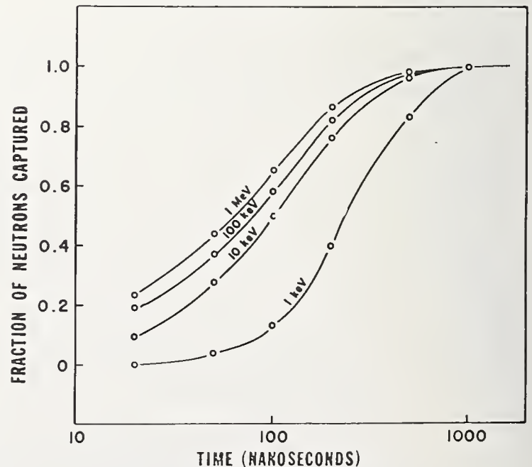
Fig. 18. Time response of LLL detector as a function of incident neutron energy.
