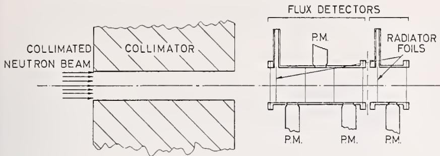
KFK PROTON-RECOIL TELESCOPE
