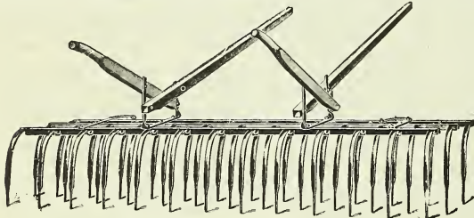
Hallock 7½-foot Walking Weeder.
