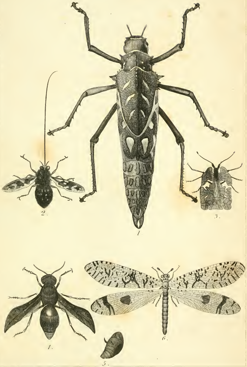
1. Pneumora scutellaris .
