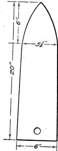
FIG. 3.—Wooden stretcher for muskrat skins.
