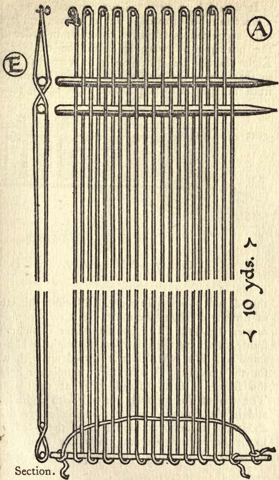
FIG. 16.—The Warp displayed.
