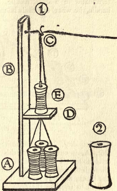
FIG. 57.—Doubling Stand.
