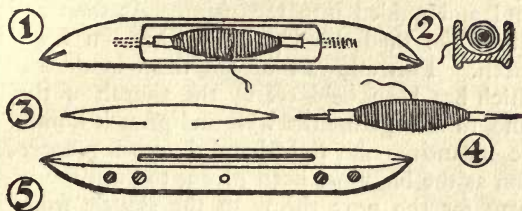
FIG. 51.—Hand-shuttle.
