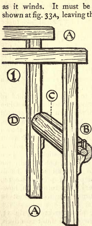
FIG. 33.—Loom Posts with Roller.
