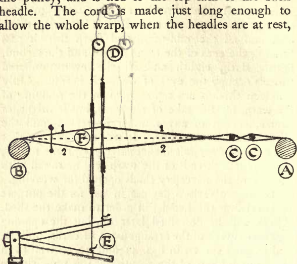
FIG. 44.—Section of Opened Warp.
