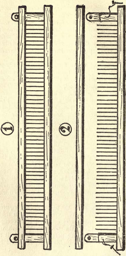
FIG. 28.—The Raddle.
