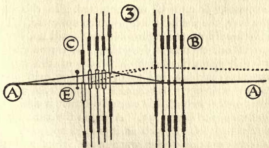
FIG. 92.—Various Two-harness Sheds.
