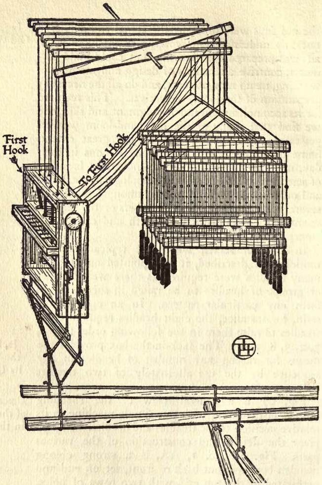
FIG. 97.—The Jack-in-the-box.
