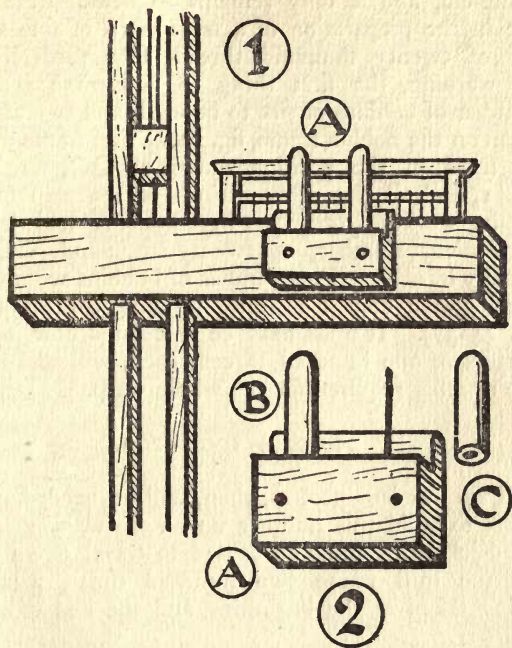
FIG. 26.—The Gatherer.
