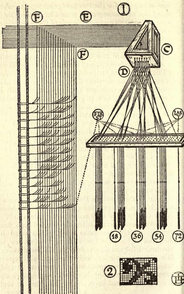
FIG. 105 — Mechanism of the Draw-loom.
