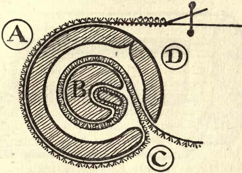
FIG. 94A.—Breast Roller of Velvet Loom.
