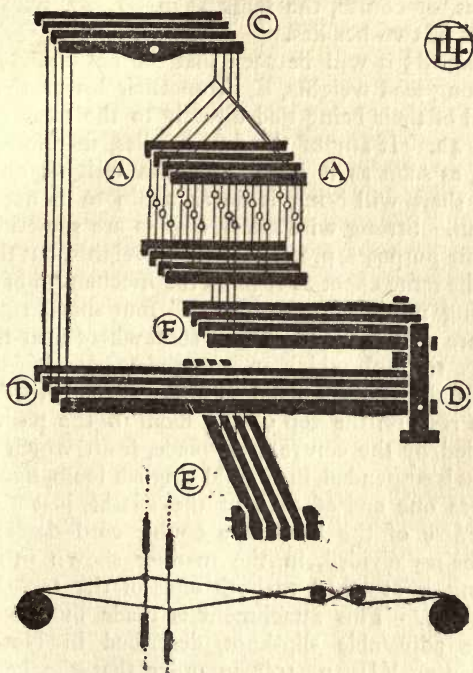
FIG. 85A.—Shedding Motion.
