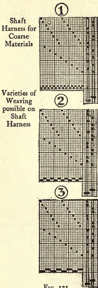
FIG. 121 Tie-ups for Tabby.
