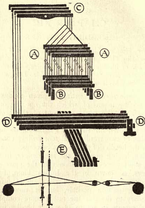
FIG. 85.—Shedding Motion.
