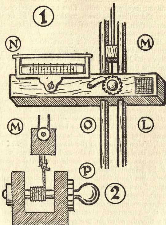
FIG. 23.—The Heck-block.
