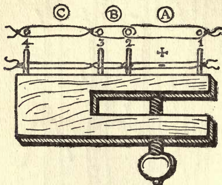
FIG. 49.—Headle or Leash Gauge.
