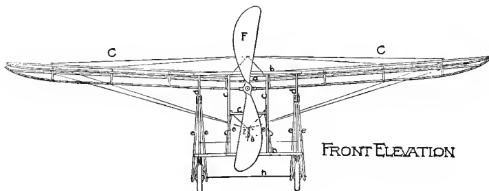
"IDEAL" BLERIOT MONOPLANE. THREE-FOOT FLYING-MODEL. DESIGN "B"
