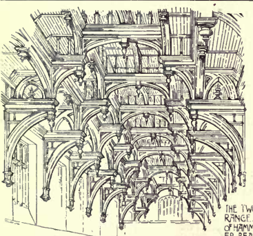
(E) DOUBLE HAMMER-BEAM ROOF MIDDLE TEMPLE HALL, LONDON. SPAN 40'0"
