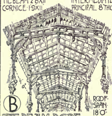
TIE BEAM ROOF TRINITY CHAPEL, CRORENCSTER THIS FORM USED THROUGHOUT MIDDLE AGES
