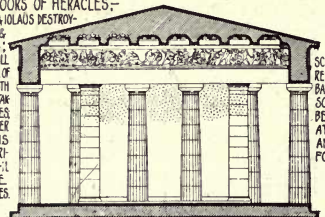
B TRANSVERSE SECTION & E. PORTICO
