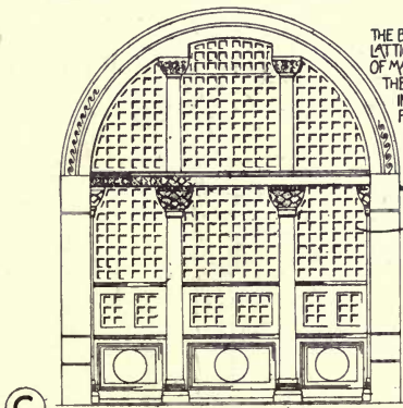
(C) ELEVATION WINDOW FROM THE GALLERY (GYNAECEUM) S. SOPHIA CONSTANTINOPLE
