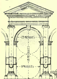
D DOORWAY OR PORTION OF IONIC COLONNADE WITHOUT PEDESTALS.
