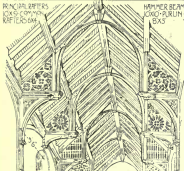
(D) HAMMER-BEAM ROOF TRINCH CHURCH, NORFOLK. SPAN 19'0" BEAM WITHOUT COLLAR
