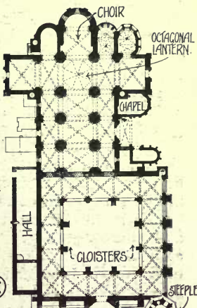
E LERIDA CATHEDRAL A.D. 1203-1278. PEDRO DE PENAFREYTA ARCHT. OCTAGONAL LANTERN OVER CROSSING ON PENDENTIVES. EXTERNAL ROOFS OF STONE.
