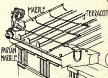
H VIEW OF LOWER ACROTERION
