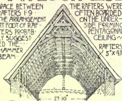
TRUSSED RAFTER ROOF. STOWE BARDOLOPH CHURCH, NORFOLK EARLY FORM USED TO OBTAIN HEADWAY
