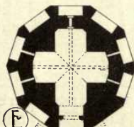
(F) HALF PLAN OF UPPER STOREY (G) HALF PLAN OF ROOF
