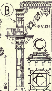
DIAGRAMS OF INDIAN ROOF CONSTRUCTION AFTER FERGUSSON - FIG. C SHOWS SECTION & PLAN LOOKING UP. COLUMNS LINTELS SUPPORT COURSES OF STONE SANS. FIG. B SHOWS METHOD OF STRENGTHENING LINTEL BY BRACKET.
