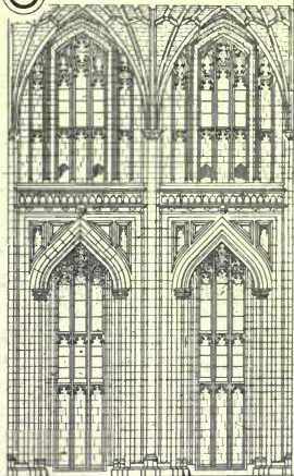
WINCHESTER CATHEDRAL. NAIVE, DATE 1359-1440
