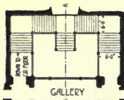
E PLAN AT FIRST FLOOR LEVEL BUCKLING HALL NORFOLK, 1620. THE GREAT STAIRCASE, AN IMPORTANT FEATURE IN ALL CAROLINE AND JACOBINE MANSIONS, HAS ELABORATELY CARVED NEWELS CROWNED WITH FIGURES, AND CARVED PENDANTS, AND BALUSTERS TREATED AS SMALL COLUMNS WITH ARCHING BETWEEN.
