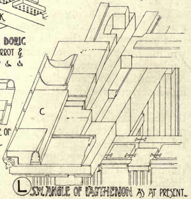
SOUTH WEST ANGLE OF PARTHENON
