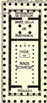
H PARTHENON ATHENS, COMPLETED B.C. 435 PERIPTERAL OCTASTYLE.
