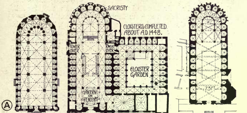
A ST. MARIA DEL MAR, BARCELONA A.D. 1328-1383. TWO OCTAGONAL PINNACLES AT WESTERN END.
