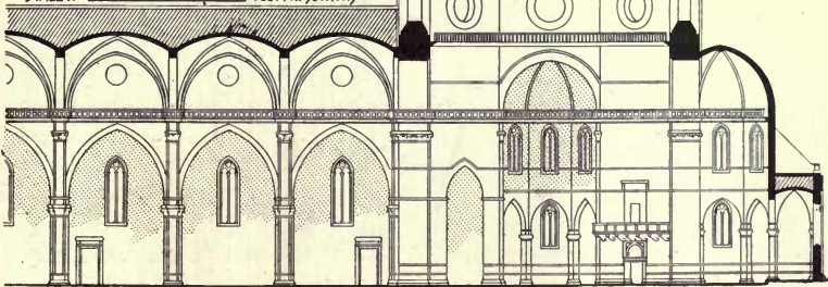
PART LONGITUDINAL SECTION (E)
