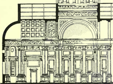
(F) PART LONGITUDINAL SECTION
