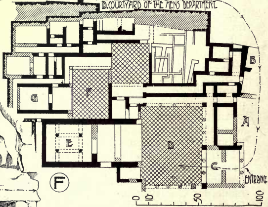
ACROPOLIS AT TIRYNS. PORTION OF THE UPPER (SOUTH) CASTLE, DESTROYED B.C. 463. ITS WALLS OF CYCLOPEAN MASONRY COMPOSED OF BLOCKS OF STONE 6 TO 10 FEET LONG & 3 FEET WIDE.
