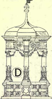
WELL HEAD 1519, OBER-EHNHEIM SCALE OF 0 5 FEET
