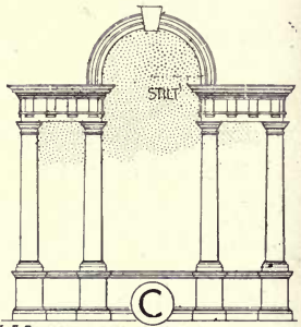
C A VENETIAN WINDOW SAID TO BE AN INVENTION OF SCAMOZZI. MUCH USED BY BROOK ADAM.
