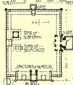
THE JUMMA-MUSJID. ALAMGIR ALI SHAH A.D. 1657-1673
