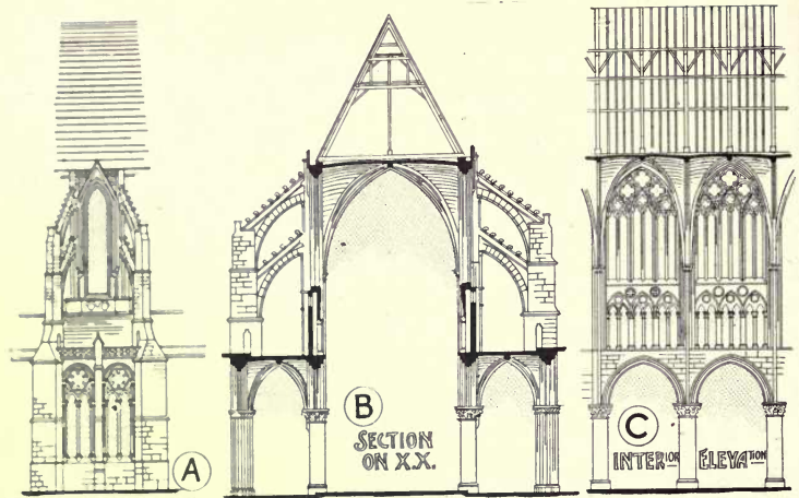
ELEVATION OF APSIDAL BAY
