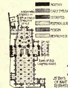
A CHRIST CHURCH DUBLIN
