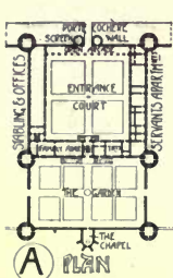
CHATEAU DE BURY NEAR BLOIS A.D. 1520.
