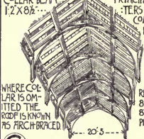
COLLAR BRACED ROOF. ST MARY MAGDALEN, PULHAM, NORFOLK THIS ROOF IS A SIMPLIFICATION OF HAMMER BEAM
