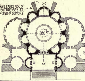
(A) PLAN A DECAGON SUPPORTING A CIRCULAR DOME WITH EARLY FORM OF PENDENTIVES.
