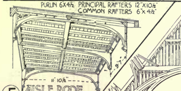
(F) AISE ROOF IXWORTH CHURCH...
