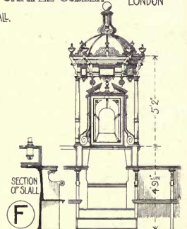
F SECTION OF SALL THRONES & STALLS, CONVOCATION ROOM, OXFORD.
