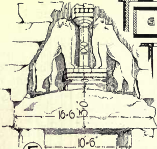
THE GATE OF LIONS MYCENÆ.
