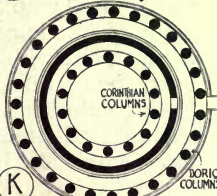
K THOLOS OF POLYCLEITOS, EPIDAUROS, 4 TH C B B.C.
