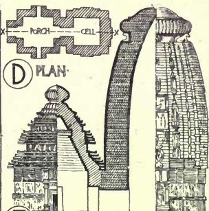
PLAN. E HALF ELEVATION AND SECTION OF BLACK PAGODA AT KANANUG IN ORISSA. AFTER FERGUSSON. TYPICAL EXAMPLE SHOWING CONSTRUCTION OF HINDOO TEMPLES. THE CELL IS INVARIABLY A SQUARE ON PLAN AND ITS POSITION INDICATED EXTERNALLY BY A TOWER OR SIKRA BENDING INWARDS TOWARDS THE SUMMIT AND SURMOUNTED BY AN AMALAKA.
