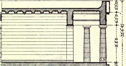
D HALF LONG. SECTION & AMBULATORY
