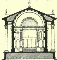
(F) TEMPLE OF JUPITER SECTION
