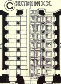
H ENLARGED PLAN PLOGGIA 0 50 100
