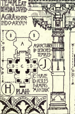
TEMPLE AT INDRAPRASTHA AGRA AD. 692. INDO-ARYAN. GREAT TEMPLE BALLUR AD. 11th. CHALUKYAN.
