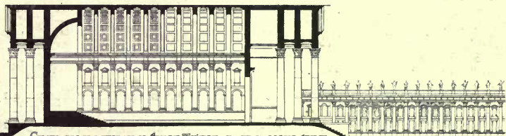
(C) SECTION Y-Y THROUGH GREAT TEMPLE & PORTION MAIN COURT
