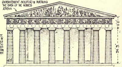
(D) EAST FACADE (RESTORED AFTER STUART)
