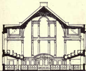
C CROSS SECTION (LOOKING EAST)
