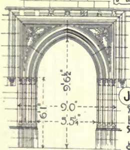
(J) MERTON COLLEGE CHAPEL-OXFORD
