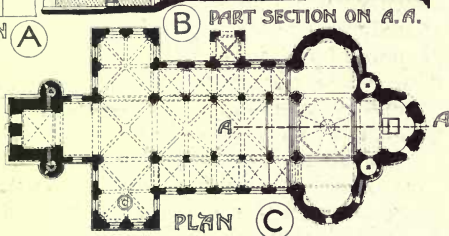
PLAN (C)
