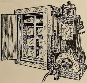
Ice-machine.
