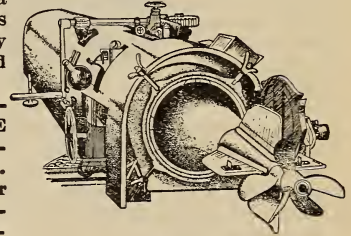
Torpedo-tube.
