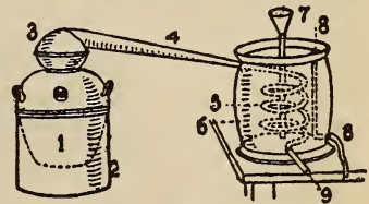
Still.
