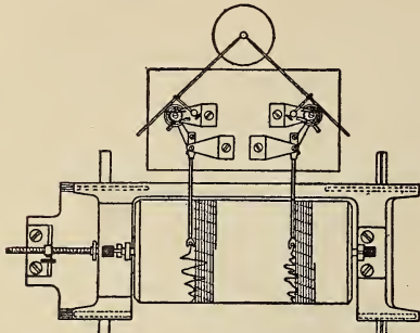
Diagrammatic View of Universal Seismograph.
