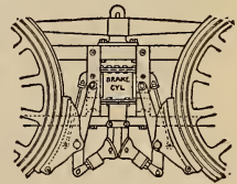
Air Brake.
