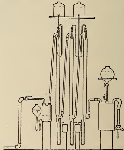
Hydrogen Generator.
