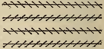
Zoellner's Pattern.
