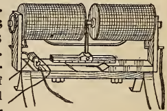
Magneto-optic rotation.
