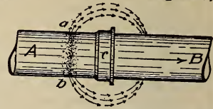
Electromagnet.
