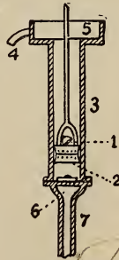
1. Plunger-valve. 2. Plunger-piston. 3. Barrel. 4. Spout. 5. Head. 6. Lower valve. 7. Induction pipe.
