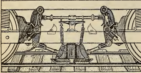
Electro-Magnetic Brake.
