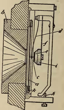
Blake Transmitter.
