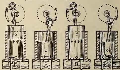
1. Suction. 2. Compression. 3. Explosion—Expansion. 4. Exhaust.
