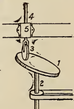
Swash-plate. 1. Swash-plate. 2. Axis. 3. Friction wheel. 4. Shaft. 5. Guide.
