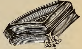
Cusp.
