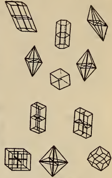
Crystals.
