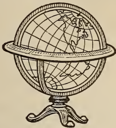
Terrestrial Globe.
