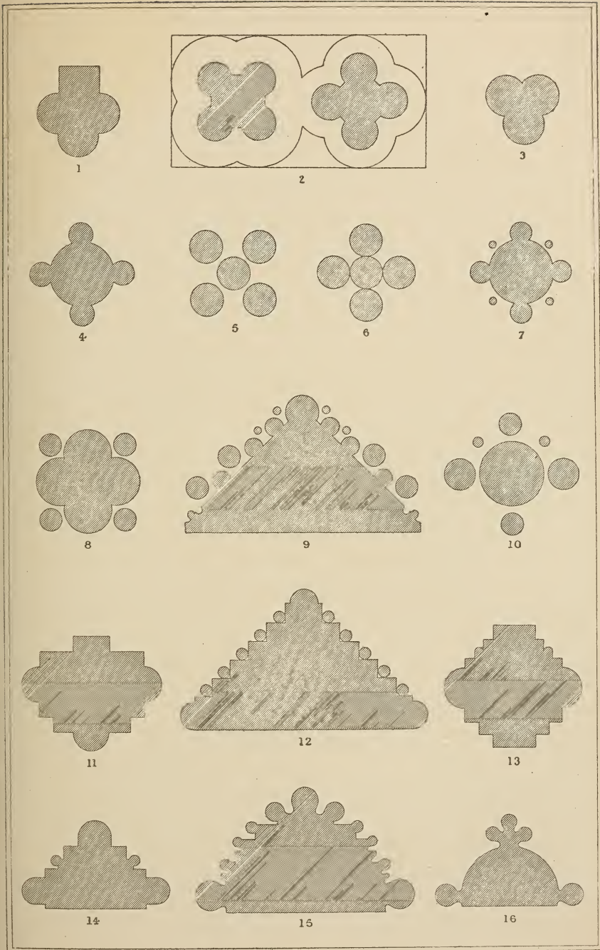
Plans of Piers.
