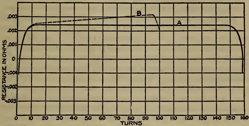
FIG. 3.—Distribution of effective alternating-current resistance. Diameter of coil, 30.4 cm.; frequency, 3,000 cycles. No. 4 bare copper wire. Spacing 6 mm.
