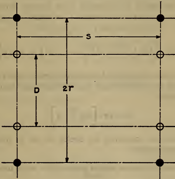
FIG. 4.—Cross section of coaxial circles and return circuits.
