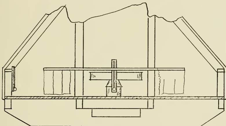
FIG. 76.—Sketch showing location of thermometer and method of hinging the hover.
