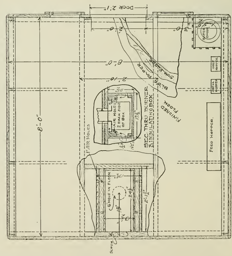
FLOOR PLAN - FIG. 1
