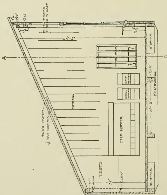
SECTION THROUGH HOUSE
