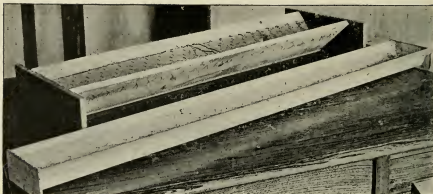
FIG. 112.—Two feed-troughs for chickens, one made of galvanized iron eaves-drip trough, the other a simple V-shaped wooden trough. Each is covered with a \frac{3}{4} -inch mesh chicken-wire. ♀
