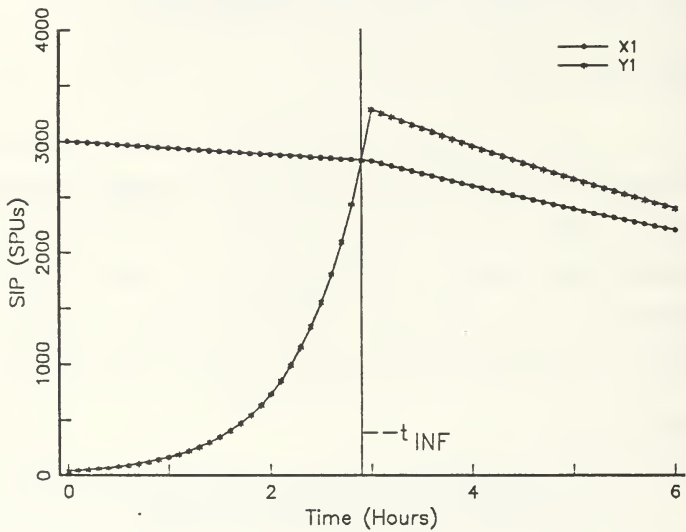
Y1 and X1 SIP Curves--General Case Example
