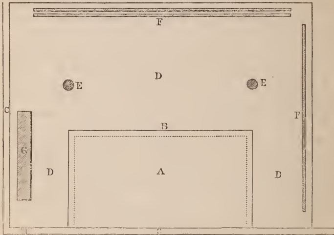
Plan of Ground for Charring Peat.
