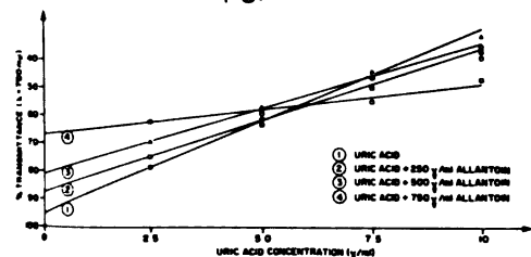
Figure 1. Influence of allantoin on the colorimetric determination of uric acid as used by the method of Archibald (1957).
