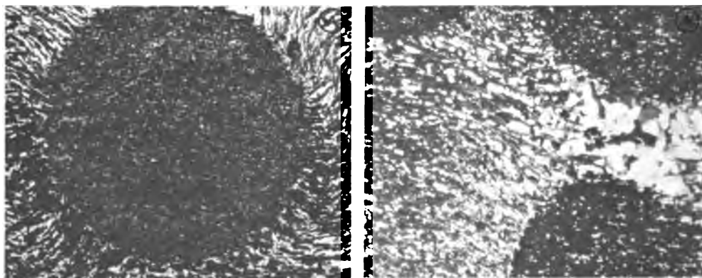
Figure 2. Magnification (X13), crossed nicols : a) Rotated perfectly spherical garnet (spessartite) crystal in a schistose matrix of quartz, feldspars, sericite, muscovite, biotite, graphite and occasional argillaceous material. The garnet contains numerous small inclusions of quartz and micas ; the orientation of the shreds in the groundmass allows one to infer the application on the tangential forces on this rock type. b) Concentration and recrystallization of quartz grains in the zone of relatively higher pressure occupying the restricted space between two adjacent spheroidal garnets.
