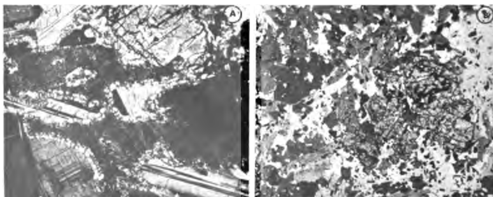
Figure 3. Magnification (X32), single nicol : a) Well developed corona structure at the interface of twinned (Carlsbad and Periclase) and occasionally zoned plagioclase and olivine. The corona is made up of hypersthene, hornblende and some biotite in this relatively fresh olivine gabbro. The plagioclase and olivine do not show corona structures when they are in contact with early magmatic augite crystals. b) Sponge garnet in a typical quartz-garnet-hornblende gneiss (amphibolitized olivine gabbro). The groundmass is composed of quartz, feldspars, amphiboles, biotite, chlorite, little magnetite, ilmenite, some pyroxenes and relicts of olivine. The garnets sometimes occupy the space of ancient coronites.
