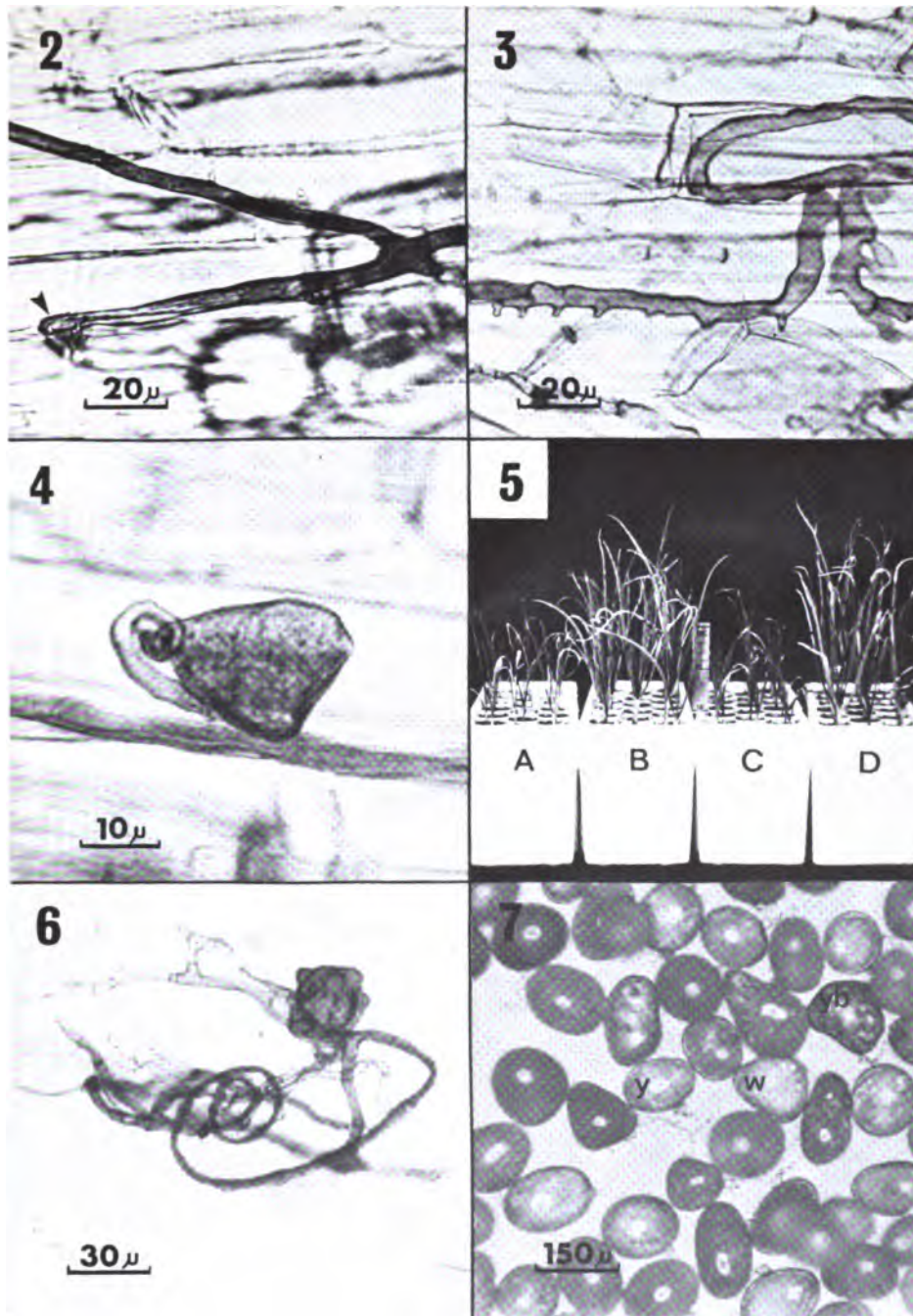
Figure 2. Hypha of Endogone calospora showing an appressorium. Figure 3. Intramatricial celium of Endogone calospora showing the comb-like hyphae. Figure 4. Intramatricial vesicle formed by Endogone calospora , showing the helial suspensor. Figure 5. Onion plants grown in styroblocks. A. inoculated control grown at 16/21°C (17 weeks). B. Inoculated plants, grown at 16/21°C (17 weeks). C. inoculated plants grown at 11/16°C (14 weeks). D. Inoculated plants grown at 21/26°C (14 weeks). Figure 6. Intramatricial vesicle of Endogone calospora . Figure 7. Spores of Endogone calospora produced on onions. W = white (young), Y = yellow, YB = yellow brown (mature).
