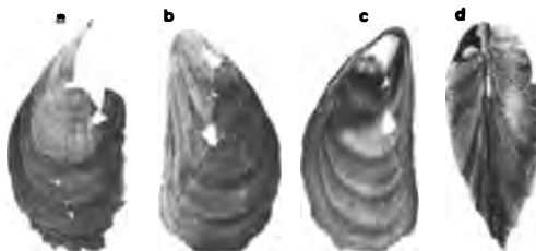
Figure 2. Views of 5 cm-long example of Mytilus edulis L. from Coburg Island, N.W.T. Hypotype, GSC No. 32086; GSC negative No. 201645; coll. W. Blake, Jr., 1970. Fig. 2a, exterior of right valve; Fig. 2b, exterior of left valve; Fig. 2c, interior of left valve; Fig. 2d, dorsal margin of both valves.
