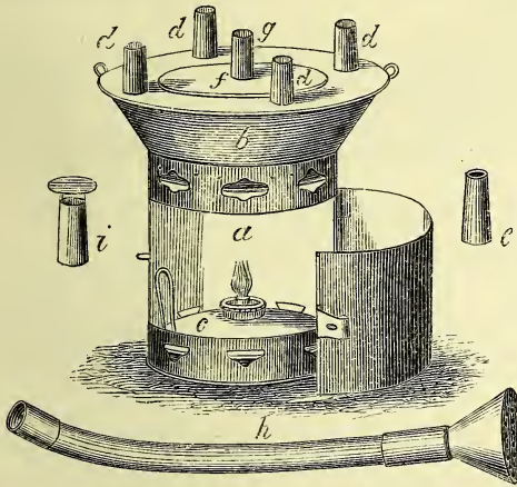
Culverwell's Portable Domestic Vapour Bath.
