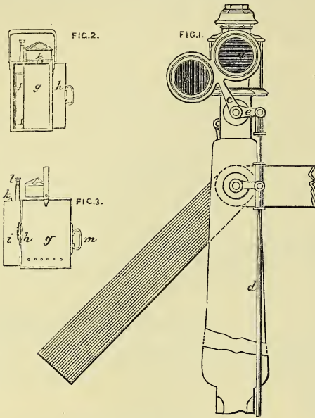
Boake's Irish Railway Signal Post.
