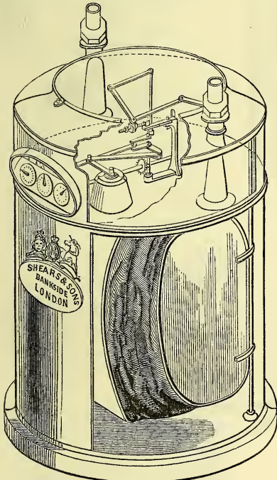
Shears & Son's Patent Dry Gas-meter.
