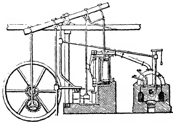
CONDENSING STEAM-ENGINE.
