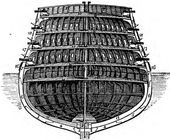
MIDSHIP SECTION.
