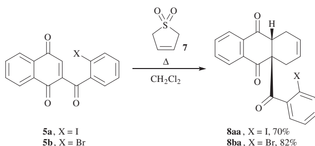
Scheme 3. DA model reaction with 3-sulfolene 7 and naphthoquinones 5a and 5b resulting in hydroanthraquinone derivatives 8aa and 8ba .
