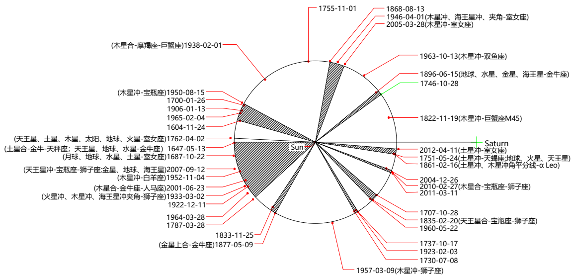
Fig.7.2 The distribution of the earth between the sun and Saturn during a major earthquake
