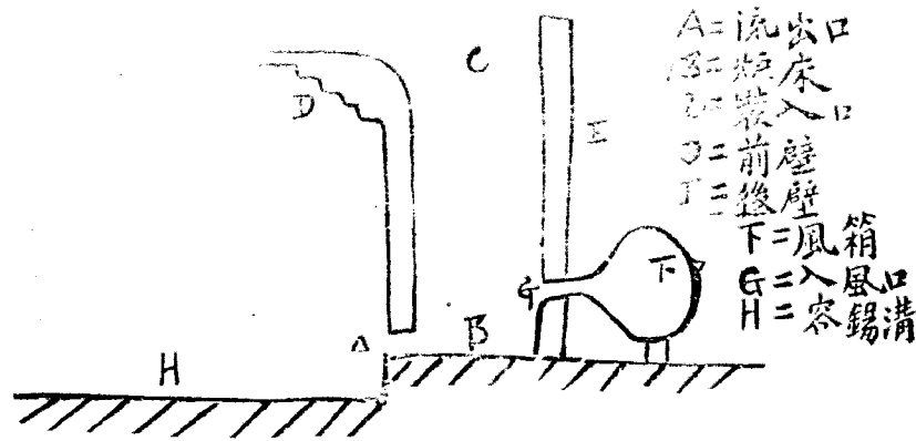
(爐之側面圖)
