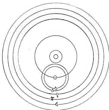
FIG. 11.—Egyptian system.
