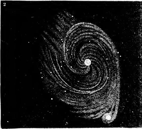
FIG. 80.—Lord Rosse's drawing of the spiral nebula in Caves Venatici , with the stub marks of the draughtsman unduly emphasised into features by the engraver.
