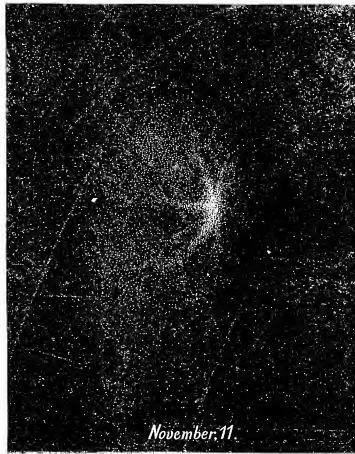
FIG. 103.—Encke's comet.
