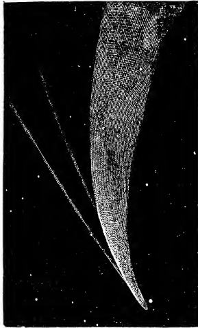
FIG. 101.—Head of Donati's comet of 1858.
