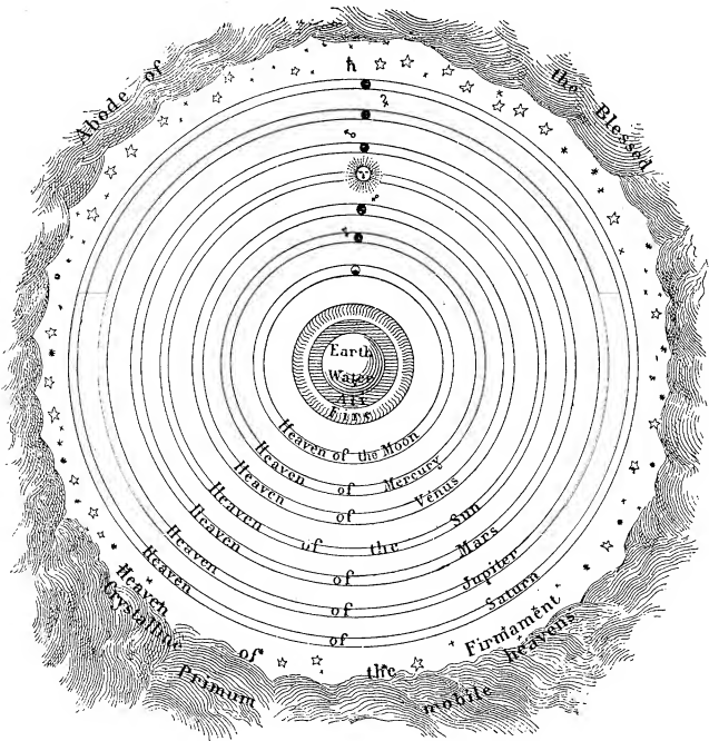
FIG. 8.—Ptolemaic system.
