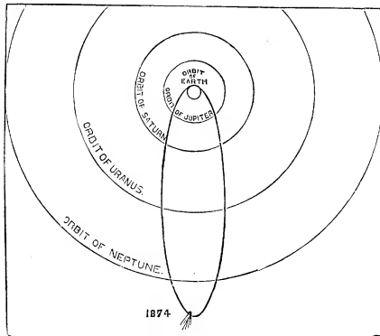
FIG. 99.—Orbit of Halley's comet.
