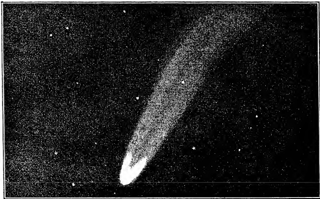
FIG. 102.—Halley's Comet.
