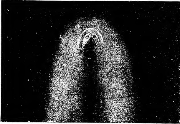
FIG. 83.—Old drawing of the Andromeda nebula.
