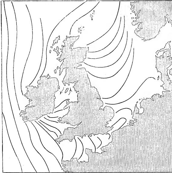
FIG. 109.—Co-tidal lines.
