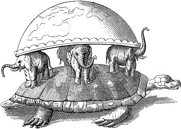
FIG. 6. —Hindoo Earth.
