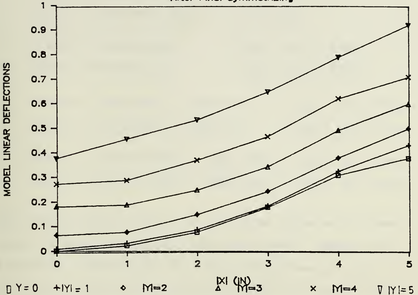
Figure 5.3.1-5: Model Deflections After Final Symmetrizing
