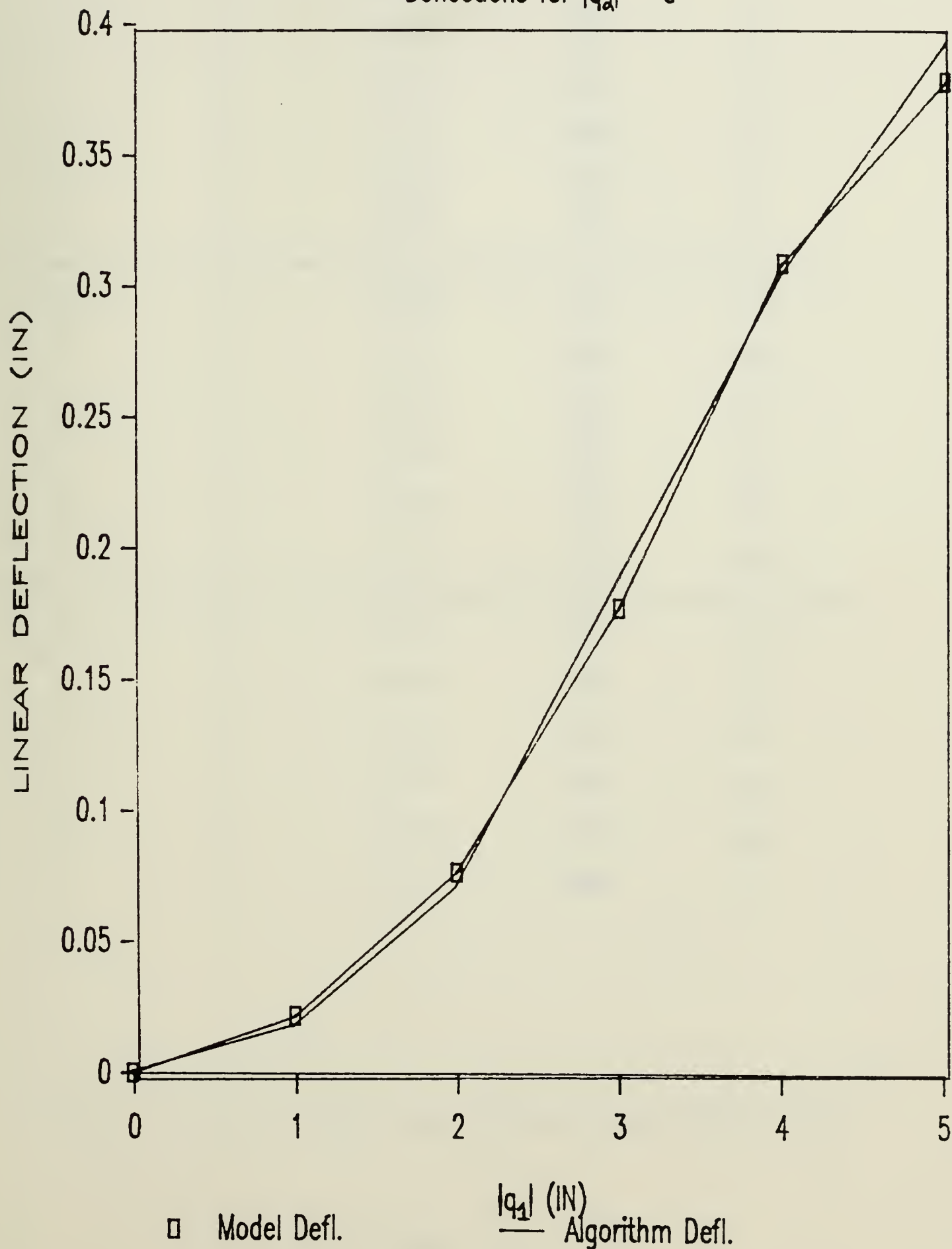
Figure 5.3.1-6: Model and Algorithm
