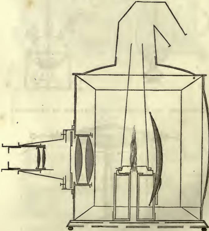
Optics. — IMPROVED MAGIC LANTERN. Fig. 17. — No. 27.
