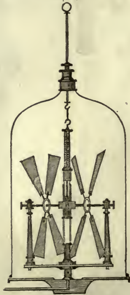
VANE AND MILL IN VACUO Fig. 79.
