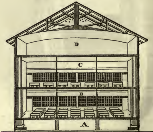
Fig. 2. Transverse Section.
