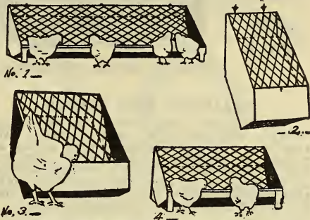
Boston Food Hoppers.
