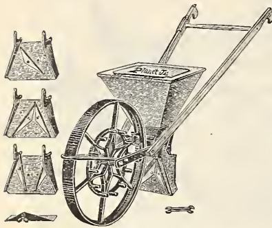
20-D Fertilizer Drill
