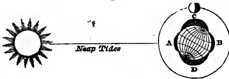
NEAP-TIDE.
