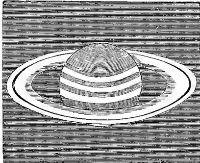
SATURN.
