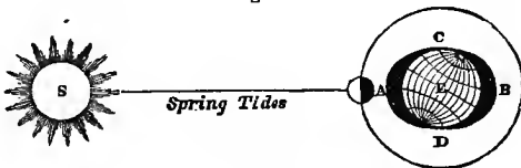
SPRING TIDE.
