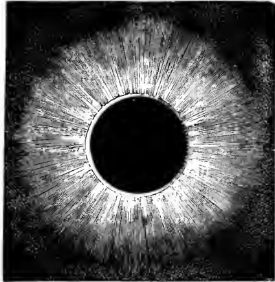
ANNULAR ECLIPSE OF 1836 SHOWING BAILEY'S BEADS.
