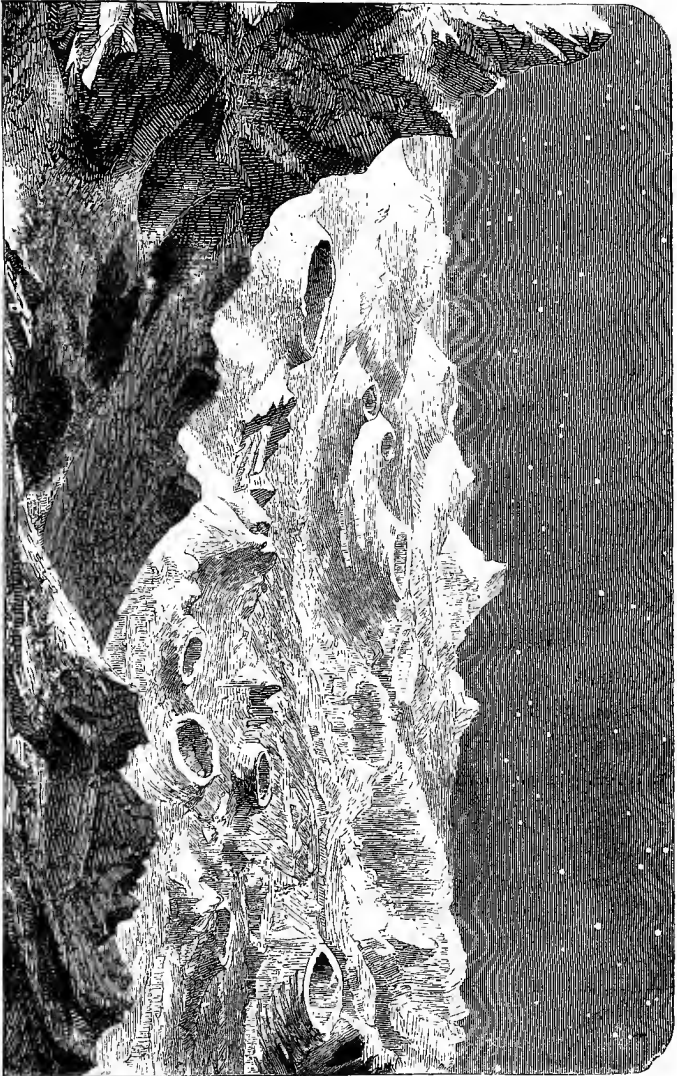
IDEAL LANDSCAPE OF THE MOON.
