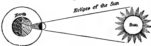
ECLIPSE OF SUN.
