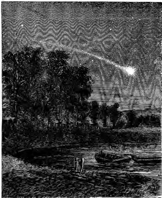
A METEOR WITH ITS TRAIN.
