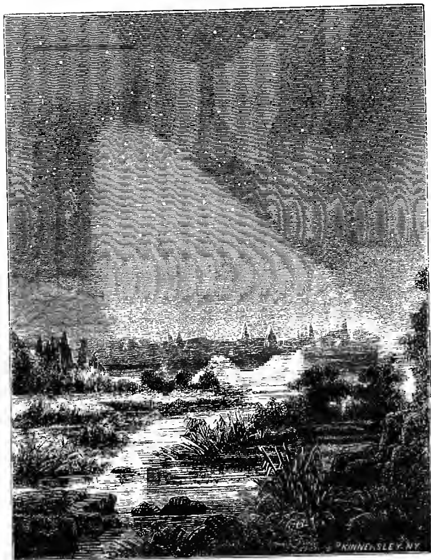
ZODIACAL LIGHT.
