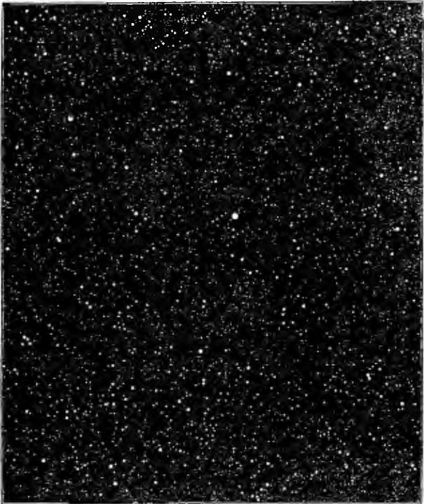
A PART OF THE CONSTELLATION OF THE TWINS.
