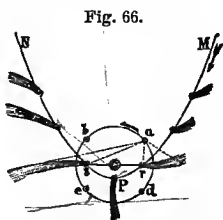
ORBIT OF COMET.
