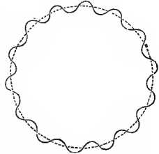
PATH OF THE NORTH POLE IN THE HEAVENS.
