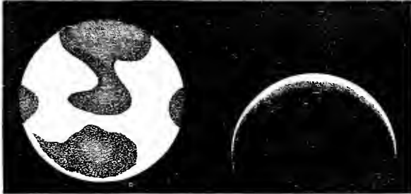
CRESCENT AND SPOTS OF VENUS.
