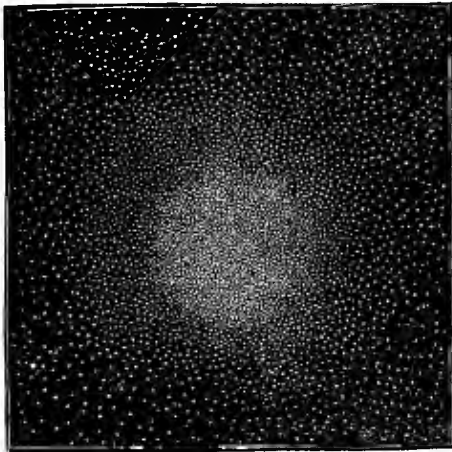
STAR-CLUSTER IN TOUCAN.
