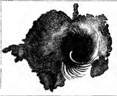
CYCLONE.
