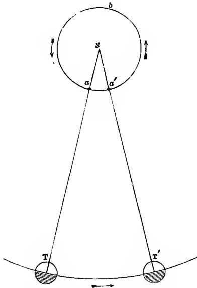
SYNODIC AND SIDEREAL REVOLUTION.
