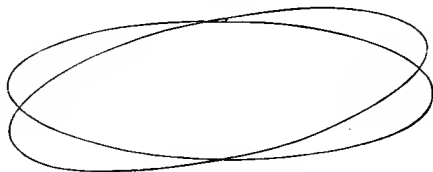
PLANETARY ORBITS.
