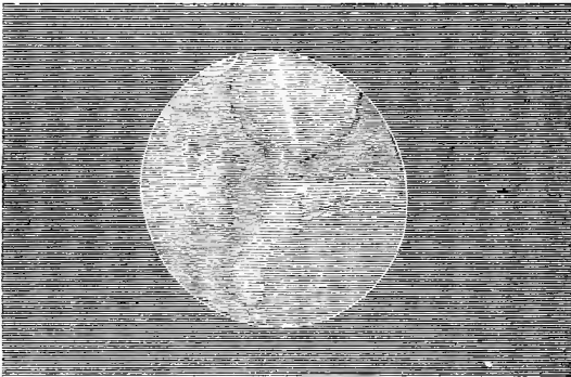
VIEW OF MARS.
