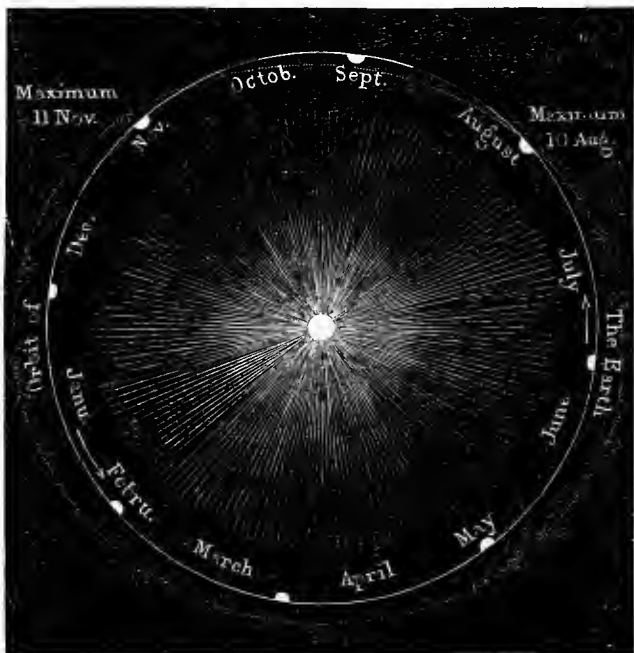
METEORIC RING.
