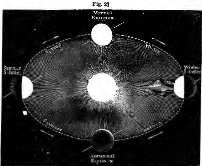
ORBIT AND SEASONS OF MERCURY.
