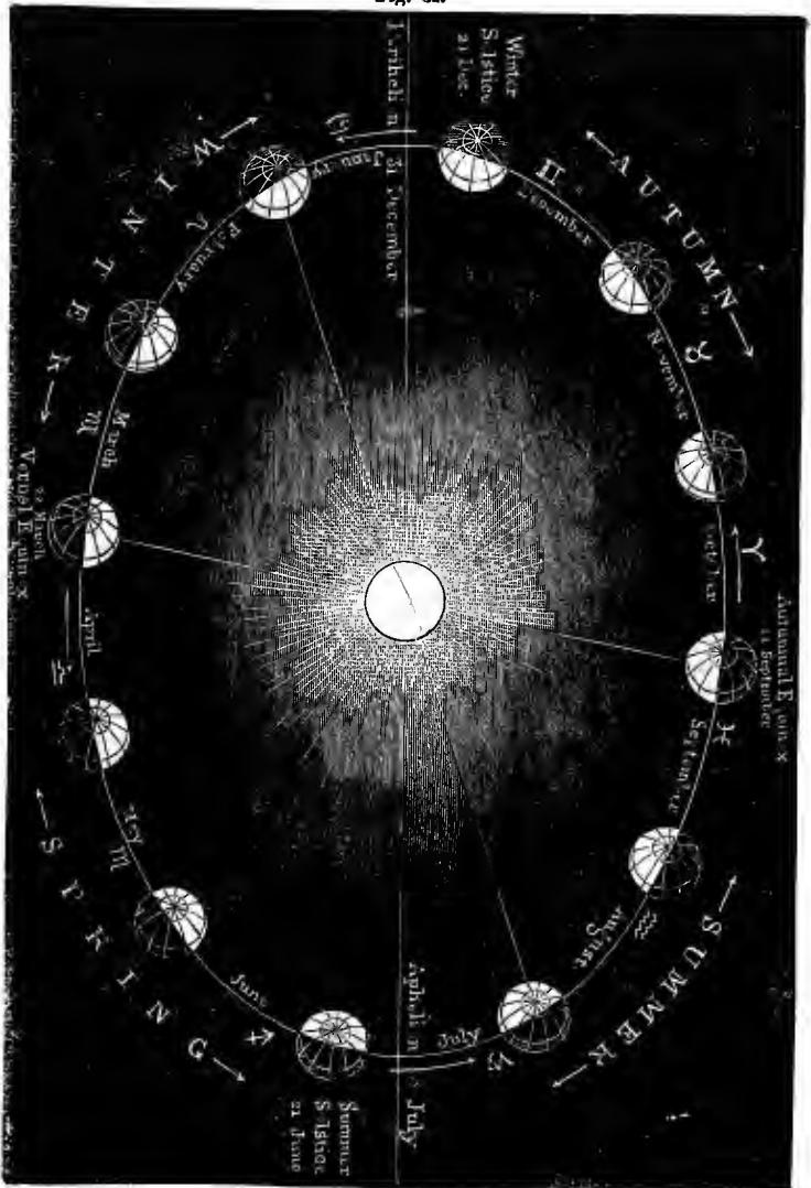
THE ORBIT OF THE EARTH.
