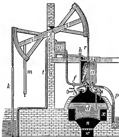
FIG. 157. NEWCOMEN'S STEAM ENGINE
