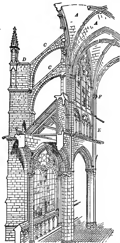
FIG. 58. CROSS SECTION OF AMIENS CATHEDRAL
