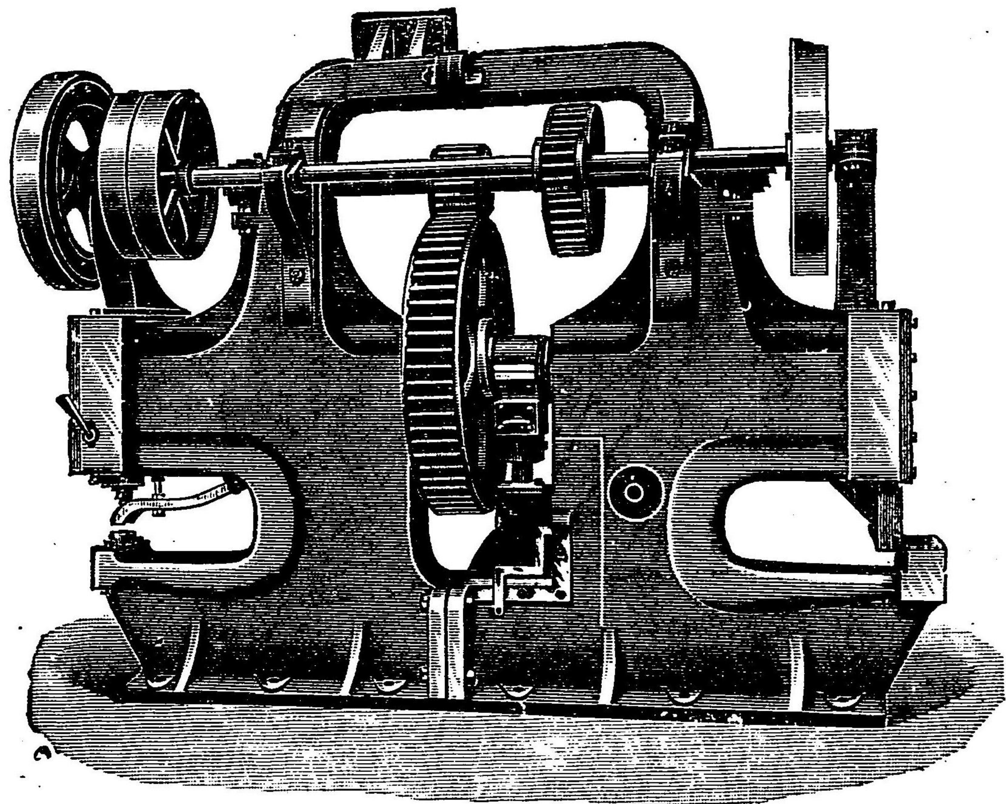
Punching Shearing & Angle-iron Cutting Machine.
