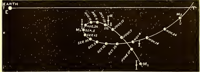
FIG. 2. ONE OF MARS'S LOOPS.
