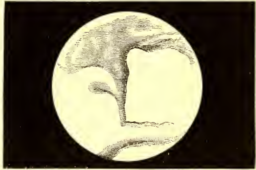
APPEARANCE OF MARS, 1852, FEBRUARY 3, 6 H. 50 M., Greenwich Mean Time. Power of Telescope, 242 and 358 on 6 1-3 inch object-glass.
