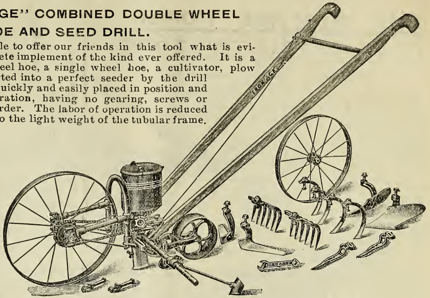
The "Iron Age" Combined Double Wheel Hoe and Seed Drill $10.50.
