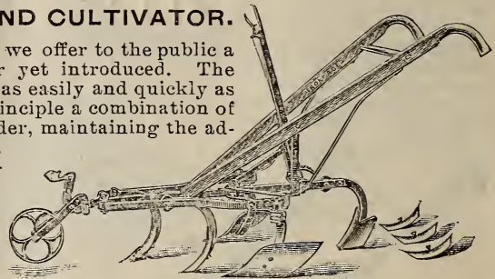
THE "IRON AGE" NO. 6, WITH LEVER AND PLAIN WHEEL. PRICE $7.25
