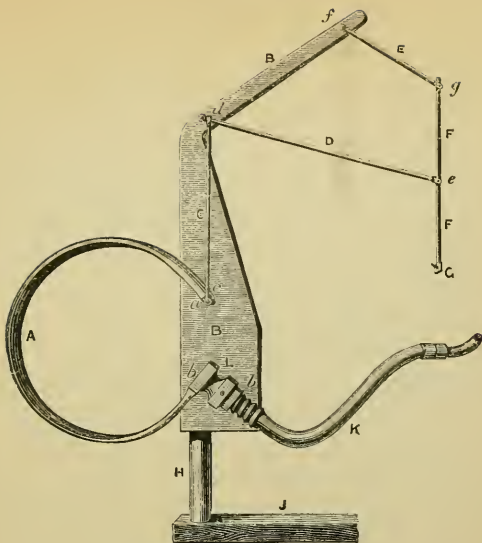
FIG. 205.—Fick's spring kymograph. A. C-spring. BE. Support. C. Rod which communicates the movements of the spring to the lever D, and thus to the writing-needle G. K. Leaden tube by which the cavity of the spring is in communication with the artery.
