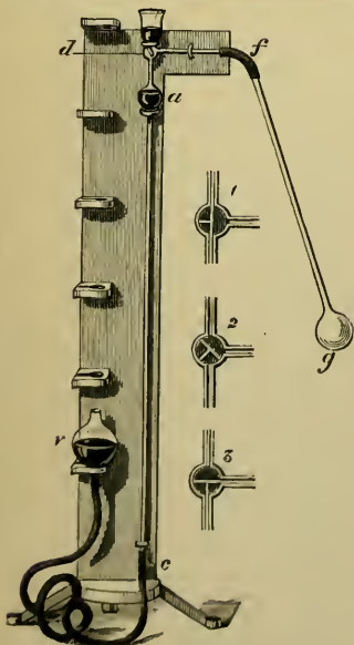
FIG. 197.—Alvergniat's mercurial pump (§ 25).
