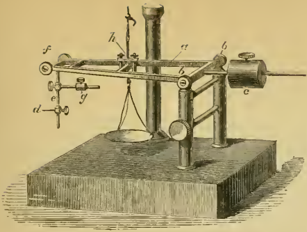
FIG. 269.—Myographion of Pflüger. The moist chamber, which is supported by the large pillar, and from which the thread h descends, is not shown. The lever a moves freely on the two pillars bb . At f the rod e , bearing the movable style d , with its movable counterpoise g , swings easily. At the opposite end of the lever is the heavy counterpoise c . The milled head on the side of one of the pillars b rotates the lower of the two bars connecting b and b . A silk thread is carried from e to this bar. By turning the milled head the style may thus be allowed to fall upon or remove away from the recording surface as desired.
