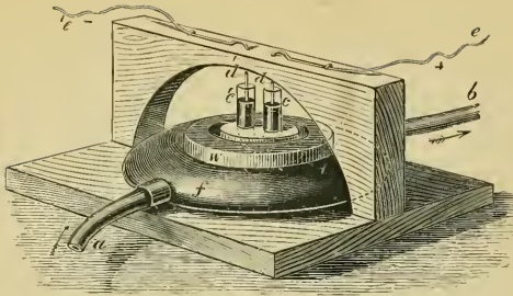
FIG. 223.—Mercurial breaker for artificial respiration (§ 49).
