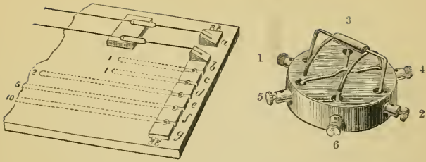
FIG. 293.—The Rheochord. The diagram represents the end of the board on which the resistance wires are stretched. a, b, c, d, e, f, g, are brass blocks which would, if it were not for the wires, be insulated. From the block b a german silver wire (the course of which is indicated by the dotted line), after turning round an ivory pin at 1 , returns to c . From c a similar wire of exactly the same length returns to d . From d a wire three times the length returns to e ; e and f are connected by a wire five times as long. From each of the blocks a and b platinum wires extend to the further end of the board, a distance of more than a metre, which are insulated at their extremities. They are, however, in metallic connection by means of a slide ("travelling mercury cups") shown in the diagram. According to the distance of the slide from a and b , which can be measured by a scale on the board, the resistance between a and b can be varied. When the slide is as far as it will go, the resistance is equal to that between b and c , or c and d . When the slide is pushed up to a b , the total resistance of the rheochord is twenty times as great as between b and c . If plugs (not shown in the diagram) are inserted between each block and its neighbour, the resistance is nil. (See p. 347.)
