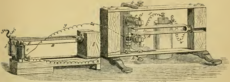
FIG. 277.—The recording tuning fork.
