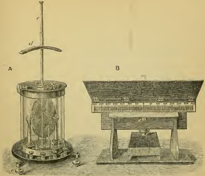
FIG. 286.—Sir W. Thomson's galvanometer and scale.
