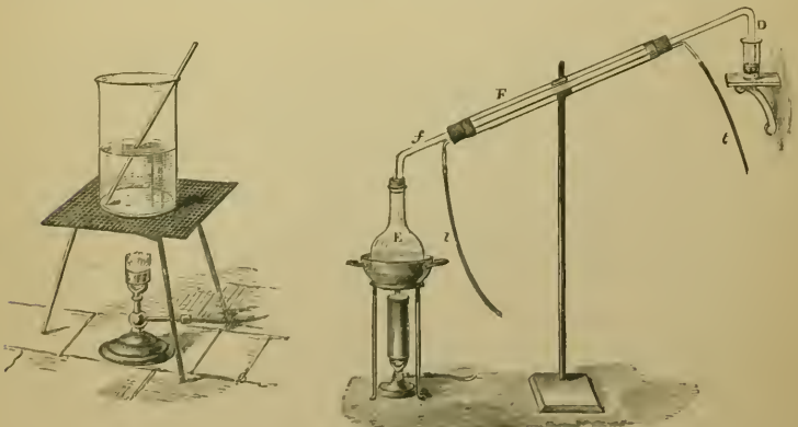
FIG. 328.—Solution. The beaker is supported on wire gauze in order to prevent it from cracking. FIG. 329.—Apparatus for preventing loss by evaporation during prolonged ebullition. E , the flask in which the liquid is boiled; F , a Liebig's condenser; f , a glass tube, which connects E and F ; t and t' , two India rubber tubes, which convey a stream of water to and from the condenser. The vapour from E is condensed in F , and runs back into E . Any of the condensed liquid that passes beyond the bend of the glass tube b , which is connected to the upper end of F , is collected in the small vessel below, D , passes to the bottom of the vessel, and as soon as any quantity of liquid accumulates in it, the flame may be removed from under E ; a vacuum then forms in E , and the liquid rushes back into it.
