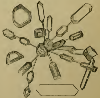
FIG. 313.—Hippuric acid.
