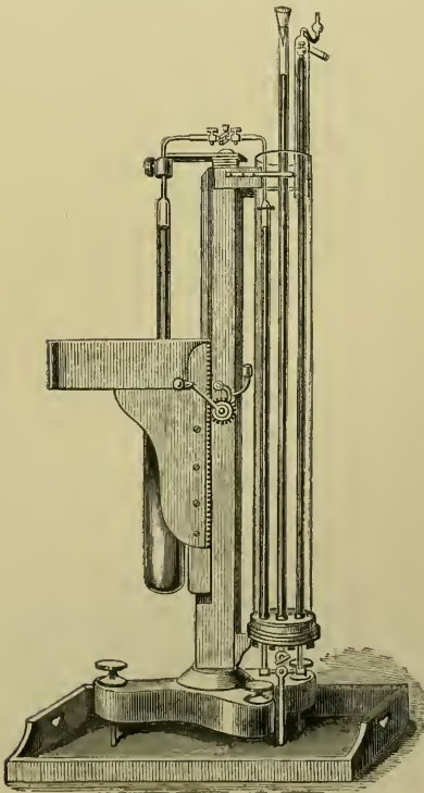
FIG. 201.—Frankland and Ward's apparatus for explosion (§ 31). (From Sutton's Volum. Analysis.)
