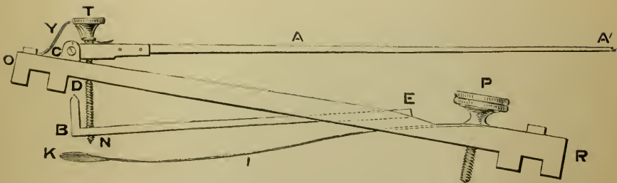
FIG. 208.—Mechanical arrangement of the sphygmograph (§ 38).
