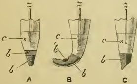
FIG. 273.—Ends of non-polarizable electrodes. A, with the clay plug b projecting beyond the glass tube; B, with the end of the glass tube closed and bent, a hole being drilled in the tube at b' , to expose the plug; C, oblique end with the clay plug flush with the glass tube.
