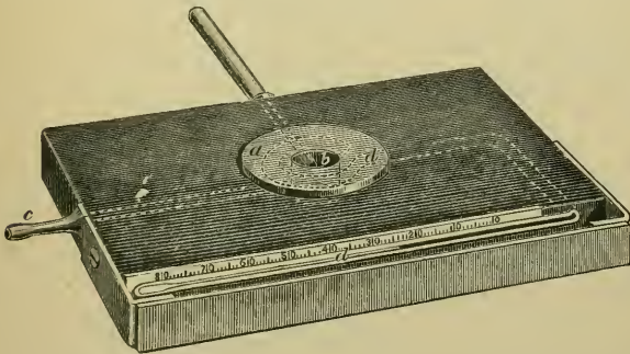
FIG. 2.—Stricker's warm stage (simple form). It consists of a block of black vulcanite about 3 inches long by 1½ wide, and ½ inch thick. The central chamber ( b ) is closed below by a glass plate, and surrounded at the top by a perforated copper dish ( a ), the orifice of which is of the same size as the chamber. The chamber is cylindrical. The cistern of the thermometer surrounds the chamber, as shown by the dotted line ( d ). Its capillary tube lies in a trough, one side of which is formed by the back of the block and the other by a metal plate screwed on to it, the form of which is shown in the figure. The tube ( c ) leads into the chamber. A second tube leads from it through the projecting metallic arm shown at the top of the figure. This arm, which is of one piece with the disk ( a ), is of such size that the rod, fig. 13, fits on to it. By means of this rod the chamber is heated in the way already explained. In experiments with gases the gas enters by c and passes out through the projecting arm. p. 14.
