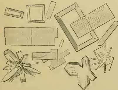
FIG. 302.—Creatinine.
