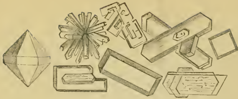
FIG. 301.—Creatine.
