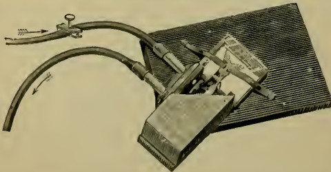
FIG. 216.—Dr. Caton's fish-trough (§ 43). It must be used with the microscope stage inclined at an angle of about 45°.
