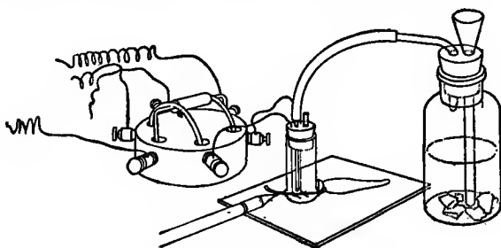
Fig. 32. The gas chamber, with hottle for generating carbon dioxide, and a pole-changer arranged to stimulate the nerve either within or without the chamber. The holes in the glass through which the nerve passes are plugged with normal saline clay.
