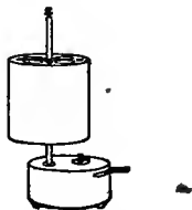
Fig. 11. The kymograph or record drum. The aluminium drum is driven by clockwork at speeds varying from one revolution per hour to eight per minute. The brass tube or sleeve on which it is held by a spring clip rests below on a disk fastened to a steel spindle which passes through the whole length of the sleeve. By turning the screw at the top the sleeve with the drum can be raised off the friction bearing. It can then be revolved rapidly by hand (spun) at a sufficiently uniform speed.
