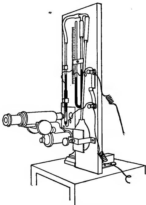
Fig. 4. The capillary electrometer.
