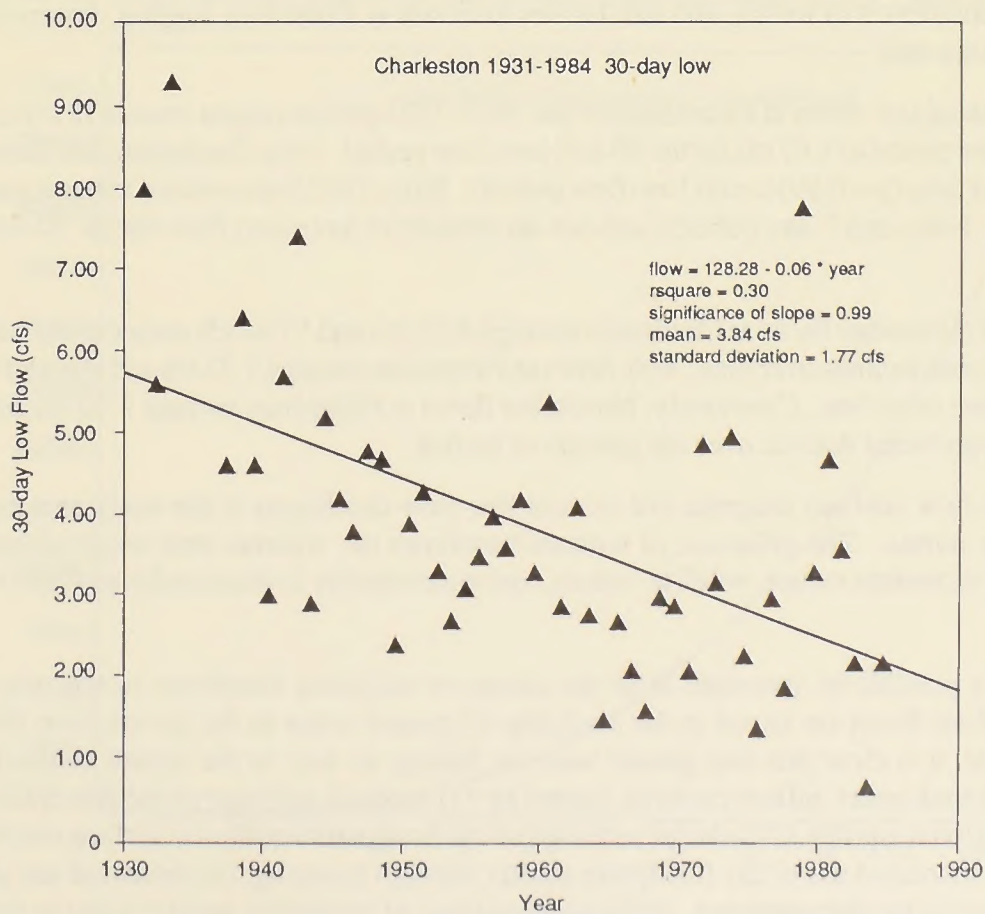
Figure 27. Trend in 30-day low flow for the San Pedro River at Charleston, 1931-1984.
