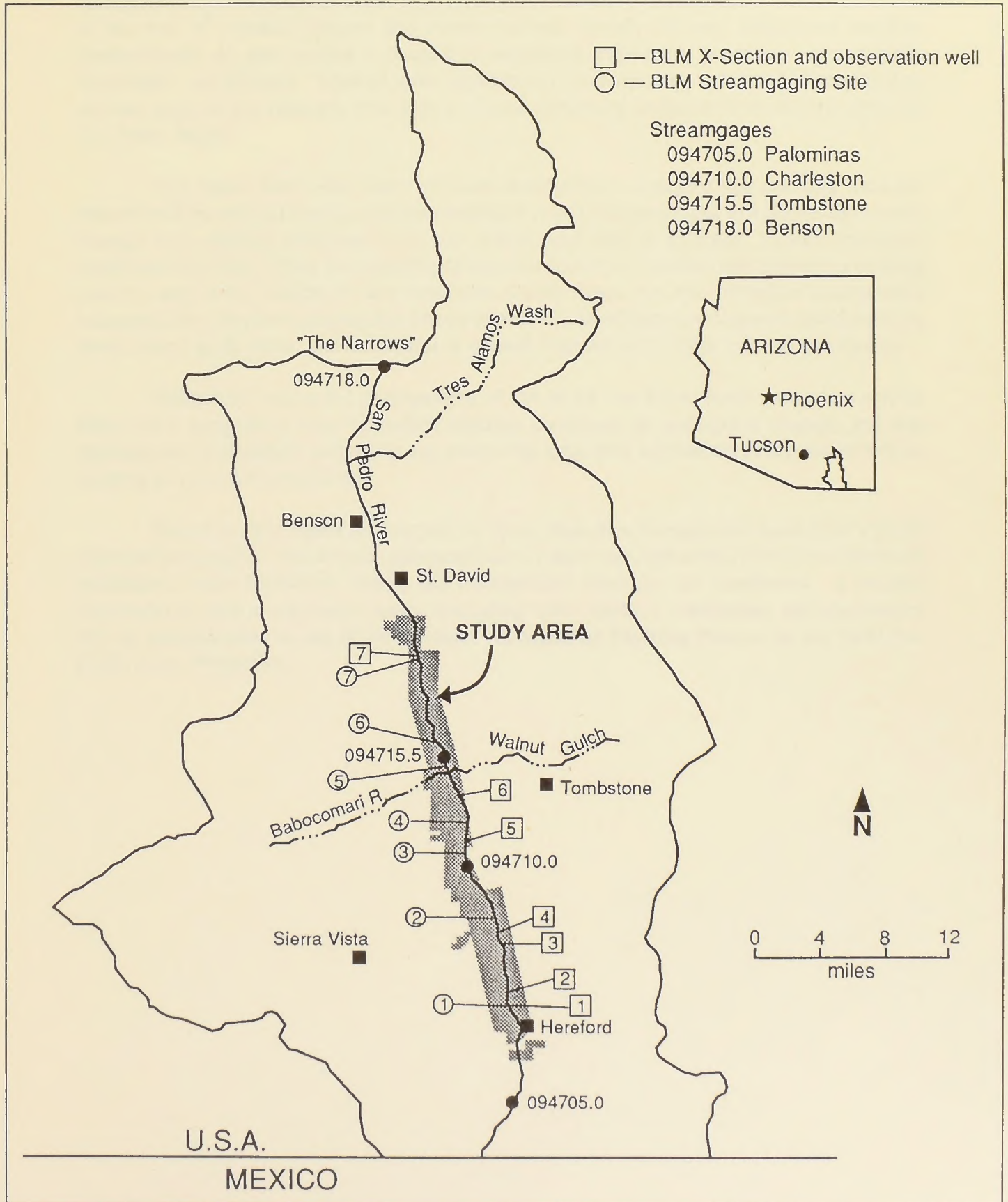
Figure 1. San Pedro River project location map.
