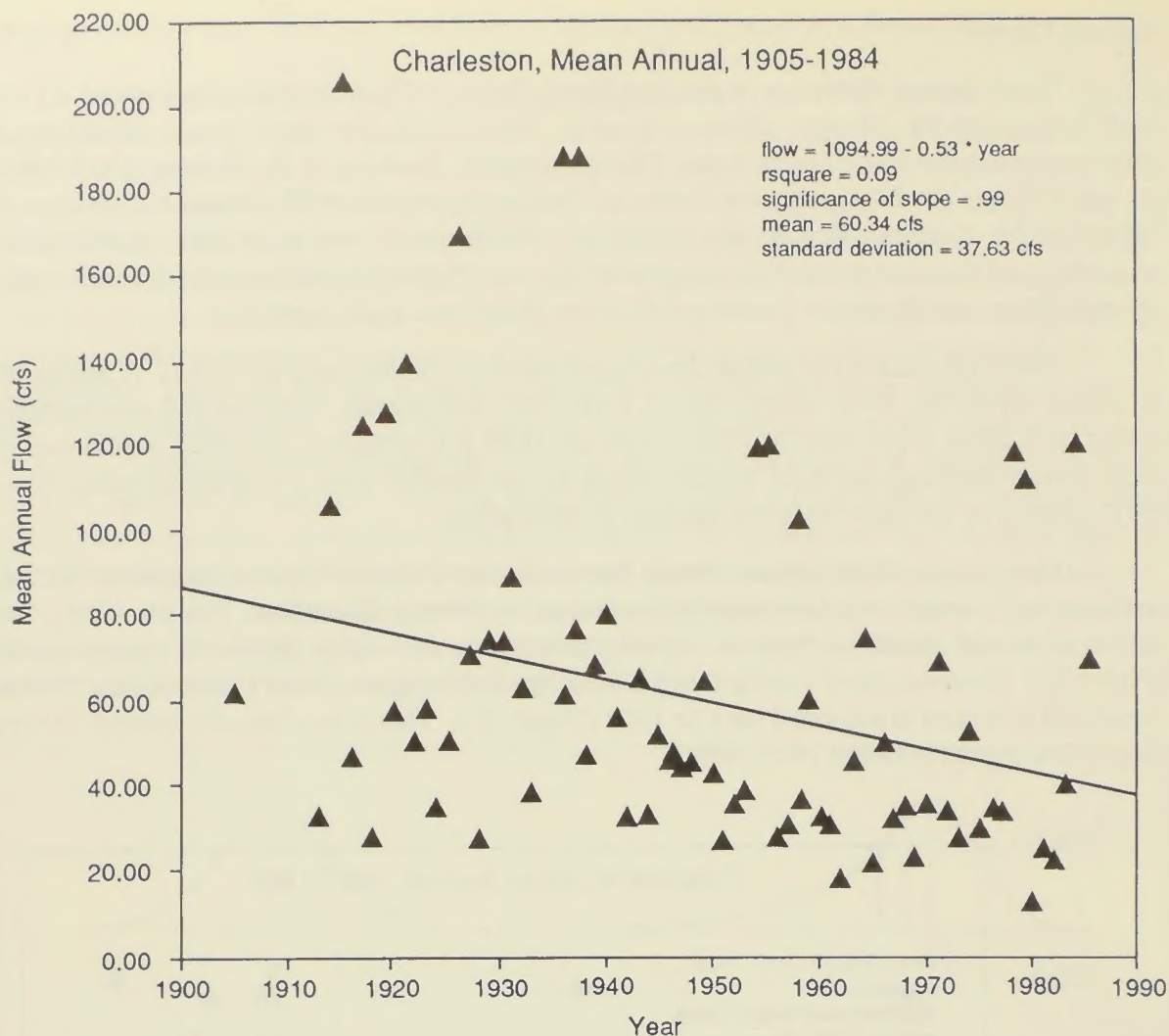
Figure 21. Trends in mean annual discharge, 1905-1984, San Pedro River at Charleston.
