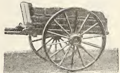
STEEL-AXLE FARM DUMP CART.
