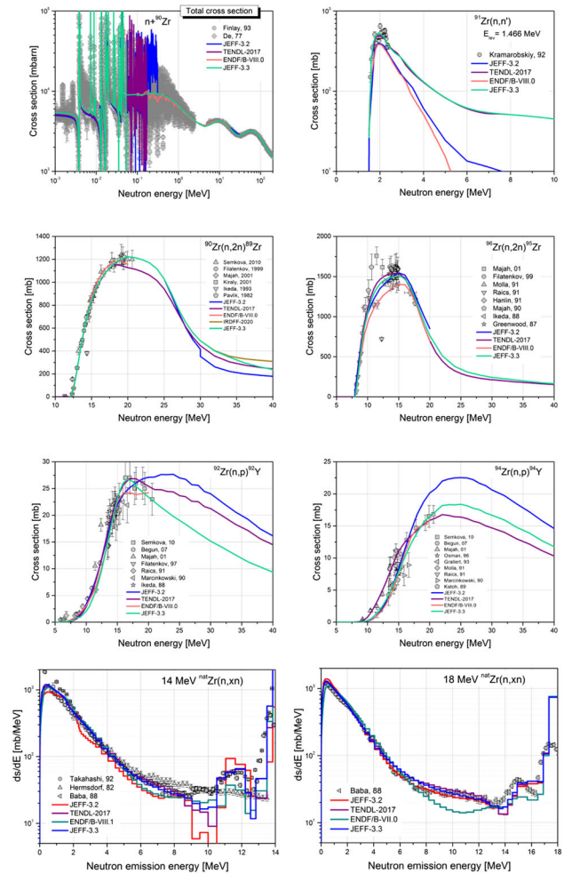
Fig. 32 Top left: evaluated total cross section for the n + {}^{90}\text{Zr} . Top right: the evaluated (n,n') cross section for the 2^{\text{nd}} excited level of the ^{91}\text{Zr} . Row 2 left: evaluated ^{90}\text{Zr}(n,2n) cross section. Row 2 right: evaluated ^{96}\text{Zr}(n,2n) cross section. Row 3 left: evaluated ^{92}\text{Zr}(n,p) cross section. Row 3 right: evaluated ^{94}\text{Zr}(n,p) cross section. Row 4 left: neutron emission spectrum for {}^{\text{nat}}\text{Zr} at 14 MeV. Row 4 right: neutron emission spectrum for {}^{\text{nat}}\text{Zr} at 18 MeV. Comparisons are with experimental data, JEFF-3.2, ENDF/B-VIII.0 and TENDL-2017 [5, 180]
