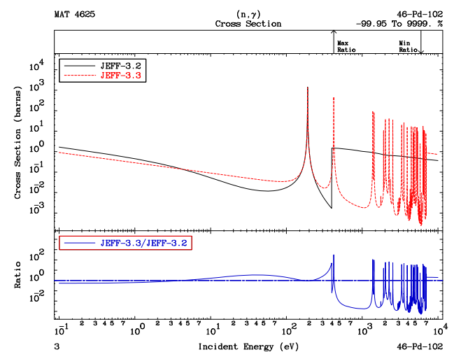
Fig. 41 Example of the new evaluated capture cross section for the ^{102}\text{Pd} stable isotope from TENDL
