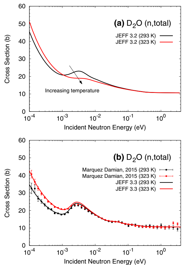
Fig. 60 Temperature dependence of the evaluated D_2O(n,tot) total cross section in the JEFF 3.2 library (a), and JEFF 3.3 library (b) compared with transmission measurements by Márquez Damián [362]
