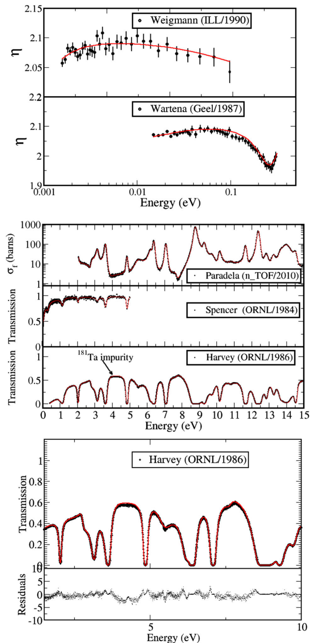
Fig. 1 Top: comparison of the experimental and calculated \eta(E) for ^{235}\text{U} in the thermal energy range. Middle: comparison of the SAMMY fit of the experimental data for ^{235}\text{U} . The bottom figure gives a flavor of typical residuals and highlights an unaccounted Ta impurity in the Harvey data. Chi-square varies between 0.94 and 1.8 over the range of the fits (see also the next figure)
