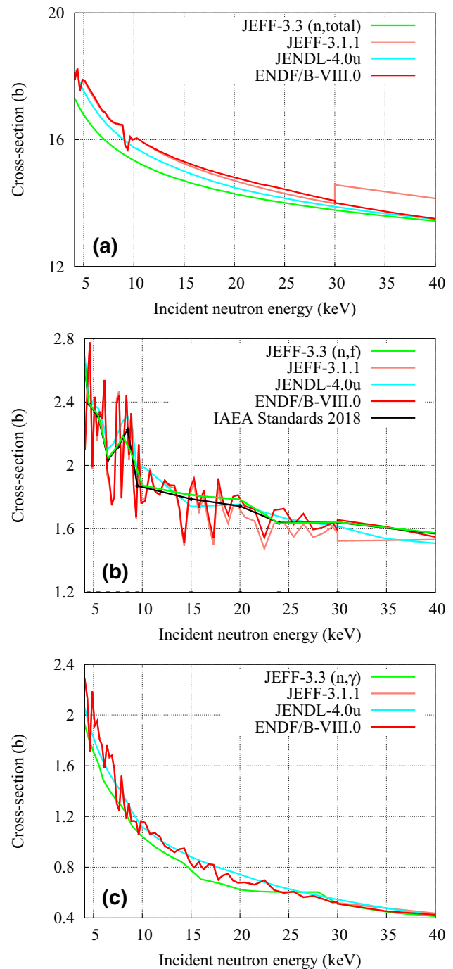
Fig. 7 Unresolved resonance range cross sections for ^{239}\text{Pu} total (a), fission (b) and capture (c), with comparisons between JEFF-3.3, JEFF-3.1.1, ENDF/B-VIII.0, JENDL-4.0u and the IAEA 2018 Standards Reference Cross Section
