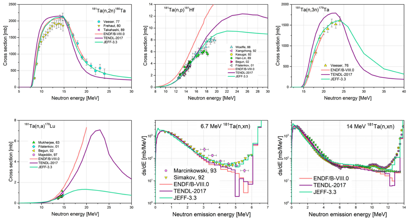
Fig. 36 Experimental data for n + {}^{181}\text{Ta} cross sections and spectra compared with the JEFF-3.3 evaluation, TENDL-2017 and ENDF/B-VIII.0. The JEFF-3.2 evaluation was adopted in JEFF-3.3. The data are from Refs. [223–235]
