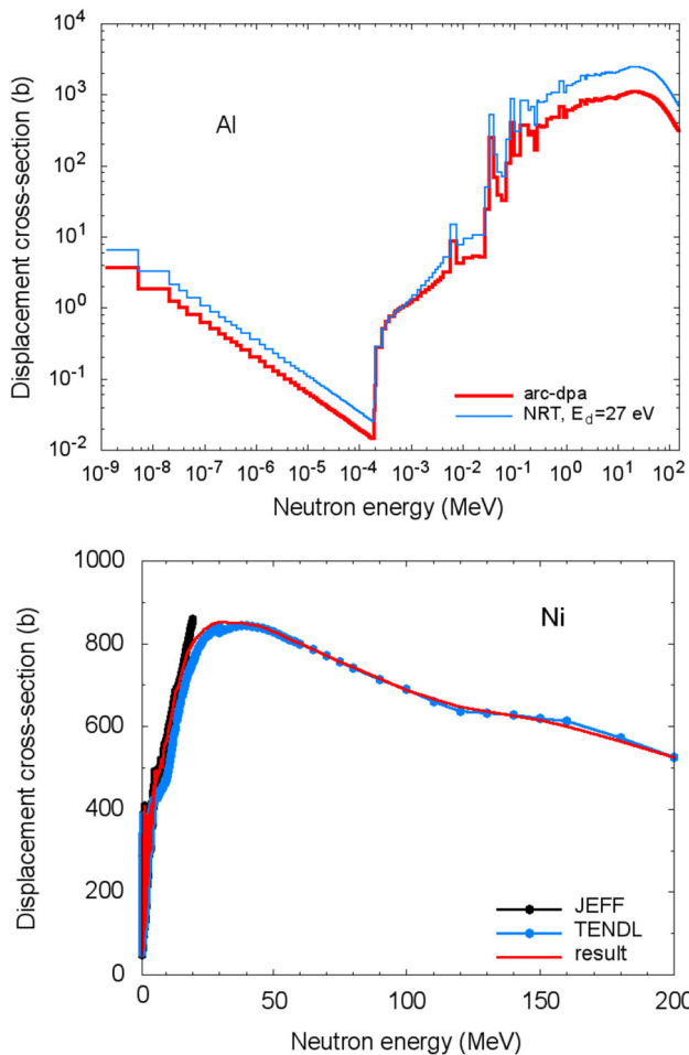
Fig. 54 Displacement cross section for aluminum calculated using the arc-dpa and NRT models (top). Displacement cross sections for nickel obtained using JEFF-3.3 and TENDL-2015 data using the arc-dpa model (bottom)
