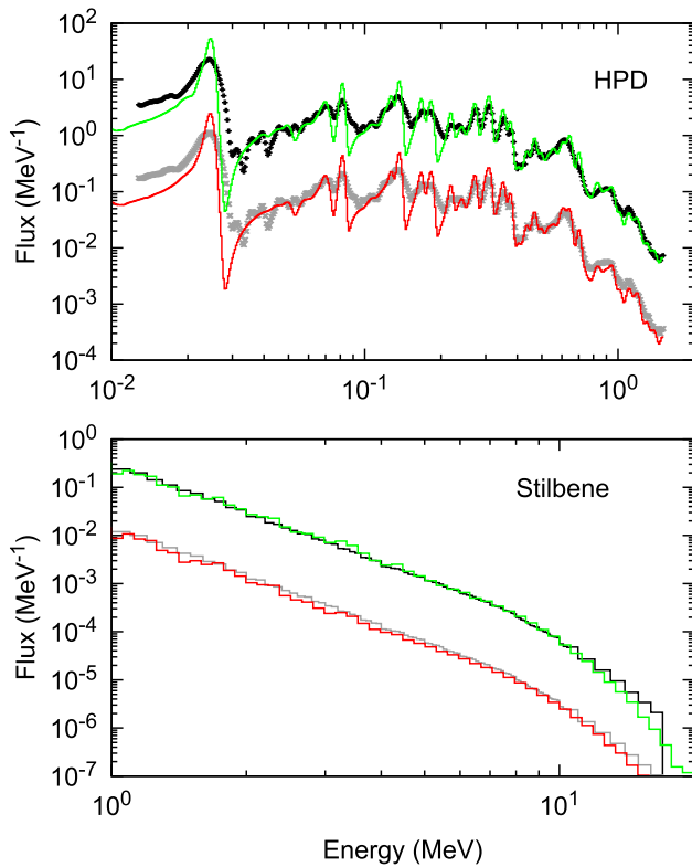
Fig. 78 Fe shielding experiment with 252 Cf at Řež. Data (black) versus JEFF-3.3 (green) and data (grey, divided by 20) versus ENDF/B-VIII.0 (red, divided by 20). The top figure shows the data for the energy range 0.01–1.3 MeV obtained with proportional counters. The iron sphere has a diameter of 100 cm and the center of the detector is at 3 cm from the surface of the sphere. The bottom figure (0.9–10 MeV) shows the data obtained with the stilbene scintillator. The sphere has a diameter of 50 cm and the center of the detector is at 100 cm from the center of the sphere
