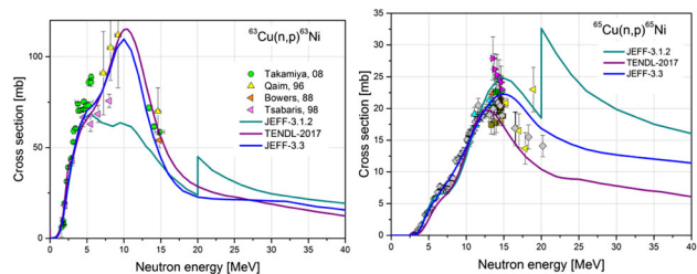
Fig. 30 Left: evaluated ^{63}\text{Cu}(n,p)^{63}\text{Ni} cross section. Right: evaluated ^{65}\text{Cu}(n,p)^{65}\text{Ni} cross section
