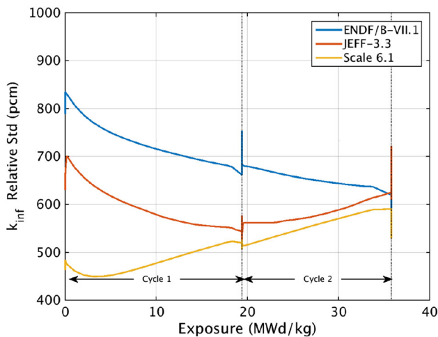
Fig. 85 Evolution of the k_{inf} relative standard deviation of a typical PWR assembly. Various covariance matrices are considered from JEFF-3.3 and other well-known libraries
