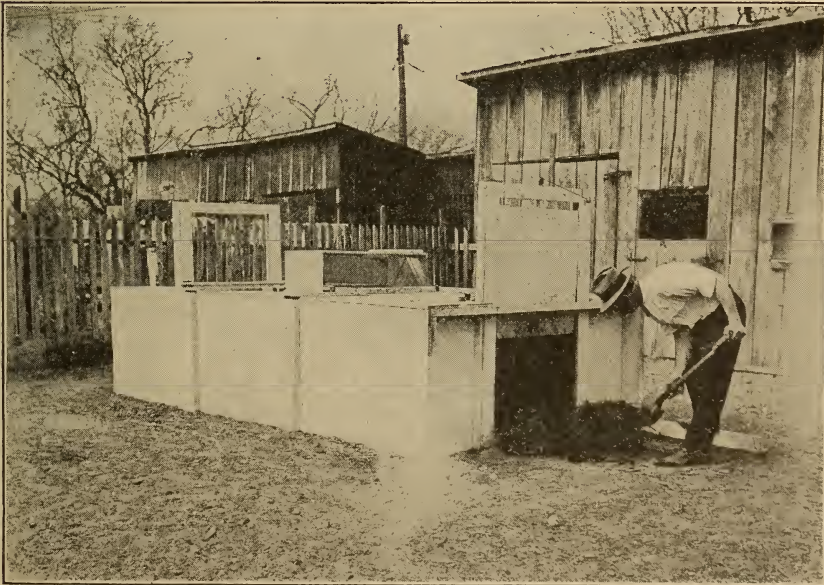
PLATE V.—Manure box with fly trap attached. (Bishopp.)
