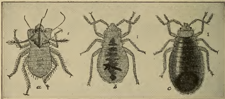
FIG. 75.—Bedbug: a , Larval skin shed at first molt; b , second larval stage immediately after emerging from a ; c , same after first meal, distended with blood. Greatly enlarged. (Marlatt.)
