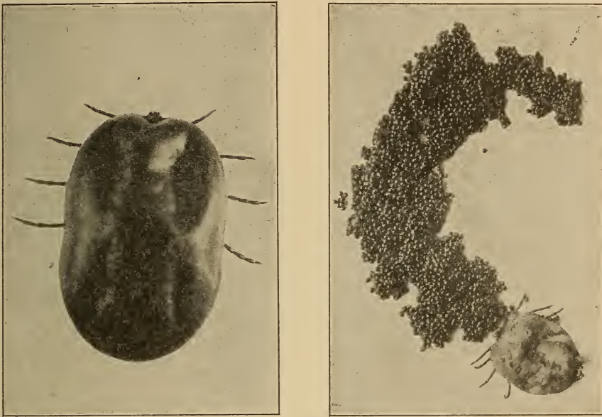
PLATE XXVII.—The cattle tick, Boophilus annulatus . Fig. 1 (Left)—Fully engorged female. Fig. 2 (Right)—Engorged female depositing eggs. (Bishopp.)
