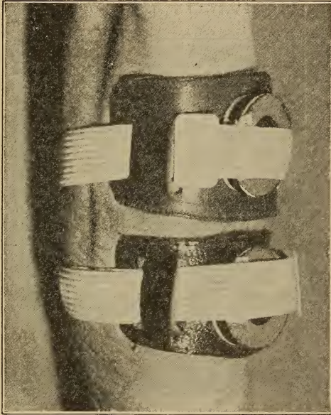
FIG. 61.—Wristlet method used for breeding lice. (Hutchison, Photo by Dovener.)
