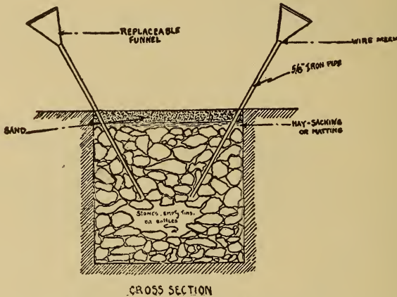
FIG. 7.—Urine soakage pit, in cross section (Mann's modification from Lelean).
