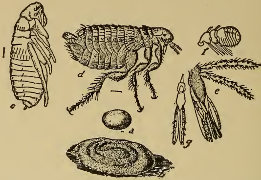
FIG. 65.—The dog flea ( Ctenocephalus canis ): a, Egg; b, larva in cocoon; c, pupa; d, adult; e, mouth parts of same from side; f, antenna; g, labium from below; b, c, d, much enlarged; a, e, f, g, more enlarged. (From Howard.) From U. S. Dept. Agr., Bull. 248, fig. 3.
